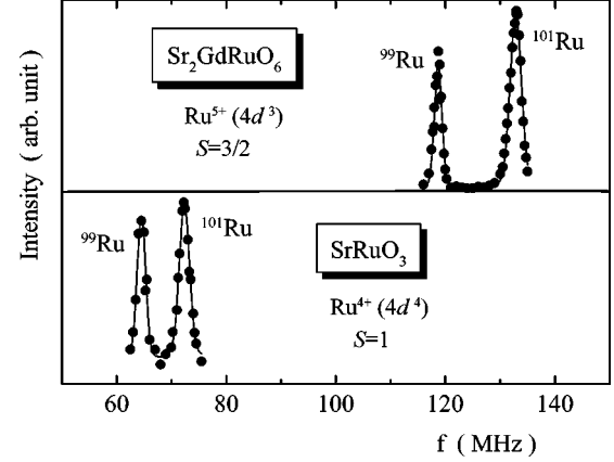
FIG. 5. Ru-ZFNMR spectra of \text{Sr}_2\text{GdRuO}_6 (insulating antiferromagnet with \text{Ru}^{5+} ) and \text{SrRuO}_3 (metallic ferromagnet with \text{Ru}^{4+} ).
