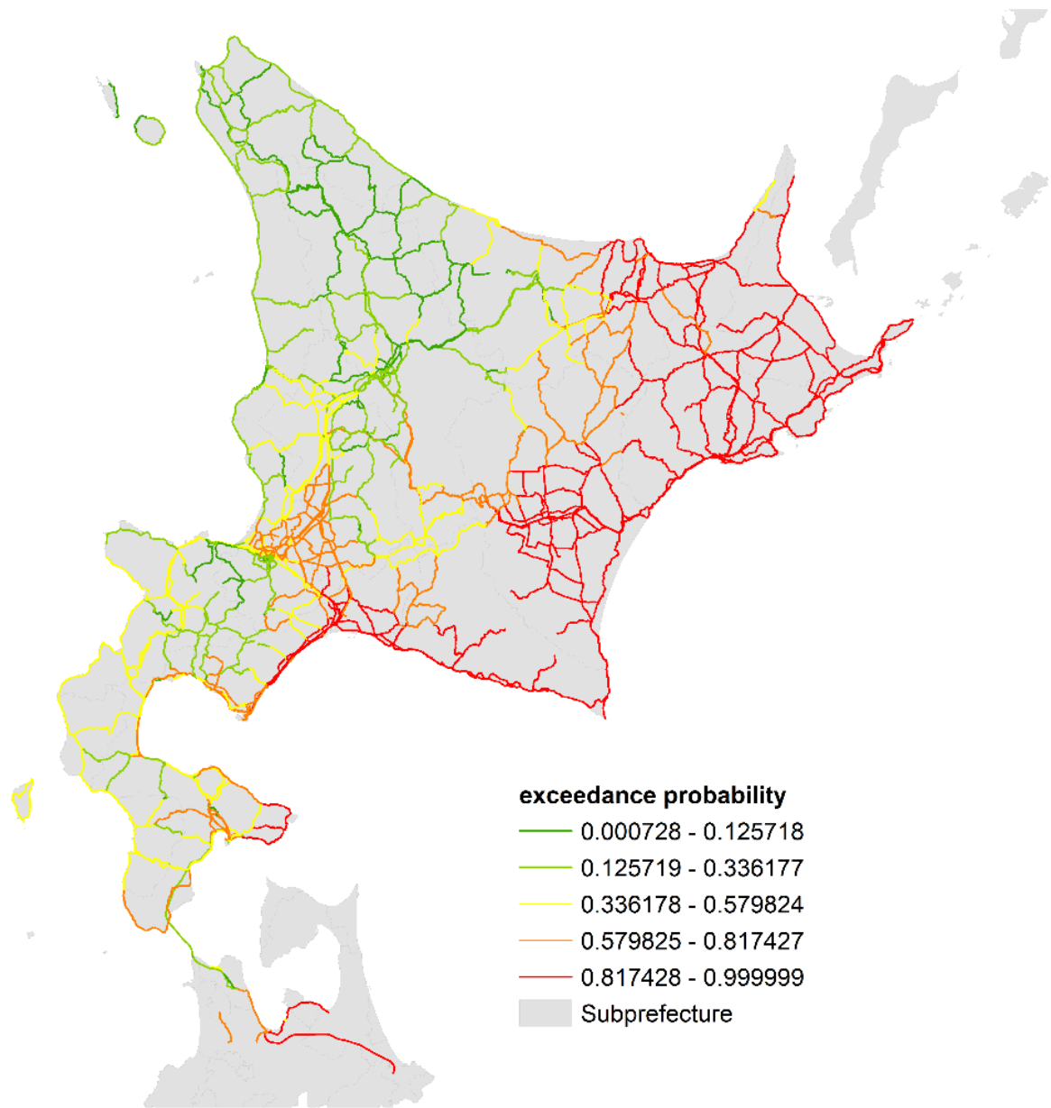
Figure 30 Seismic disaster probability of Hokkaido logistics transportation network (JAM intensity \geq 5)
