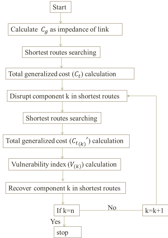
Figure 4 vulnerability scanning algorithm
