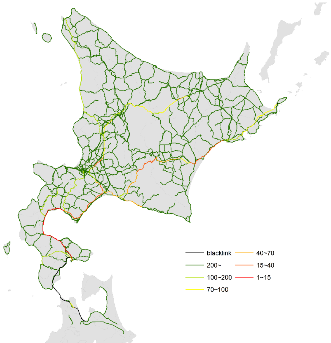
Figure 36 Link categories by seismic vulnerability index (import direction)
