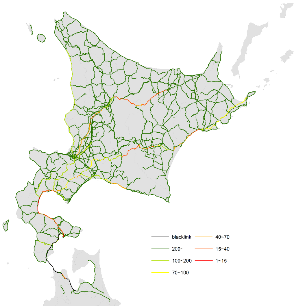
Figure 35 Link categories by seismic vulnerability index (export direction)
