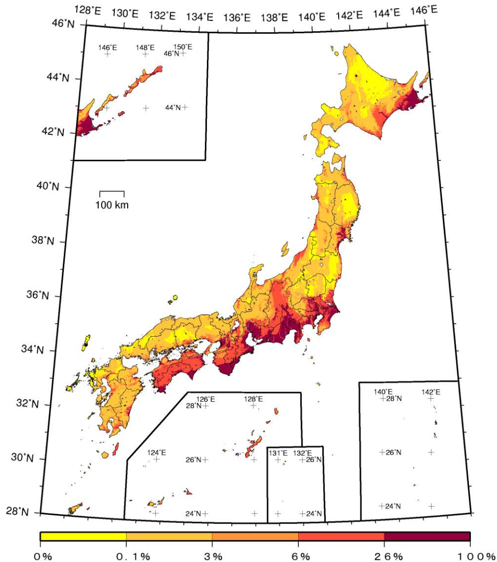
Figure 32 Exceedance probability within 30 years considering all earthquakes (JMA seismic intensity: 6 Lower or more; average case; period starting Jan. 2010)
