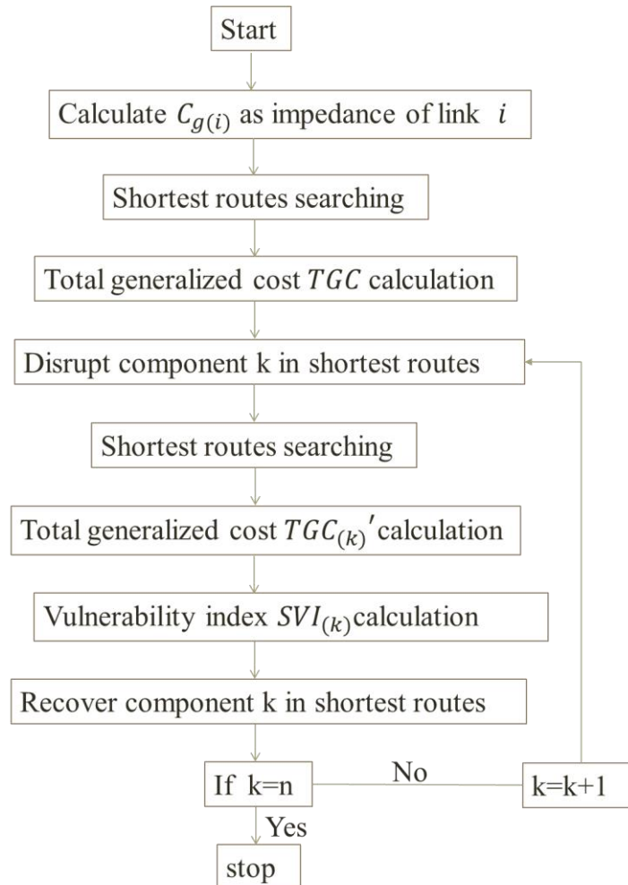
Figure 24 Seismic vulnerability scanning algorithm
