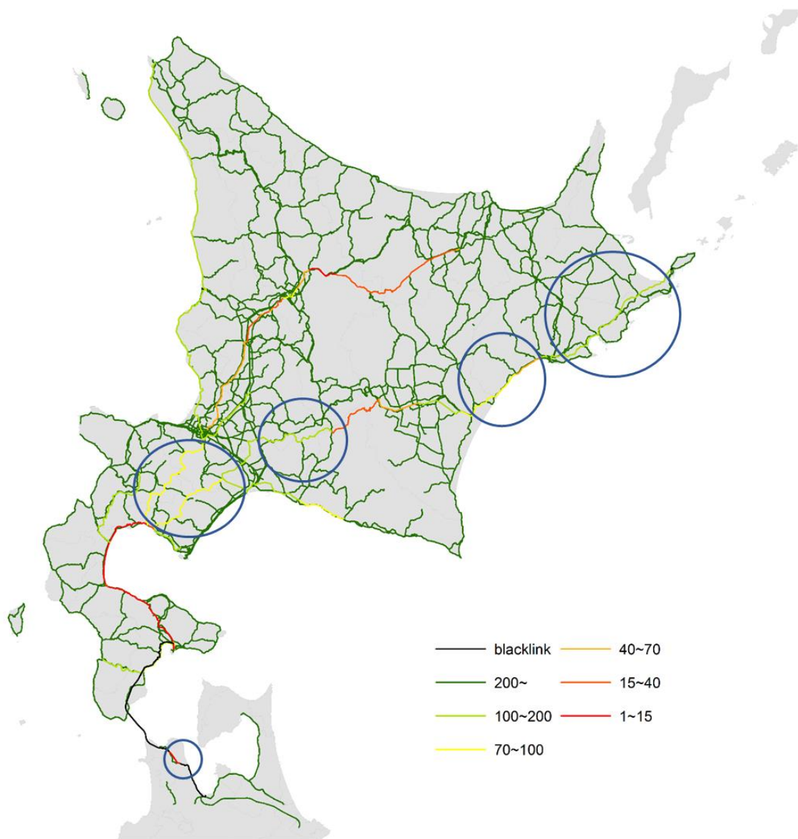
Figure 37 Link categories without considering probability of degradation (export direction)
