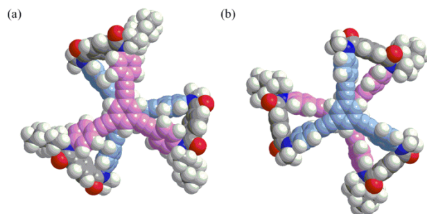
Fig. 2 Energy-minimized structures for a model (R,R,R) - 1a' : (a) Mnnn (rel. 0 kJ mol -1 ) and (b) Pppp (+7.9 kJ mol -1 ), obtained by a conformational search with MacroModel software (v9.9 Monte Carlo Multiple Minimum method, MMFF*, nonsolvated, 50000 steps).
