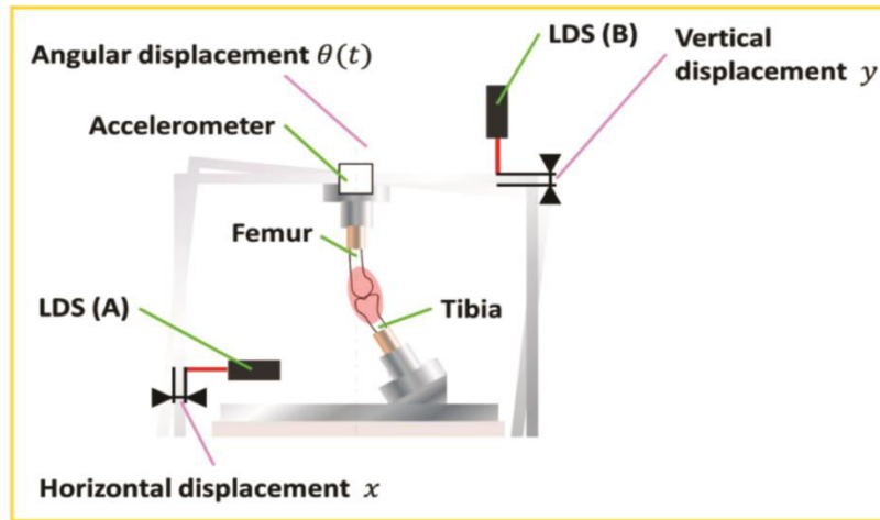
Figure 3. Illustration of the pendulum friction tester used in this study. The friction coefficient \mu was calculated using the equation \mu = L\Delta\theta/4r , where r is the radius of the rabbit femoral condyle, L is the distance between the pendulum's center of gravity and center of rotation, and \Delta\theta is the average decrease in the amplitude of the pendulum swing per cycle
