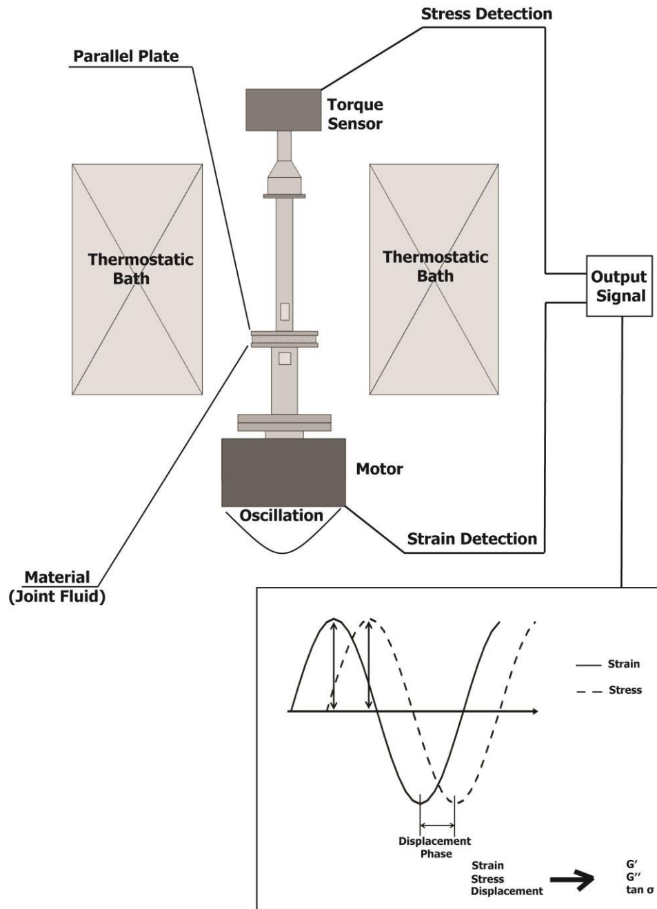
Figure 4. Illustration of the Dynamic Mechanical Analyzer (DMA) used in this study. G' = shear storage modulus (measuring the fluid's elastic character); G'' = shear loss modulus (measuring the fluid's viscous character); \tan \delta = loss rate of energy of a mode of oscillation (measuring the phase displacement).
