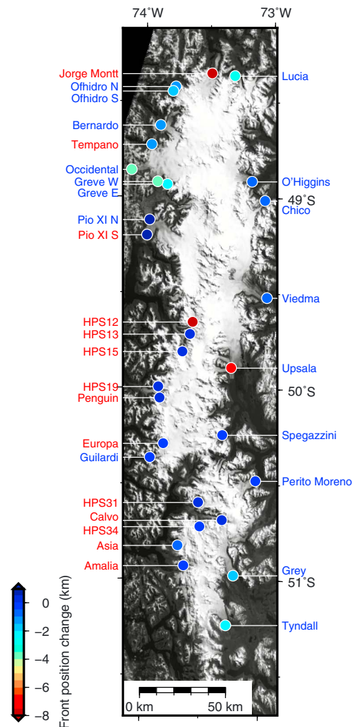
Figure 2. Changes in the glacial front positions from 1984 to 2011 (advance is positive). Tidewater-calving glaciers are written in red, while freshwater calving in blue. Background is a mosaic Landsat 7 ETM+ image acquired in 2001. The white color indicates snow, ice, or cloud-covered regions.
