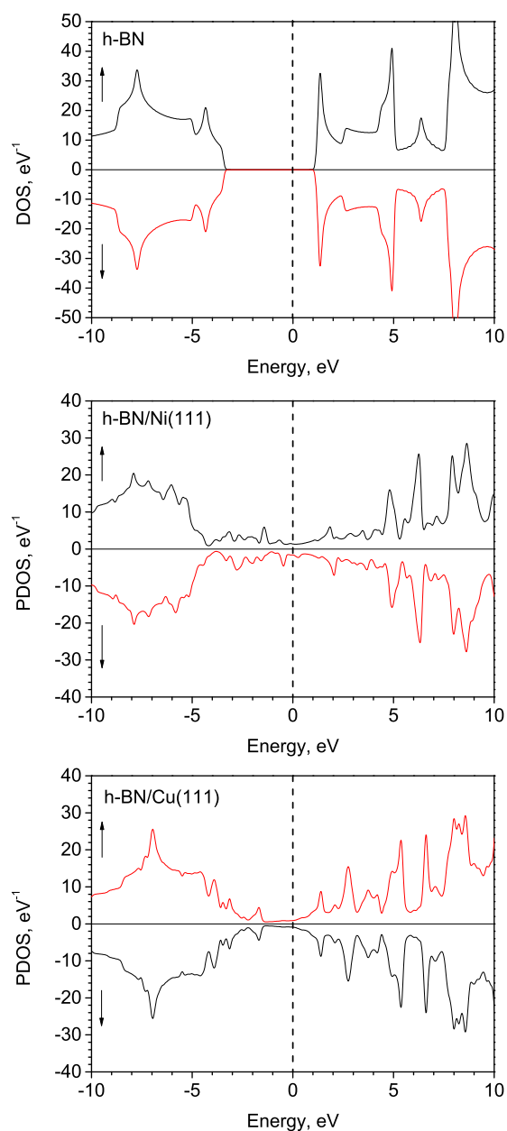
Fig. 2 Spin polarized density of electronic states (DOS) calculated for the defect free h-BN monolayer as well as partial DOS (PDOS) projected on B and N atoms for h-BN/Ni(111) and h-BN/Cu(111) systems. The location of the Fermi level is indicated by a dashed vertical line at 0 eV. Arrows directed up and down indicate the up-spin and down-spin DOS, respectively. A Gaussian broadening of half-width 0.1 eV has been used.
