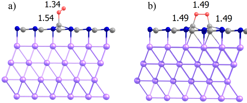
Fig. 4 Optimized structure of the molecular oxygen chemisorbed on the h-BN/Ni(111) surface in (a) on-top (in a doublet spin state) and (b) bridge configuration (in a singlet spin state). The distances are given in Angstroms.
