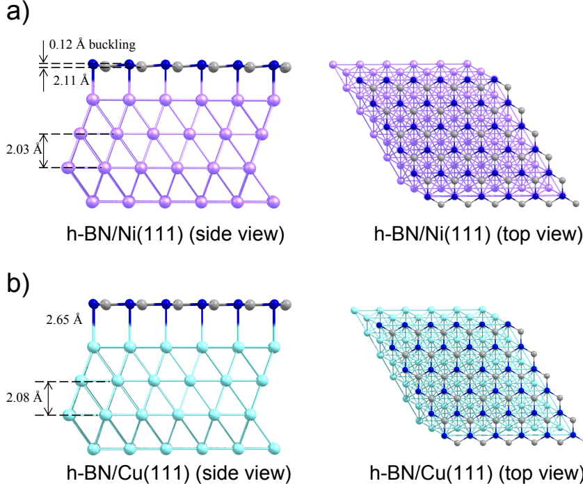
Fig. 1 Surface models: side (left) and top (right) views of the optimized h-BN/Ni(111) (a) and h-BN/Cu(111) (b) structures. All distances are given in Angstroms.
