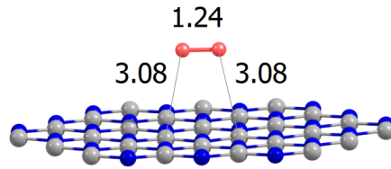
Fig. 3 Optimized structure of the molecular oxygen physisorbed on a free h-BN monolayer. The distances are given in Angstroms.
