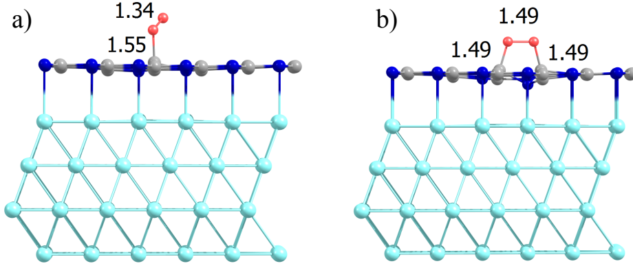
Fig. 5 Optimized structure of the molecular oxygen chemisorbed on the h-BN/Cu(111) surface in (a) on-top (in a doublet spin state) and (b) bridge configuration (in a singlet spin state). The distances are given in Angstroms.
