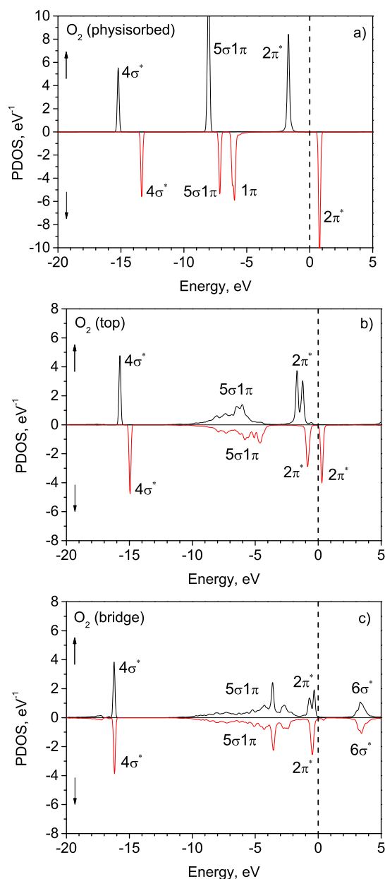
Fig. 6 Partial density of electronic states (PDOS) projected on the O_2 molecule (a) physisorbed on h-BN monolayer, and adsorbed on the h-BN/Ni(111) surface in the (b) top (superoxo-like) and (c) bridge (peroxo-like) configurations. The position of the Fermi level is indicated by a dashed vertical line at 0 eV. Arrows directed up and down indicate the up-spin and down-spin PDOS, respectively. Gaussian broadening of half-width 0.1 eV has been used.
