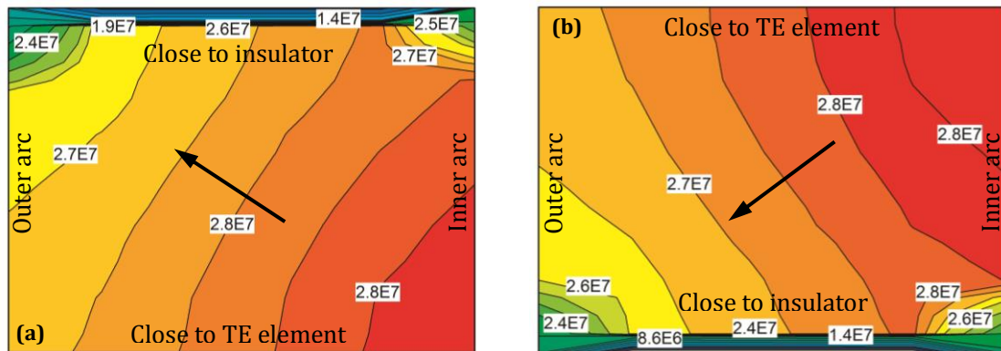
Figure 11 Current density ( \text{A}\cdot\text{m}^{-2} ) inside electrodes of contacting with hot (a) and cold (b) insulators
