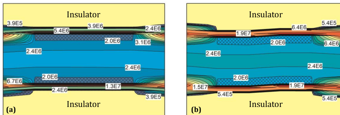
Figure 10 Current density ( \text{A}\cdot\text{m}^{-2} ) inside p-type (a) and n-type (b) elements
