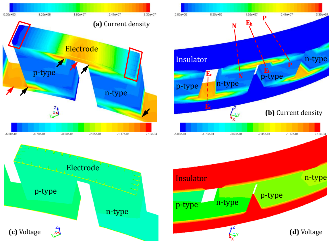
Figure 9 Current density ( \text{A}\cdot\text{m}^{-2} ) and voltage (V) in helical system
