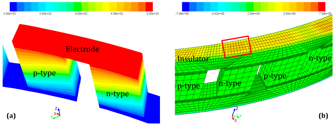
Figure 13 Temperature (K) (a) and heat flux ( \text{W}\cdot\text{m}^{-2} ) (b) in helical system
