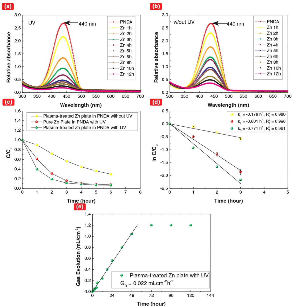
Figure 4. Detection of OH radicals and measurement of gas evolution. (a–b) PND peak intensity decrease at \lambda = 440 \text{ nm} to observe the effect of UV irradiation. (a) Plasma-treated Zn plate (UV). (b) Plasma-treated Zn plate (No UV). (c,d) Decomposition trend for PND by evaluating the concentration change at the \lambda = 440 \text{ nm} peak. (e) Time dependence of the gas evolution on extended UV-irradiated, plasma-treated Zn. The gas volume increase slowed down after \text{UV}_{72\text{h}} , which is consistent with the terminated apical growth of a nanorod in Fig. 1(d).
