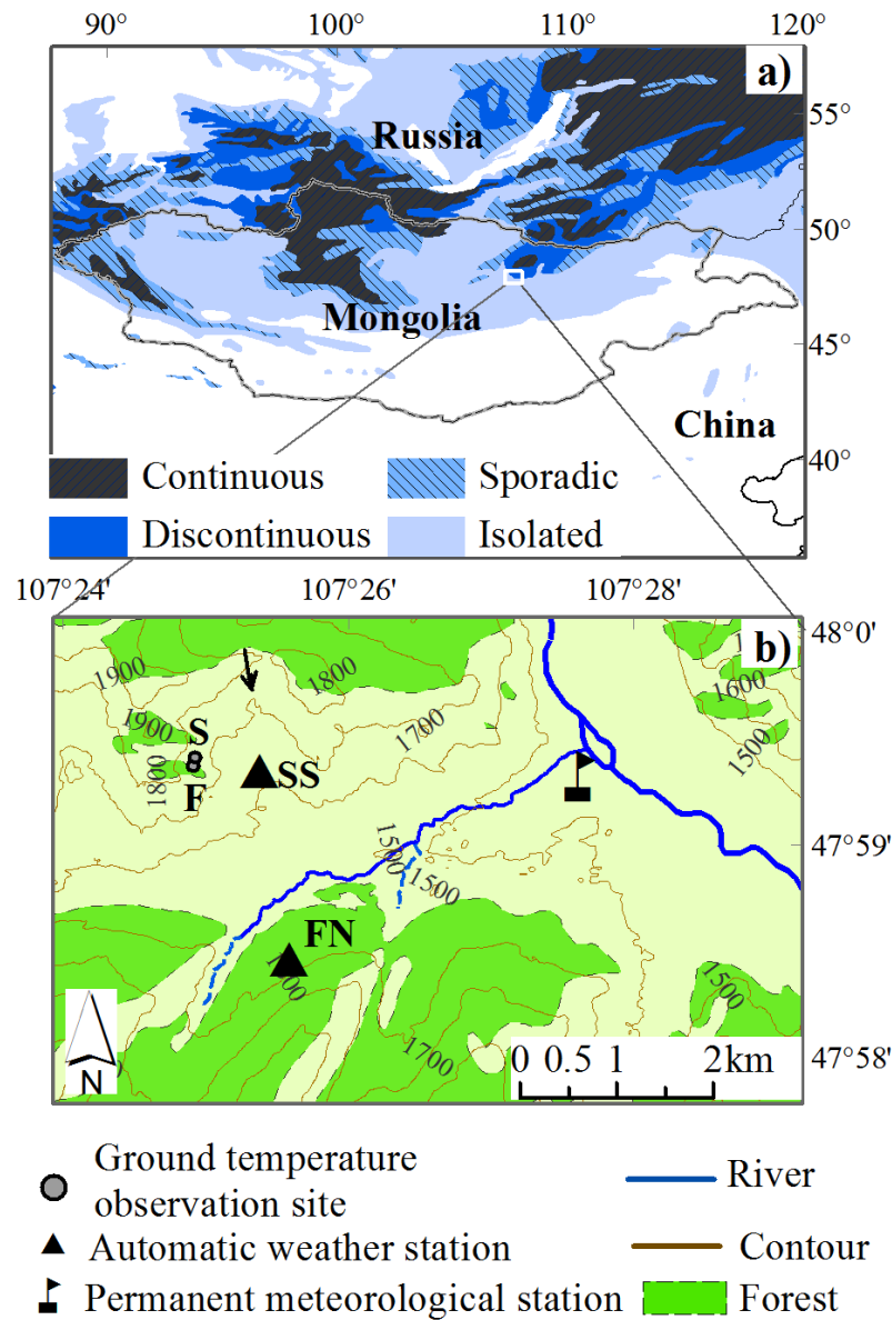
Figure 2.1 Study site locations. (a) Permafrost distribution around Mongolia based on Brown et al. (1997). (b) Field site: FN and SS are automatic meteorological stations; F and S are shallow boreholes with temperature dataloggers. The black arrows show direction of photograph was taken, corresponding to the black arrow in Photo 2.1. The meanings of FN, SS, F and S are the forested north-facing slope, steppe south-facing slope, forest and steppe, respectively.
