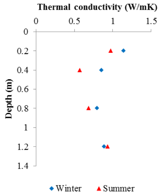
Figure 4.8 Seasonal variations in thermal conductivity for soil layers from 0.2 m to 1.2 m under the forested north-facing slope (FN) for winter and summer in 2006.
