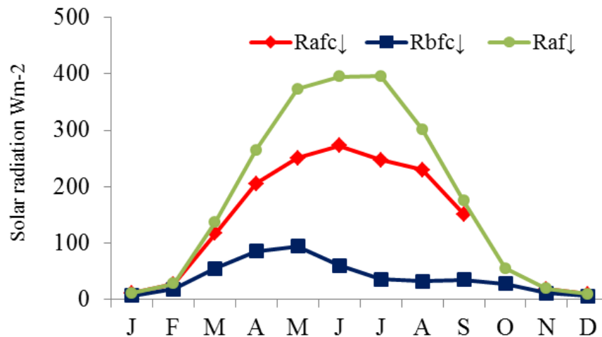
Figure 3.5 The monthly potential ( R_{afc\downarrow} ), calculated ( R_{af\downarrow} ) and observed solar radiation ( R_{bfc\downarrow} ) at FN for 2006.
