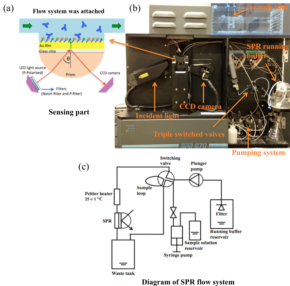
Figure 2.7 SPR 670 from Nippon Laser and Electronics-Japan: (a) sensing part, (b) SPR instrumentation, (c) diagram of SPR flow system.
