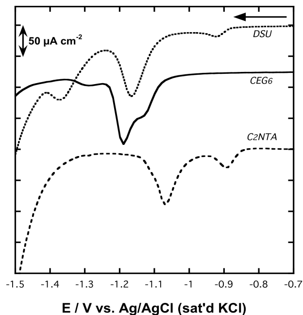
Figure 4.3 Voltammograms of reductive desorption of DSU, CEG 6 and C 2 -NTA monolayer. Electrolyte solution was 0.1 M KOH, while sweep rate was 0.1 V s -1 .
