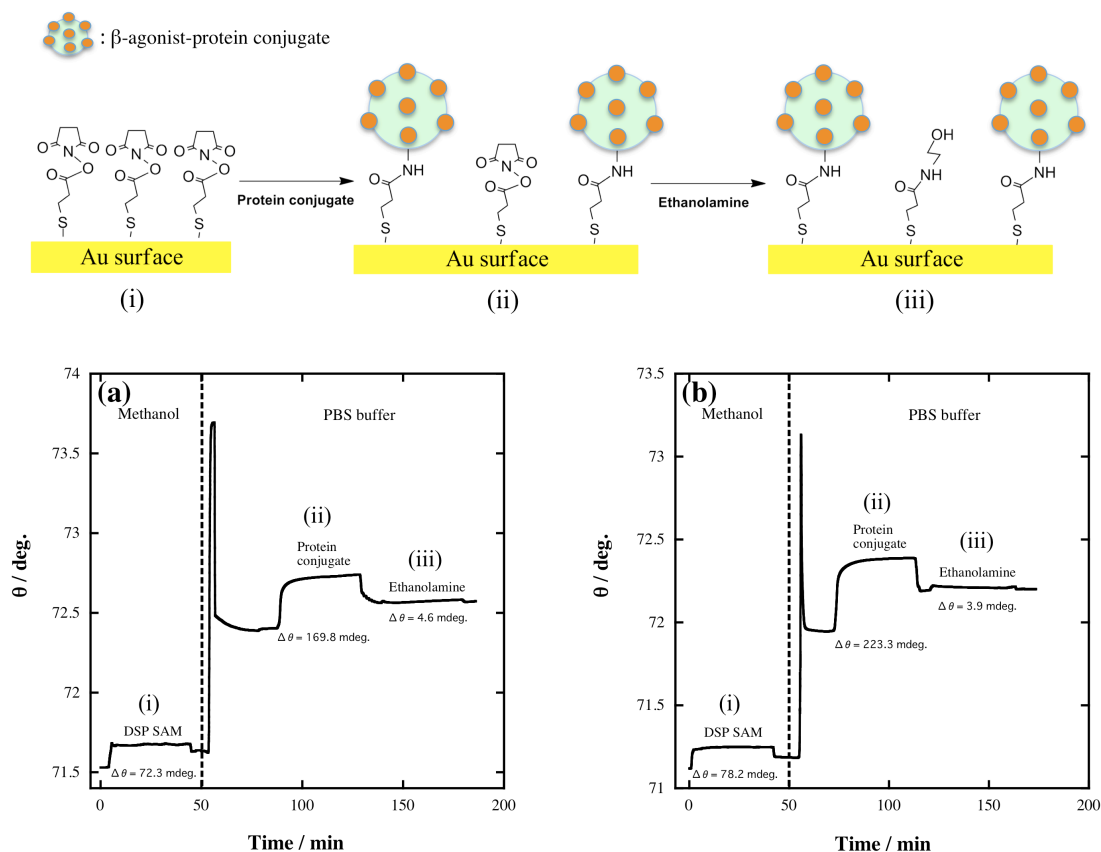
Figure 5.1 SPR sensorgram of the fabrication of the sensor surface at the flow rate of 5 \mu\text{L min}^{-1} : (i) self-assembly of the succinimidyl-terminated propanethiol monolayer, (ii) immobilization of the \beta -agonistprotein conjugates (ractopamine–BSA and salbutamol–HRP), and (iii) blocking of the unreacted succinimidyl-terminated propanethiol with ethanolamine.
