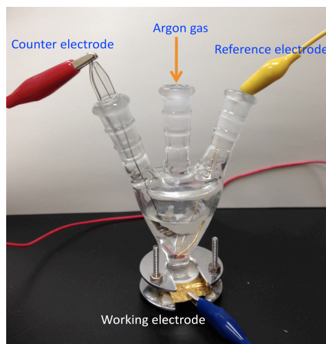
Figure 2.8 Electrochemical cell including Au-chip substrate, platinum wire, and Ag/AgCl (saturated KCl) as working electrode, counter electrode, reference electrode, respectively.
