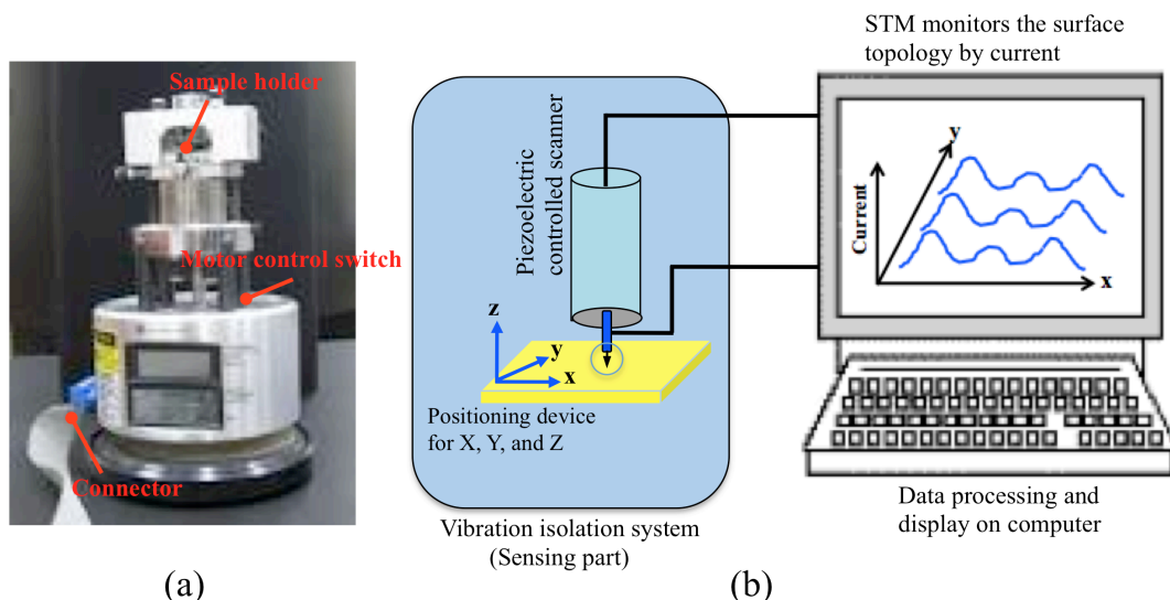
Figure 2.10 Scanning tunneling microscopy: (a) sensing tools, (b) sensing principle.
