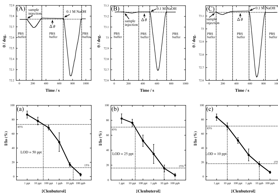
Figure 4.4 SPR sensing format for immunoreaction at (A) DSU, (B) CEG 6 and (C) C 2 -NTA sensor surfaces at the flow rate of 100\mu\text{L min}^{-1} . Clenbuterol detection by using indirect competitive inhibition immunoassay on various sensor surfaces: (a)
