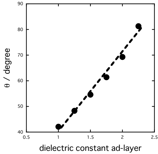
Figure 2.5 Dielectric constant change of ad-layer affected on the resonance angle.
