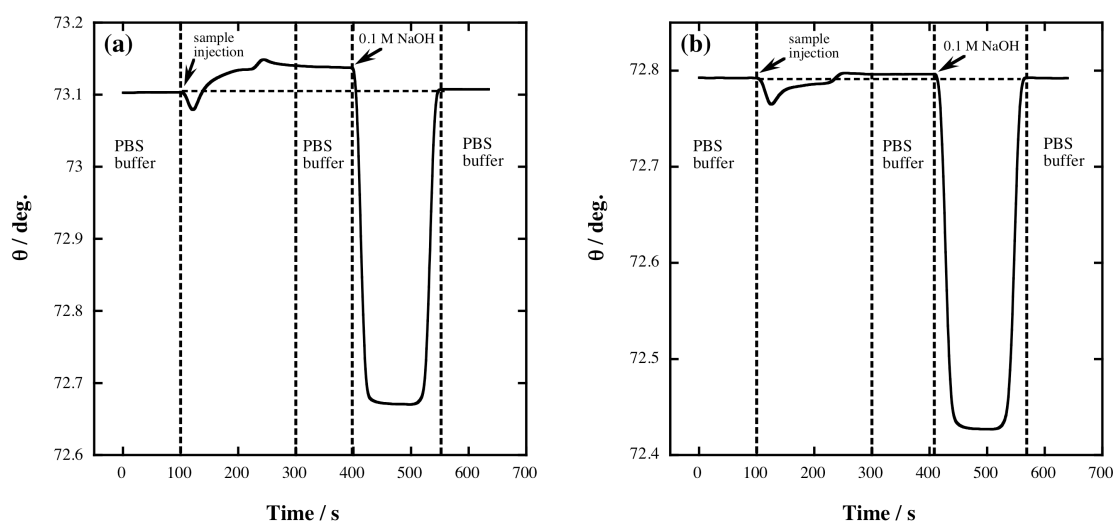
Figure 5.2 SPR sensorgrams of the detection of (a) ractopamine and (b) salbutamol. The flow rate was 100 \mu\text{L}\cdot\text{min}^{-1} , PBS (10% ethanol) solution was used as the running solution, and 0.1 M NaOH aqueous solution was used to regenerate the sensor surface.
