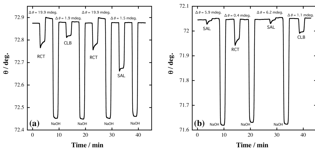
Figure 5.6 Selectivity studies of \beta -agonist sensor surfaces by multiple antibodies injection on: (a) RCT sensor surface and (b) SAL sensor surface. Flow rate was 100\mu\text{L min}^{-1} .
