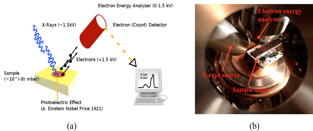
Figure 2.9 X-ray photoelectron spectroscopy: (a) principle of method, (b) view inside of XPS chamber.
