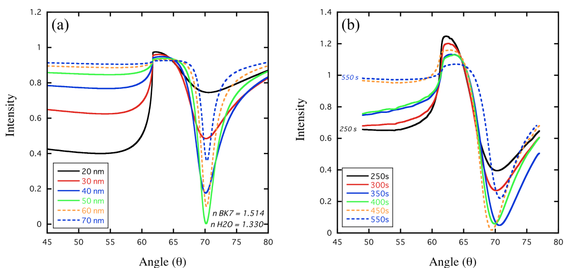
Figure 2.11 SPR angle for various Au thicknesses on glass chip: (a) SPR simulation, (b) Experimental result using sputtering machine of JFC 1600 Auto Fine Coater from JEOL-Japan; note: 1 nm thickness \approx 10 s deposition.
