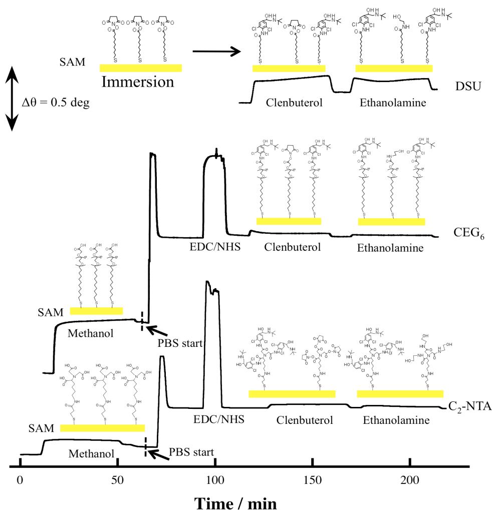
Figure 4.2 SPR sensorgram for fabrication of the sensor surface by using functionalized various thiols monolayer (DSU, C 2 -NTA and CEG 6 ) on Au surface. Flow rate was 5 \mu\text{L min}^{-1} .
