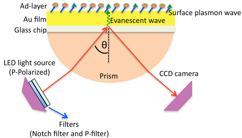
Figure 2.4 Principle of SPR sensing
