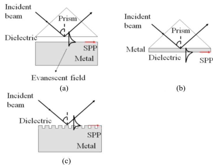
Figure 2.1 Surface plasmon resonance configurations [10]: (a) Otto configuration, (b) Kretschmann configuration, and (c) Diffraction grating.
