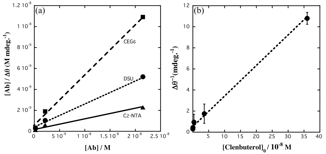
Figure 4.5 (a) Langmuir adsorption isotherm plot for binding of anti-clenbuterol antibody (Ab) to clenbuterol immobilized on the sensor surface, and (b) clenbuterol solution concentration dependence using indirect competitive inhibition immunoassay.
