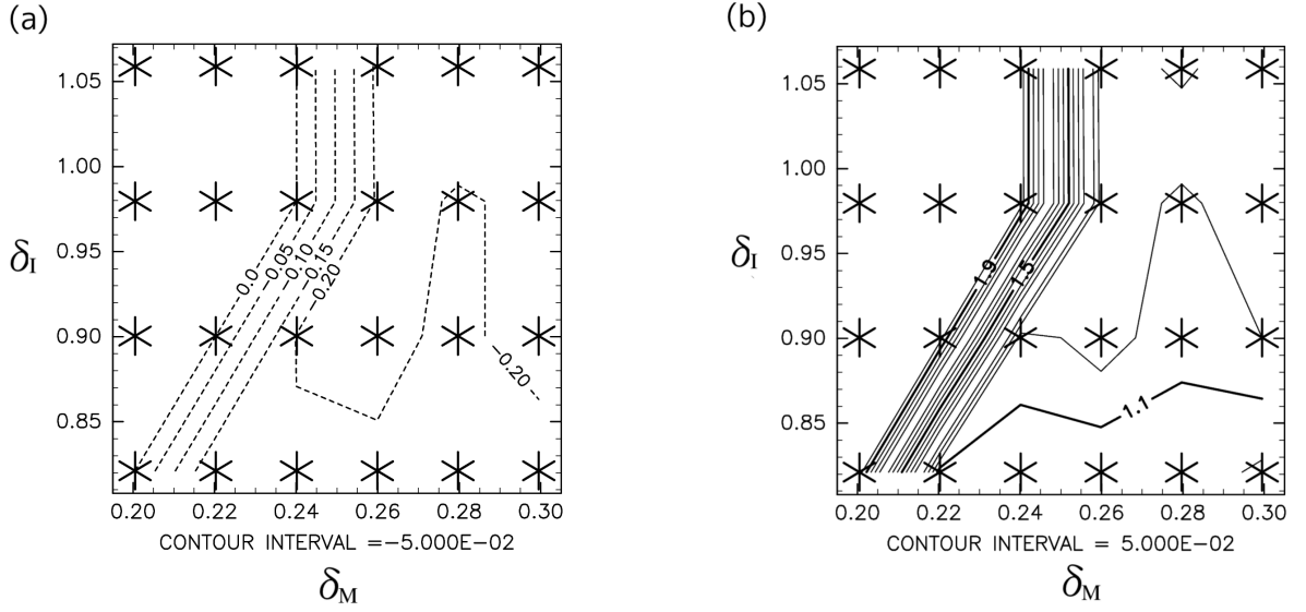
Figure 12: (a) Dependence of the y coordinate of the eastward extension jet, Y_{Jet} , on \delta_M and \delta_I . (b) Dependence of the jet length on \delta_M and \delta_I . The asterisks denote data points for which computations were made. Y_{Jet} changes discontinuously from 0 (gyre boundary jet case) to -0.2 (prematurely separated jet case) between two adjacent computational points and there is no intermediate value of Y_{Jet} . All experiments were run from rest. The final state depends on the initial condition; in many cases an initial condition in the gyre or prematurely separated jet case will persist even under parameter values in which the other state is found when spun up from rest (see text for details).
