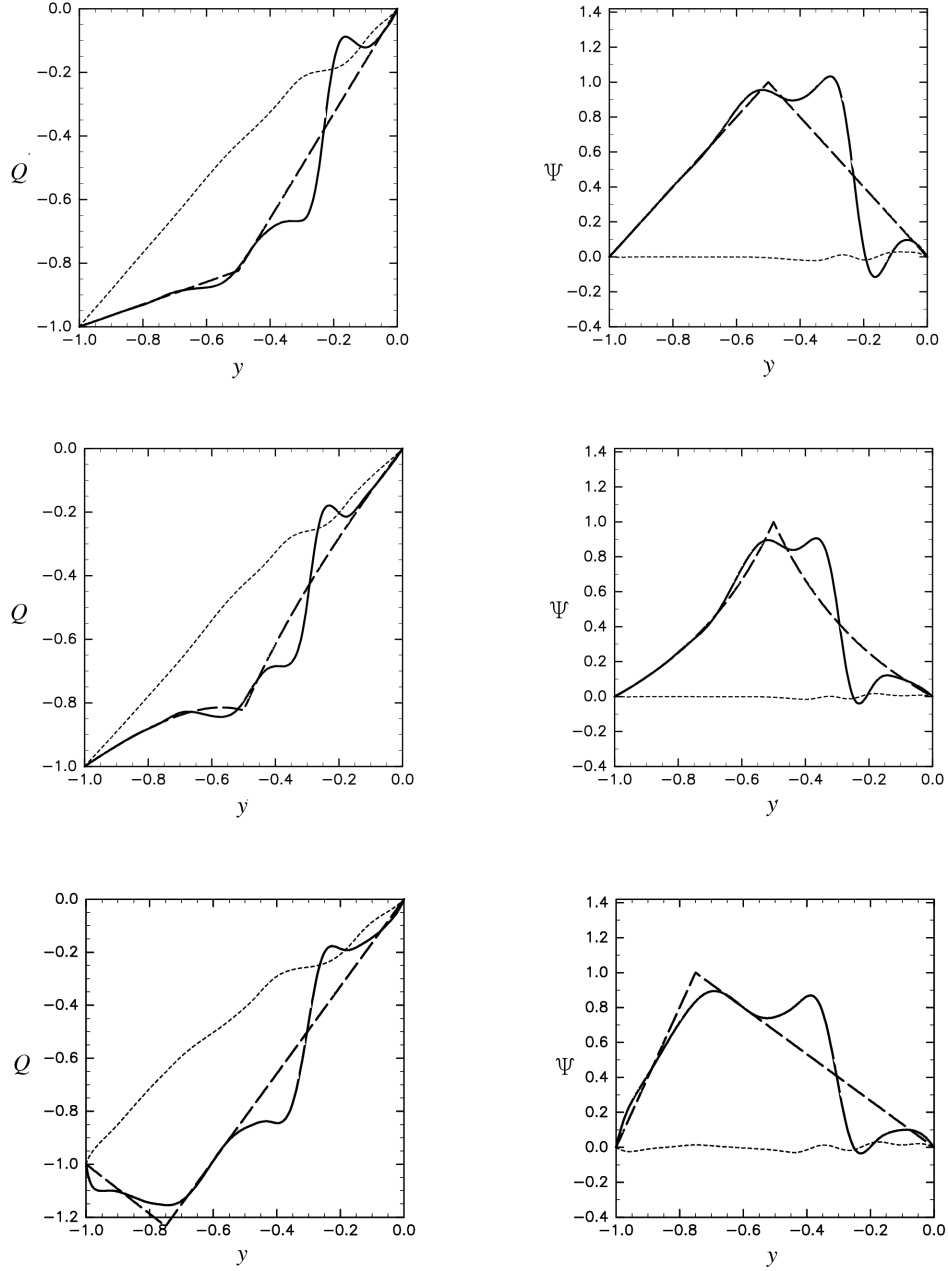
Figure 19: Meridional distribution of the temporal mean potential vorticity and streamfunction; definitions are the same as in Fig. 7. (Upper): L_1 ; (middle): X_1 ; (lower): L_2 . (Left): potential vorticity; (right): streamfunction in the upper layer (solid line) and the lower layer (dotted line) averaged in the zonal direction from x = 0.5 to x = 1.0 . The dashed lines are \hat{q}_{Sv} and \hat{\psi}_{Sv} , which were estimated from the Sverdrup balance for the upper layer.
