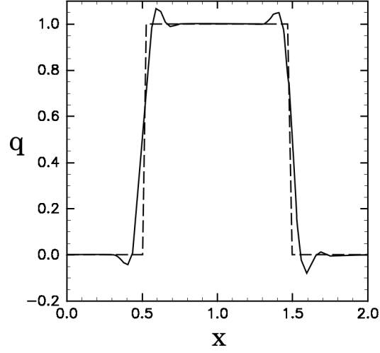
Figure 2: Numerical solution of advection equation of rectangular wave. The solid line indicates using IDO-CF scheme; the dashed line indicates initial.
