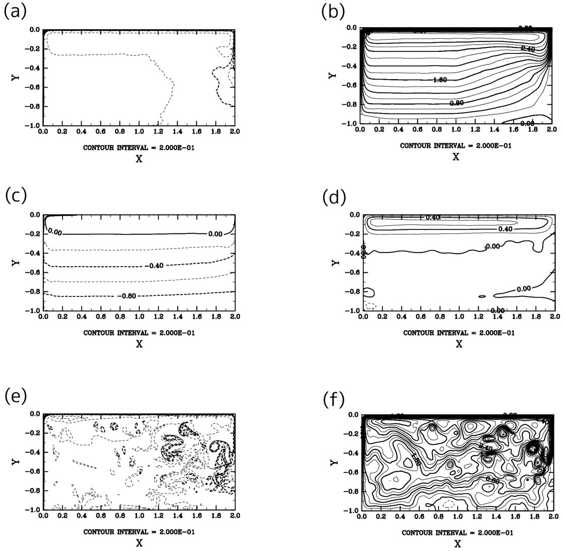
Figure 10: Same as Fig. 8 but for the gyre boundary jet case ( \delta_m = 0.22, \delta_I = 0.9 ).
