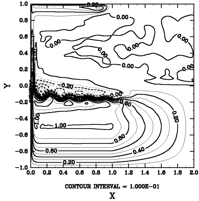
Figure 17: Same as Fig. 16 but for Y_N = 1 and slip western boundary condition was used.
