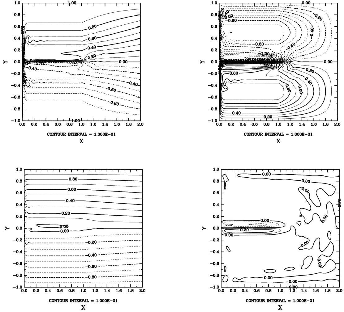
Figure 5: Same as Fig. 4 but for the gyre boundary jet case ( \delta_M = 0.22, \delta_I = 0.9 )
