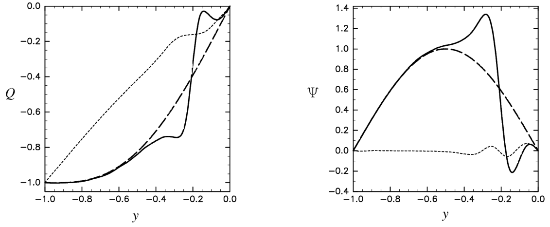
Figure 9: Meridional profiles of mean potential vorticity (left) using single-gyre forcing and streamfunction (right) for the prematurely separated jet case ( \delta_M = 0.30, \delta_I = 0.9 ). Averaged from x = 0.5 to x = 1.0 in the western half region of the basin. The solid line in the upper layer, the dotted line in the lower layer and the dashed line indicate the values estimated by the Sverdrup balance in the upper layer.
