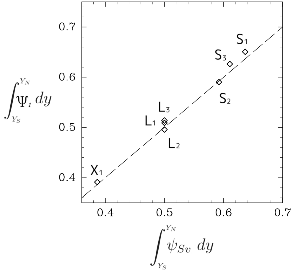
Figure 22: A plot of meridionally integrated value of time mean streamfunction against that of the Sverdrup streamfunction at arbitrary longitude in the west-half region. The dashed line shows \int \psi_{Sv} dy = \int \Psi_1 dy .
