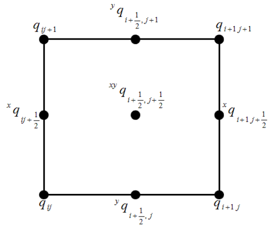
Figure 3: Configuration of variables on grids for the IDO-CF scheme.
