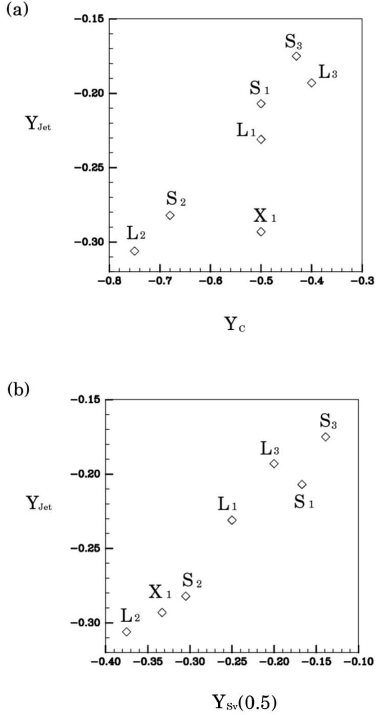
Figure 20: (a) The y -coordinate of the extension jet, Y_{Jet} , as a function of the y -coordinate of the center of the Sverdrup circulation, Y_C . (b) Y_{Jet} as a function of the y -coordinate at which \hat{\psi}_{Sv} = 0.5 , Y_{sv}(0.5) . The letter symbols in the figure correspond to Table 3. The letter symbols in the figure correspond to Table 3.
