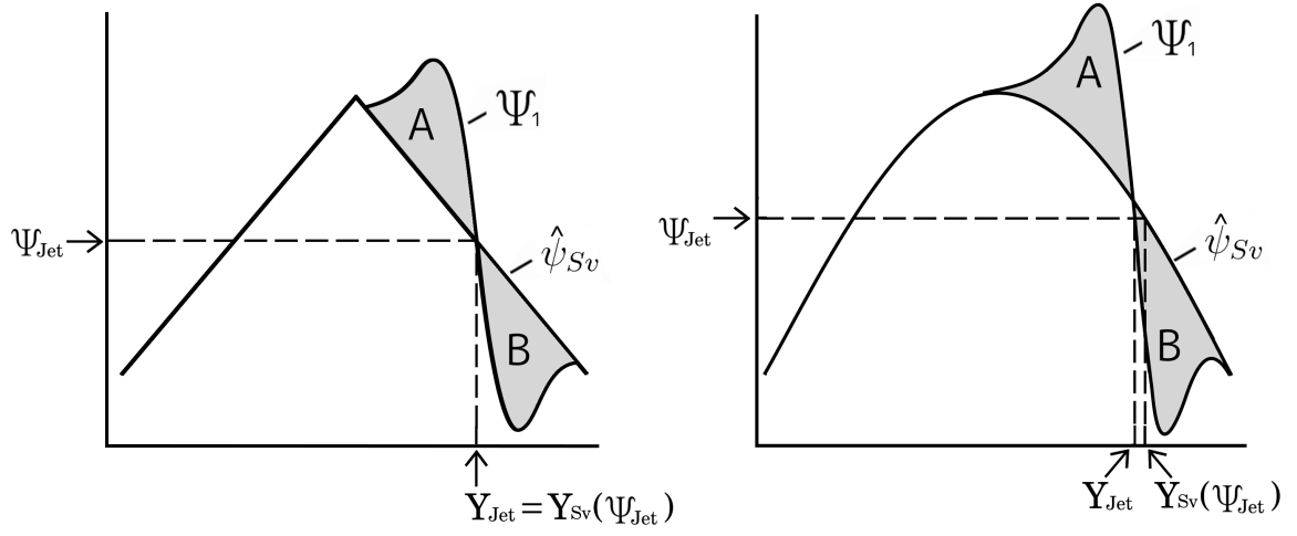
Figure 23: Schematic illustration of the change in meridional direction of Y_{Jet} arising from the change in \hat{\psi}_{Sv} distribution. The area of the shadow denoted by A is equal to that by B when equation (3.5) is maintained. Because \Psi_{Jet} takes the middle value of the local maximum value and local minimum value of \Psi_1 , Y_{Sv}(\Psi_{Jet}) should correspond to Y_{Jet} in the case of \frac{\partial^2 \hat{\psi}_{Sv}}{\partial y^2} = 0 , (left panel) and Y_{Sv}(\Psi_{Jet}) should be to the north from Y_{Jet} in the case of \frac{\partial^2 \hat{\psi}_{Sv}}{\partial y^2} < 0 (right panel).
