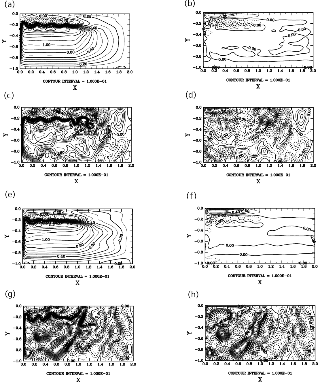
Figure 15: Streamfunction field for each coefficient of bottom friction, \hat{r} . (a) and (b): temporal mean for \hat{r} = 10^{-4} ; (c) and (d): snapshot for \hat{r} = 10^{-4} ; (e) and (f): temporal mean for \hat{r} = 0 ; (g) and (h): snapshot for \hat{r} = 0 . The left side shows the upper layer, and the right side shows the lower layer.
