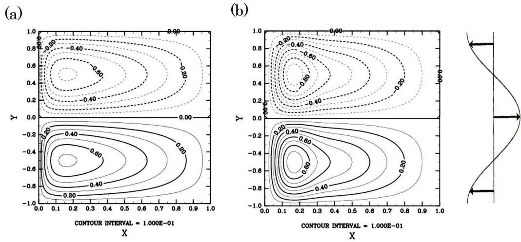
Figure 1: Linear solutions. (a) The streamfunction of Stommel model; (b) That of Munk model with Ekman pumping velocity to \sin \pi y . The domain length is 2.
