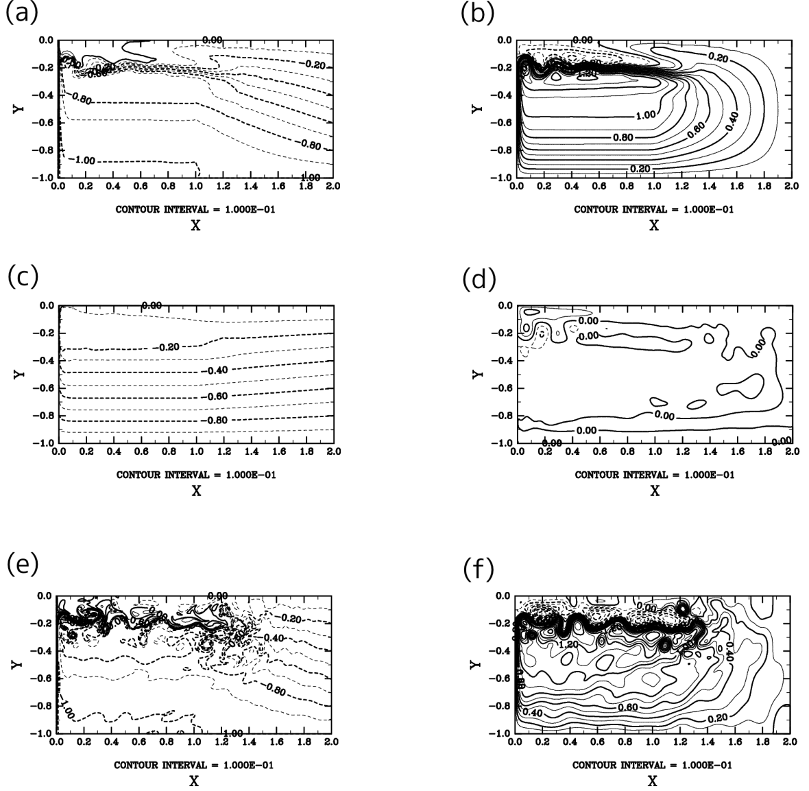
Figure 8: Typical solution of the prematurely separated jet case ( \delta_M = 0.3, \delta_I = 0.9, H_1/H_2 = 1/4 ) under single-gyre forcing. (a) and (b): temporal mean fields of the upper layer potential vorticity divided by \hat{\beta} and streamfunction, respectively. (c) and (d): same as (a) and (b) but for the lower layer. (e) and (f): same as (a) and (b) but for snapshots ( t=100,000 ) in the upper layer.
