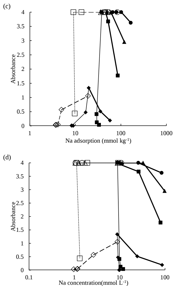
Figure 1 Relationship between (a) phosphate sorption, (b) phosphate concentration, (c) Na adsorption, (d) Na concentration, and absorbance of the soil suspension. \diamond pH 4, \square pH 5.5, \triangle pH 7, \circ pH 8.5 for initial \text{NaNO}_3 concentration of 1 \text{mmol L}^{-1} at step 1 in the phosphate sorption experiment. \blacklozenge pH 4, \blacksquare pH 5.5, \blacktriangle pH 7, \bullet pH 8.5 for initial \text{NaNO}_3 concentration of 10 \text{mmol L}^{-1} at step 1 in the phosphate sorption experiment.. ----- electrolyte concentration = 1 \text{mmol}_c \text{ L}^{-1} , - - - - - 1 \text{mmol}_c \text{ L}^{-1} < \text{electrolyte concentration} < 10 \text{ mmol}_c \text{ L}^{-1} , ————— electrolyte concentration = 10 \text{mmol}_c \text{ L}^{-1} , ————— electrolyte concentration > 10 \text{mmol}_c \text{ L}^{-1} ,
