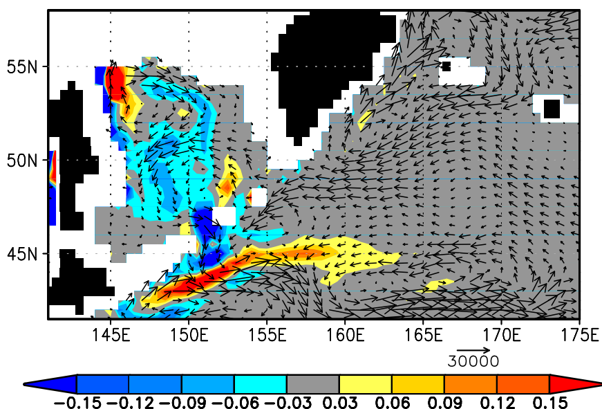
FIG. 16. As in Fig. 13, but for region B, calculated from the WSTR experiment.
