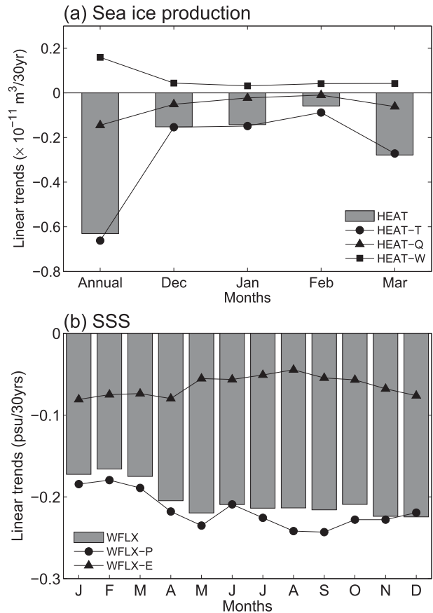
FIG. 14. (a) Linear trends [ \times 10^{11} \text{ m}^3 (30 \text{ yr})^{-1} ] in the annual and monthly sea ice production in the HEAT (gray bars), HEAT-T (circles), HEAT-Q (triangles), and HEAT-W (squares) experiments. Sea ice production is integrated over the northwestern shelf region ( 54^{\circ} – 60^{\circ}\text{N} , 137^{\circ} – 150^{\circ}\text{E} ). (b) Linear trends [ \text{psu} (30 \text{ yr})^{-1} ] in monthly sea surface salinity over the northwestern shelf region in the: WFLX (gray bars); WFLX-P (circles); and WFLX-E (triangles) experiments.
