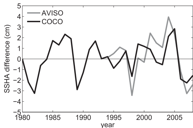
FIG. 9. Time series of the annual mean of EKC index, which is the difference in SSHA between the east Kamchatka coast ( 53^\circ\text{N} , 160^\circ\text{E} ) and the offshore area ( 50^\circ\text{--}55^\circ\text{N} , 165^\circ\text{--}170^\circ\text{E} ) from the altimeter data (gray) and simulated data (black). The positive anomaly means that the EKC is enhanced relative to the climatological value.
