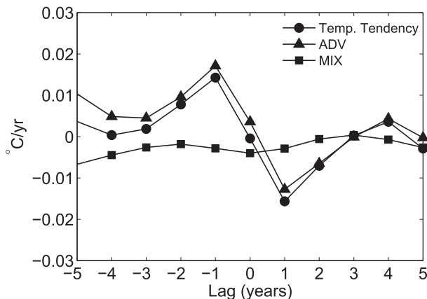
FIG. 15. As in Fig. 12, but for the subarctic frontal region in the WSTR experiment.
