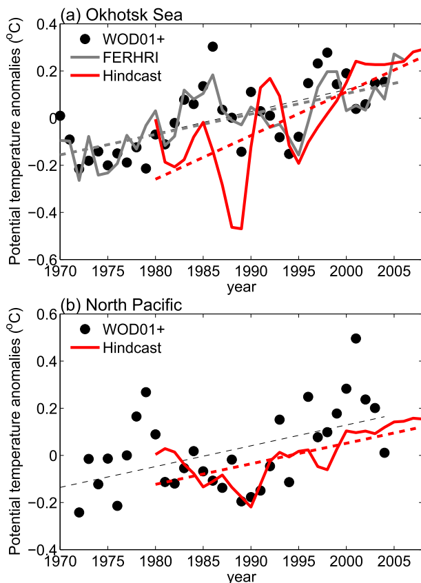
FIG. 6. Time series of the annual mean of potential temperature anomalies averaged over (a) the southern part of the Okhotsk Sea (region A) and (b) the western subarctic North Pacific (region B), at 27.0\sigma_\theta for the WOD01+ (black circles), FERHRI (gray line), and hindcast data (red line). Linear regressions of the annual time series are indicated by dashed lines.
