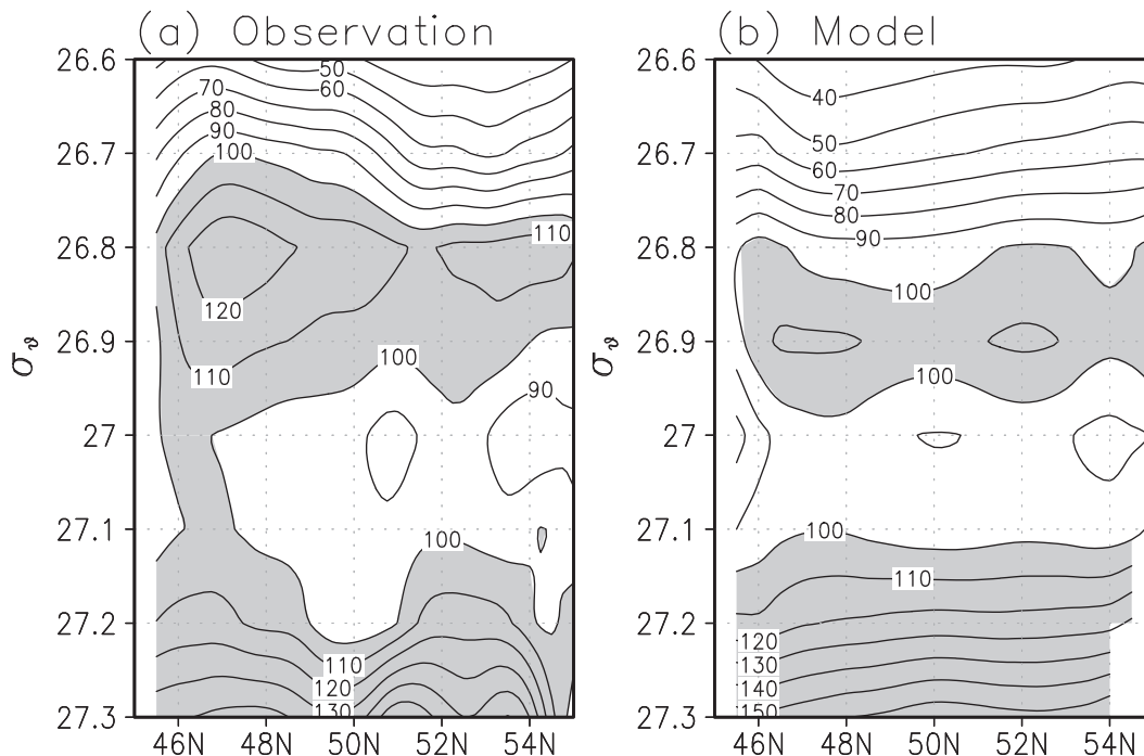
FIG. 3. The latitudinal cross section of the climatological layer thickness (m) along 148°E derived from the (a) observation and (b) model. The vertical axis is potential density. The shading indicates the regions where the thickness is >100 m.
