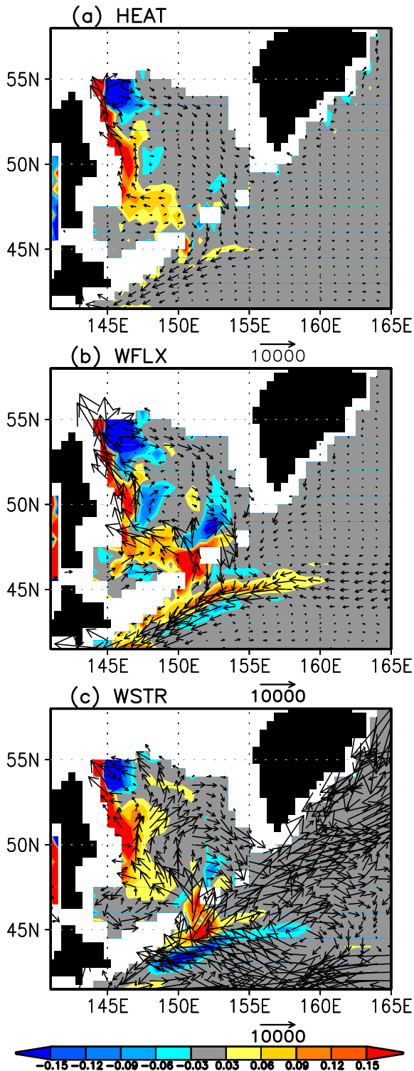
FIG. 13. Lag -1 yr regression maps of annually averaged heat fluxes (vectors, ^{\circ}\text{C m}^{-3} \text{ yr}^{-1} ) and their convergence (color shades with positive values, ^{\circ}\text{C yr}^{-1} ) by large-scale flow (ADV) onto the potential temperature at 27.0\sigma_{\theta} averaged over the western part of the Okhotsk Sea (region A), calculated from the (a) HEAT, (b) WFLX, and (c) WSTR experiments. The vertical component of the heat flux is not shown. In (c), the signs of the regression coefficients are inverted. The white regions represent areas with water lighter than 26.9\sigma_{\theta} .
