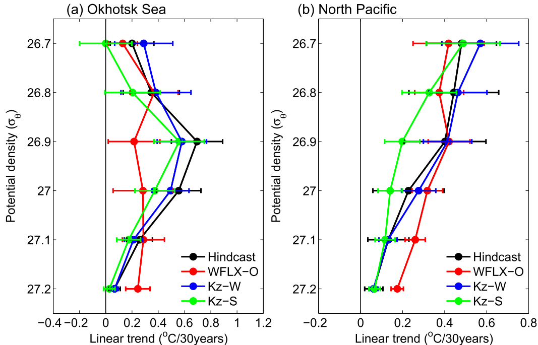
FIG. 8. As in Fig. 6, but for the annually averaged potential temperature on isopycnal surfaces from the hindcast data (black), the WFLX-O (red), K_z -W (blue), and K_z -S (green).
