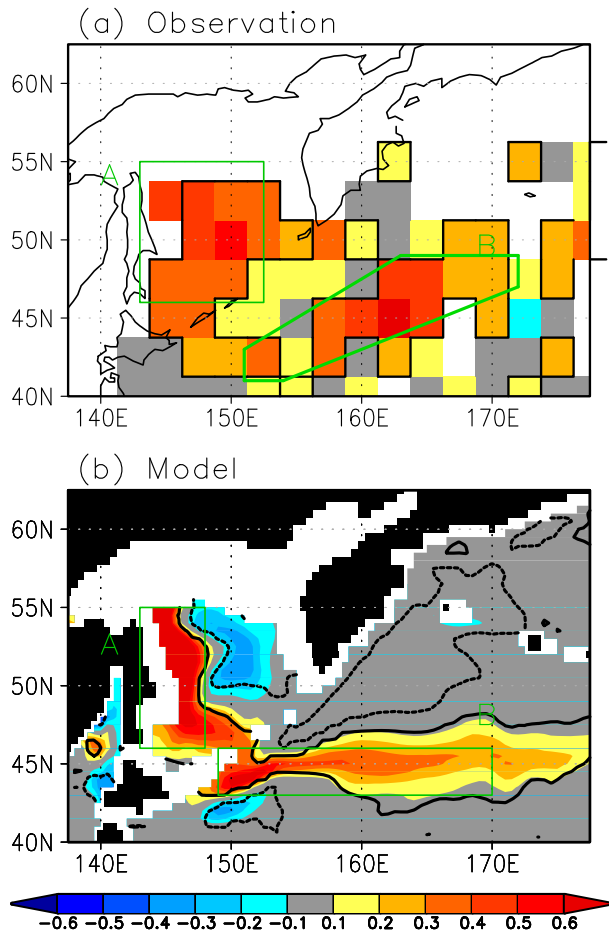
FIG. 4. Linear trend maps [ ^{\circ}\text{C} (30 \text{ yr})^{-1} ] in the annually averaged potential temperature at 27.0\sigma_{\theta} in (a) observed data from 1970 to 2004 and (b) the hindcast experiment from 1980 to 2008. The white-colored regions in (b) represent water that is lighter than the corresponding density. The contour indicates the regions where the linear trend is significant at 90% confidence level. The significance of the linear trend estimate is based on a Student's t distribution.
