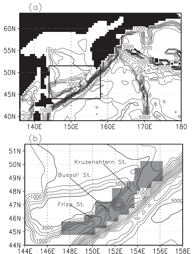
FIG. 1. (a) Model topography. Contour interval is 500 m for depths >1000 m. (b) Model topography around the Kuril Straits [rectangular region in (a)]. Shading indicates region where the tidal mixing parameterization is applied.
