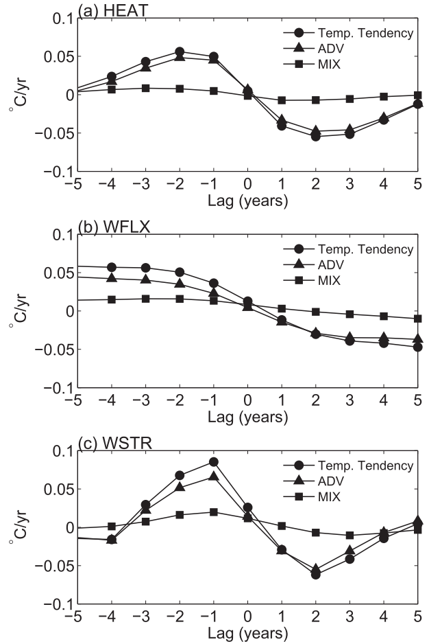
FIG. 12. Lagged regression of annually averaged tendency for the potential temperature (circles) and the convergence of the heat fluxes by large-scale flow (ADV, triangles) and mixing processes (MIX, squares) onto the time series of the potential temperature at 27.0\sigma_\theta averaged over the western part of the Okhotsk Sea (region A) in the (a) HEAT, (b) WFLX, and (c) WSTR experiments. The negative values of lag time mean that the tendency leads the potential temperature.
