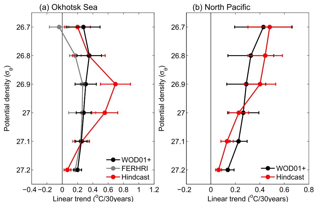
FIG. 5. Linear trends of the annually averaged potential temperature on isopycnal surfaces from the WOD01+ (black), FERHRI (gray), and hindcast data (red), averaged over (a) the western part of the Okhotsk Sea (region A) and (b) the western subarctic North Pacific (region B). The error bars indicate the 90% confidence interval for the linear trend estimate.
