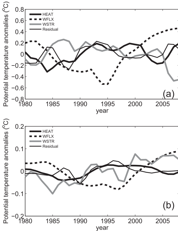
FIG. 11. Time series of the annual mean of potential temperature anomalies at 27.0\sigma_\theta over (a) the western part of the Okhotsk Sea (region A) and (b) the subarctic frontal region (region B), derived from perturbation experiments (HEAT, WFLX, and WSTR) and the residual component (the hindcast experiment minus the sum of the perturbation experiments).
