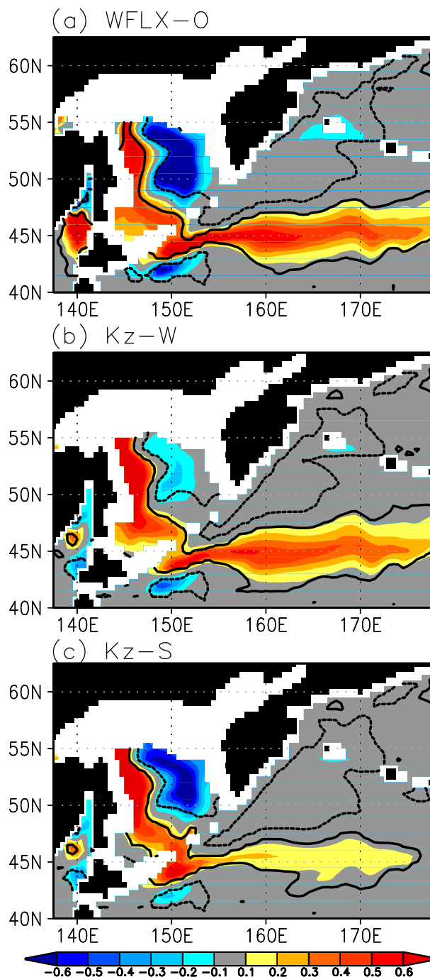
FIG. 7. As in Fig. 4b, but for the sensitivity experiments of (a) WFLX-O, (b) K_z -W, and (c) K_z -S.
