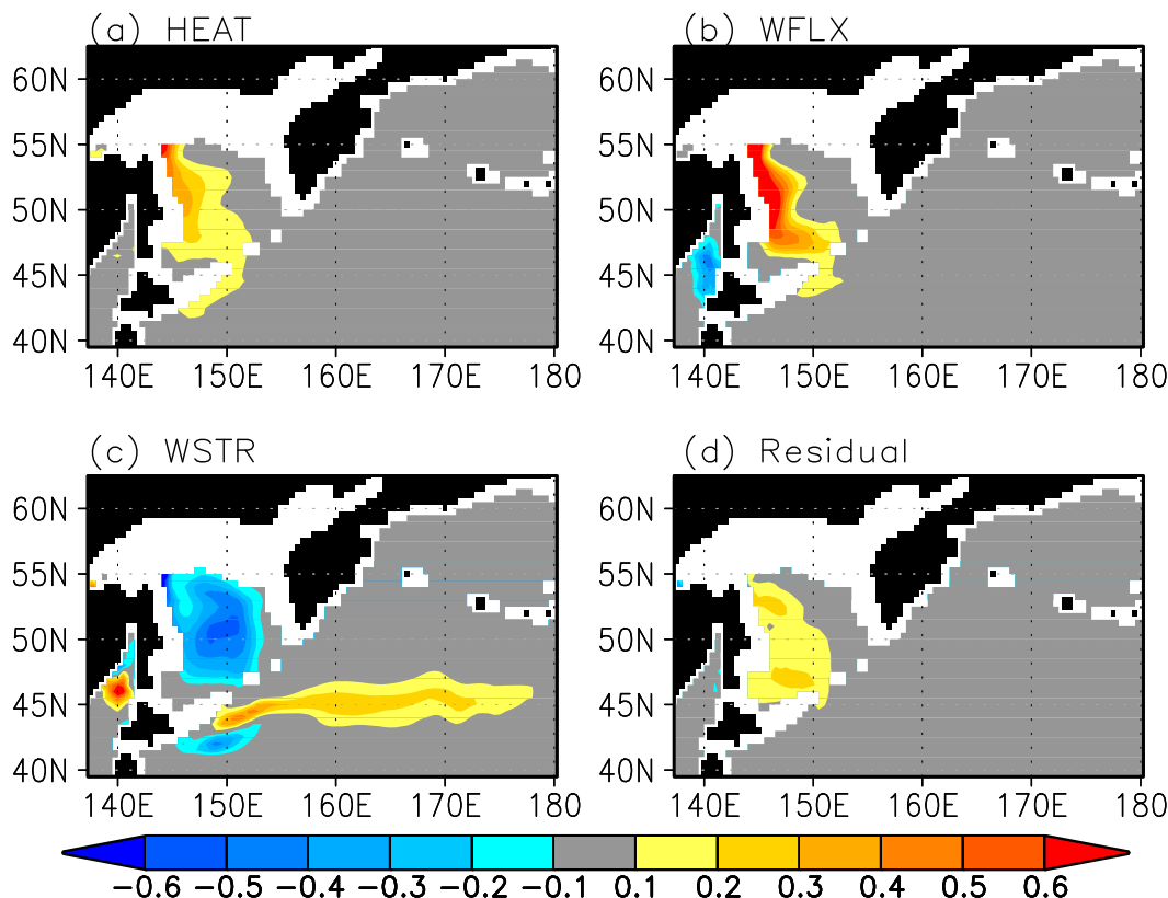
FIG. 10. Linear trends [ ^{\circ}\text{C} (30 \text{ yr})^{-1} , colors] in annually averaged potential temperature at 27.0\sigma_{\theta} , calculated from the (a) HEAT, (b) WFLX, (c) WSTR experiments, and (d) the residual component (the hindcast minus the sum of the HEAT, WSTR, and WFLX experiments). The white regions represent areas where water is lighter than 27.0\sigma_{\theta} .
