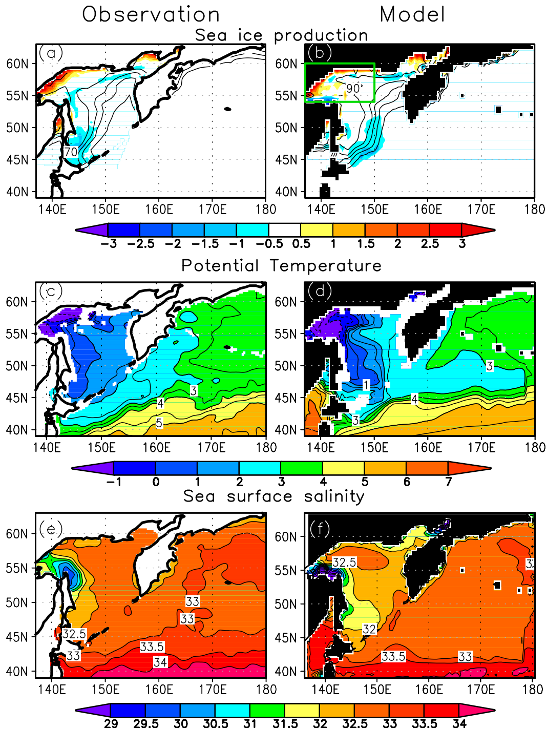
FIG. 2. (a) Observed and (b) simulated (hindcast) climatologies of the annual freshwater flux ( \text{m yr}^{-1} ) associated with sea ice production (positive) and melting (negative). Climatological sea ice concentrations in February are superimposed. Contour interval is 10%, 30%, 50%, 70% and 90%. (c) Observed and (d) simulated (hindcast) climatologies of annually averaged potential temperature ( ^{\circ}\text{C} ) at 26.8\sigma_{\theta} . (e), (f) As in (c), (d), but for sea surface salinity (psu).
