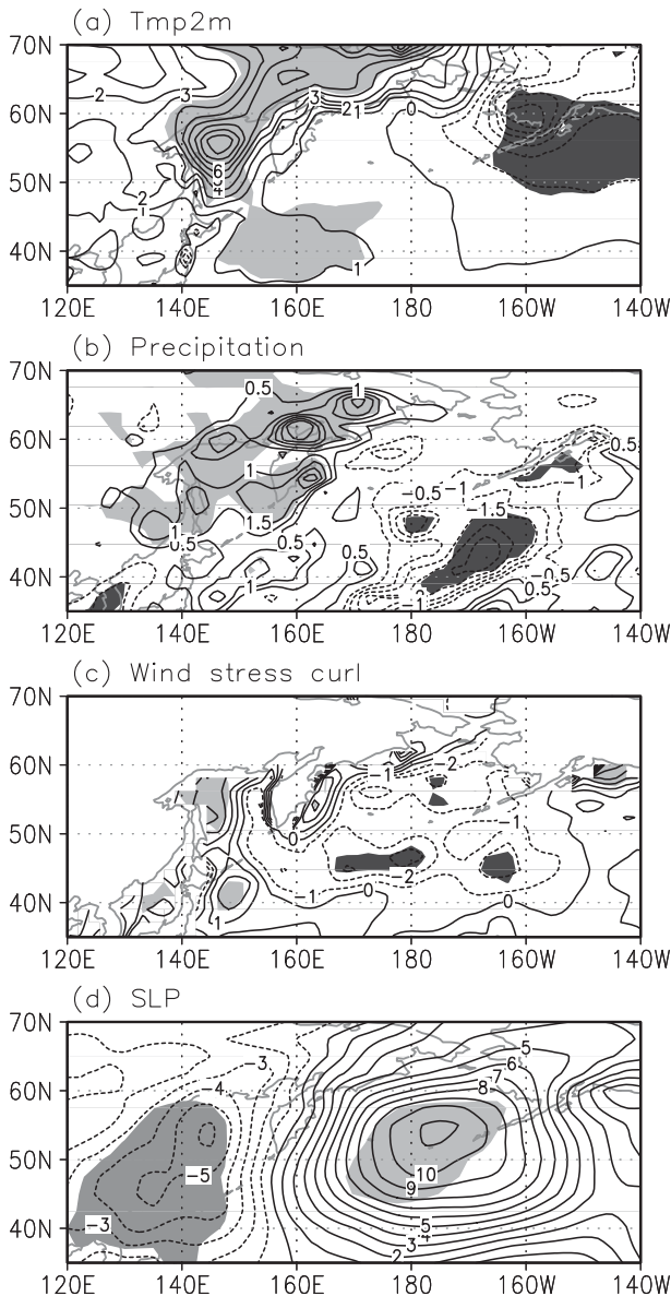
FIG. 19. Linear trends in: (a) surface air temperature [ ^{\circ}\text{C} (30 yr) ^{-1} ], (b) precipitation [mm (30 yr) ^{-1} ], (c) wind stress curl [ \times 10^{-7} \text{ N m}^{-3} (30 yr) ^{-1} ], and (d) sea level pressure [hPa (30 yr) ^{-1} ] in March, as calculated from NCEP–NCAR reanalysis data during the period 1980 to 2008. Shading indicates regions where trends are significant at the 95% confidence level, based on the t test.
