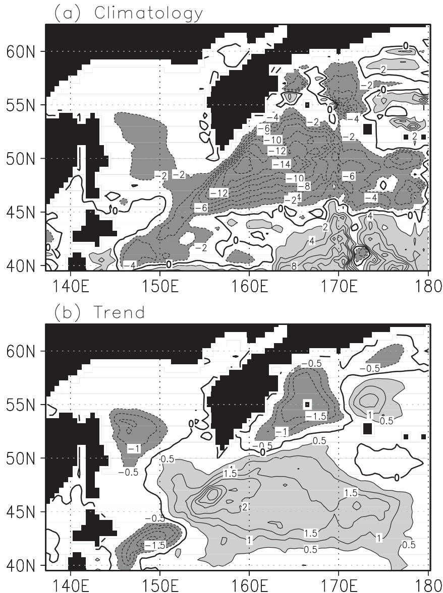
FIG. 17. (a) Climatology (Sv), and (b) linear trend [ \text{Sv (30 yr)}^{-1} ] of annually averaged \Psi in the WSTR experiment. The contour interval is 2 Sv and 0.5 Sv ( 30 \text{ yr}^{-1} ) in (a) and (b), respectively. Negative values indicate cyclonic circulation. The light (dense) shading indicates positive (negative) values larger (less) than 2 Sv and 0.5 Sv ( 30 \text{ yr}^{-1} ) in (a) and (b), respectively.
