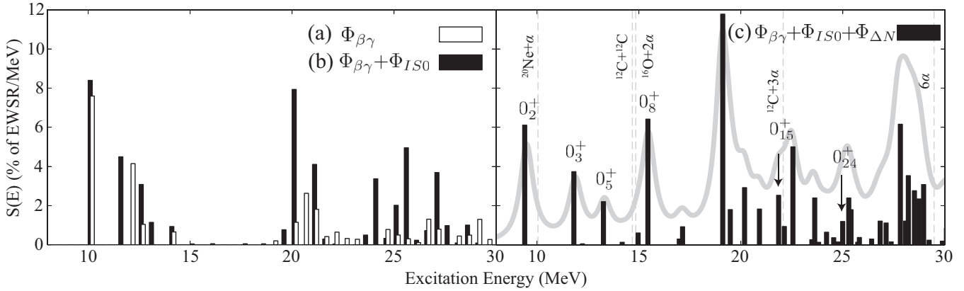
FIG. 2. The isoscalar monopole transition strength functions calculated with the basis sets (a) \Phi_{\beta\gamma} , (b) \Phi_{\beta\gamma} + \Phi_{IS0} , and (c) \Phi_{\beta\gamma} + \Phi_{IS0} + \Phi_{\Delta N} . The solid line in the right panel shows the strength function smeared by a Lorentzian with 0.8 MeV width. The vertical dashed lines indicate cluster decay threshold energies which are located at the observed binding energies.
