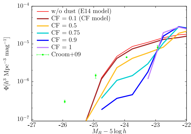
Figure 3. Quasar luminosity functions of the CF model. The red solid line shows the quasar luminosity function without dust attenuation. Other five thick lines show that of with CF = 0.1 (brown solid line), 0.5 (orange solid line), 0.75 (cyan solid line), 0.9 (blue solid line) and 1 (purple solid line); the smaller CF corresponds to the brighter bright end.
