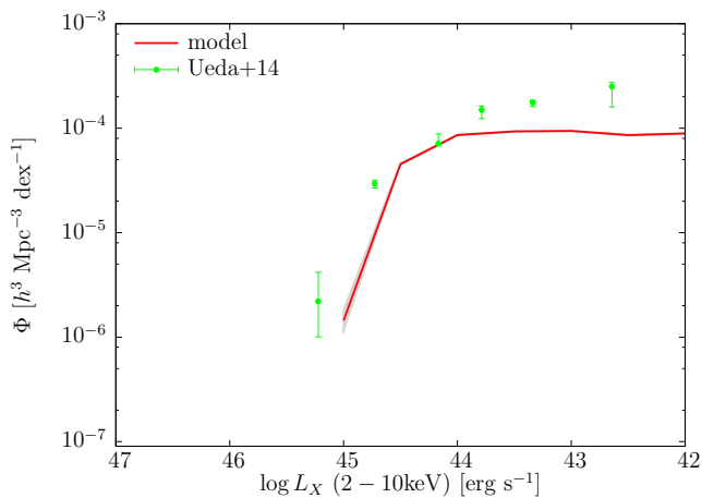
Figure 1. AGN luminosity functions in hard X-ray. We set \epsilon_{\text{bol}} and f_{\text{life}} so that the model reproduces the observed luminosity function obtained by Ueda et al. (2014, green points). Note that the model includes only AGNs that are triggered by major mergers. Hence, it is not surprising that it misses the less powerful Seyfert population. Red line shows the model result. The shaded region indicates 1\sigma error.
