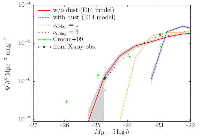
Figure 2. Quasar luminosity functions in the B -band at z \sim 2 . The luminosity function of E14 model is indicated by the red solid line in which we ignore the dust attenuation. We also show the result by the same parameter set as E14 model but with the dust attenuation (blue dotted line). The shaded regions indicate 1\sigma error. The observational estimation is indicated by the green filled circles (Croom et al. 2009). The dark-green filled squares indicate the luminosity function that is converted from the hard X-ray luminosity function obtained by Ueda et al. (2014) using Marconi relations. These points are corresponding to the first and second brightest points in Fig. 1. We also show the results of delay model with \nu_{\text{delay}} = 1 (orange dot dashed line) and with \nu_{\text{delay}} = 3 (black dashed line).
