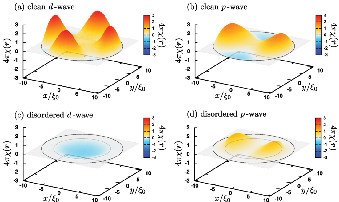
FIG. 2. (Color) Local susceptibilities of small superconducting disks. The results for a d -wave and those for a p -wave superconductor with a clean surface (i.e., w = 0 , \xi_0/\ell = 0 ) are presented in (a) and (b), respectively. The results for a d -wave and those for a p -wave superconductor with a rough surface ( w = 3\xi_0 , \xi_0/\ell = 1.0 ) are demonstrated in (c) and (d), respectively. The parameters used in the simulation are R = 10\xi_0 , \lambda_L = 5\xi_0 , \omega_c = 10\Delta_0 , H^{\text{ext}} = 0.01 H_{c1} , and T = 0.1 T_c .
