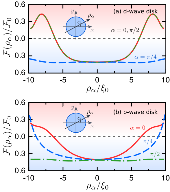
FIG. 8. (Color online) Free-energy densities on a trajectory \rho_\alpha of a d -wave disk (a) and a p -wave disk (b), where \mathcal{F}(\mathbf{r}) is normalized to \mathcal{F}_0 = N_0 \Delta_0^2/2 . The angle \alpha is measured from the x axis as shown in schematics in the figures. The temperature is set to T = 0.1T_c so that the superconducting disks show the paramagnetic response. The second energy cutoff is set to \omega_{c_2} = 400\Delta_0 . The other parameters are fixed as R = 10\xi_0 , \lambda_L = 5\xi_0 , \omega_c = 10\Delta_0 , and H^{\text{ext}} = 0.01H_{c1} .
