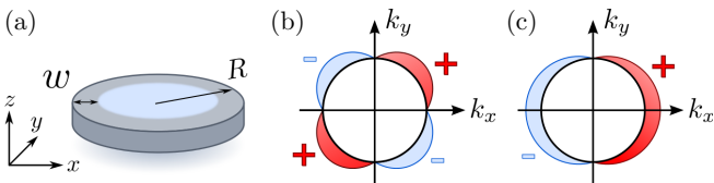
FIG. 1. (Color online) (a) Schematic figure of a superconducting disk with a rough surface, with R and w the radius of the disk and the width of the disordered region, respectively. An external magnetic field is applied in the z direction. The origin of a spatial coordinate is located at the center of the disk. The pair potential in momentum space for a d -wave superconductor and that for a p -wave one are illustrated in (b) and (c), respectively.
