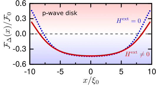
FIG. 10. (Color online) Condensation energy density \mathcal{F}_\Delta obtained with an external field (solid line) and without an external field (dotted line). The calculations are carried out for a p -wave superconducting disk. All the parameters are set to be the same as those of Fig. 8.
