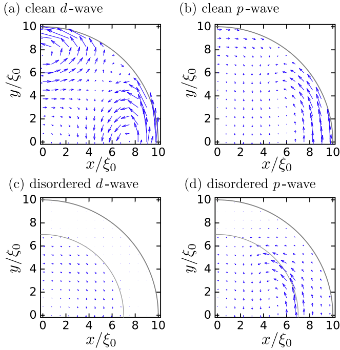
FIG. 6. (Color online) Spatial distribution of the current density on a superconducting disk. The results for a d -wave and a p -wave superconductor with a clean surface ( w = 0, \xi/\ell = 0.0 ) are shown in (a) and (b), respectively. The results for a disk with a rough surface are shown in (c) and (d). The outer circles indicate the edge of the disk and the inner circles in (c) and (d) indicate the effective interface between the clean region and the disordered region. The parameters are set to the same values as those in Fig. 2.
