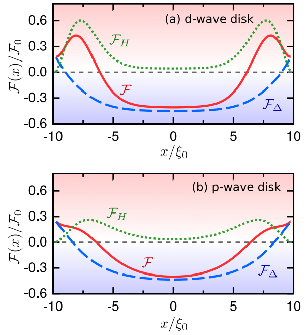
FIG. 9. (Color online) Condensation energy density and energy density of a magnetic field for \alpha = 0 . The results for a d -wave disk and those for a p -wave disk are plotted in (a) and (b), respectively. \mathcal{F} , \mathcal{F}_\Delta , and \mathcal{F}_H are indicated by solid lines, broken lines, and dotted lines, respectively. All of the energy densities are normalized to \mathcal{F}_0 = N_0 \Delta_0^2/2 , which is the condensation energy density of a homogeneous s -wave superconductor. All the parameters are set to be the same as those of Fig. 8.
