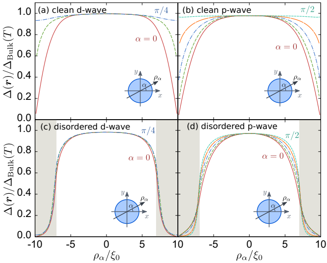
FIG. 4. (Color online) Amplitudes of pair potentials in real space for several azimuthal angles \alpha measured from the x axis. The results for a d -wave disk with \ell/\xi_0 = 0.0 and \ell/\xi_0 = 1.0 are shown in (a) and (c), respectively. Since the pair potential is fourfold symmetric, we plot its spatial profile for \alpha = 0, \pi/8 , and \pi/4 . The results for a p -wave disk with \ell/\xi_0 = 0.0 and \ell/\xi_0 = 1.0 are shown in (b) and (d), respectively. The pair potentials for \alpha = 0, \pi/8, \pi/4, 3\pi/8, \pi/2 (from bottom to top) are shown since the results are twofold symmetric. The pair potentials are normalized to \Delta_{\text{bulk}}(T) . All the parameters are set to be the same as those of Fig. 2. The shadowed areas in (c) and (d) indicate the disordered regions.
