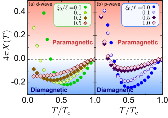
FIG. 7. (Color online) Temperature dependencies of the whole disk susceptibility X(T) for the d -wave (a) and the p -wave (b) disk.
