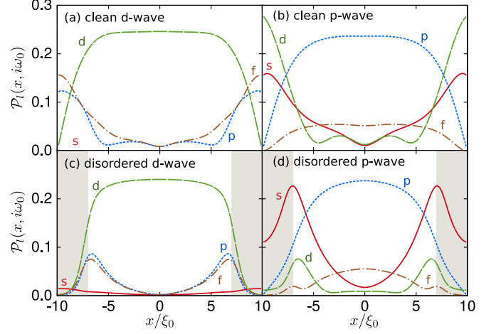
FIG. 5. (Color online) Spatial dependencies of the decomposed pairing functions at the lowest Matsubara frequency on the x axis for (a) a clean d -wave, (b) a clean p -wave, (c) a disordered d -wave, and (d) a disordered p -wave disk. The parameters are set to the same values as those in Fig. 2. The shadowed areas indicate the disordered regions.
