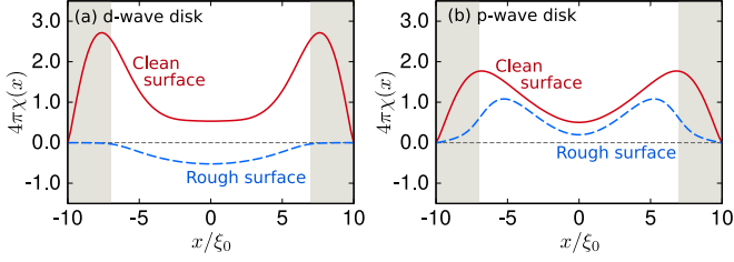
FIG. 3. (Color online) Local susceptibilities on the x axis (i.e., y = 0 ). The results for a d -wave disk and for a p -wave disk are plotted in (a) and (b), respectively. All the parameters are set to be the same as those of Fig. 2. The solid and the broken lines indicate the results for the disk with the clean surface and those with the rough surface, respectively. The shadowed areas indicate the disordered regions.
