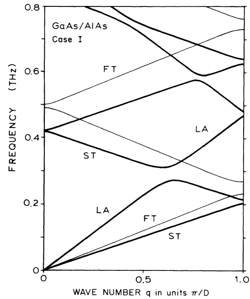
FIG. 2. Dispersion curves of acoustic phonons propagating in the (001) GaAs/AlAs superlattice with layer thickness of d_1 = d_2 = 40 Å. [Case I of Fig. 1(b).] The wave number q_{\max} of the zone boundary phonons is 3.927 \times 10^6 \text{ cm}^{-1} .
