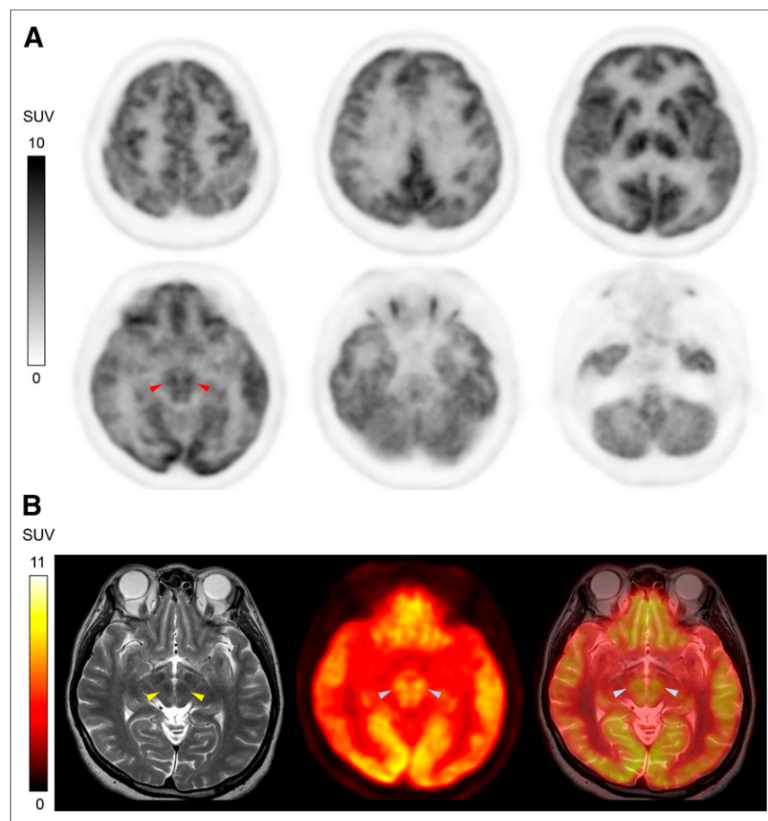
FIGURE 1. A representative case. (A) Bilateral RN indicates areas of higher metabolism (arrowheads). (B) Coregistration with T2-weighted MR images confirmed that high ^{18}\text{F} -FDG uptake corresponded to low-signal-intensity areas in midbrain, indicating RN (arrowheads).
