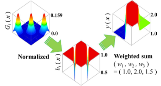
Fig. 3. Gaussians, normalized Gaussians, and output of NGnet.
