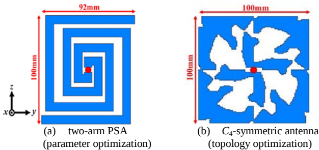
Fig. 5 Selected optimized antennas
