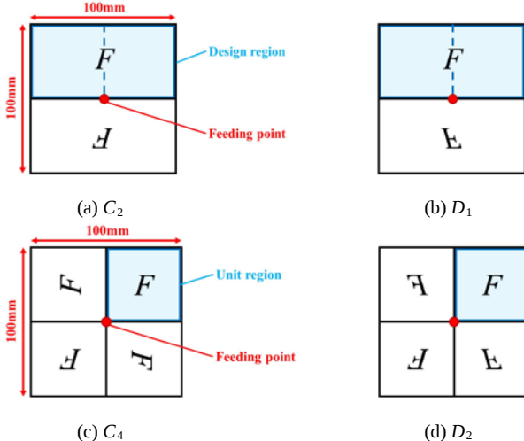
Fig. 2 Symmetry of antennas
