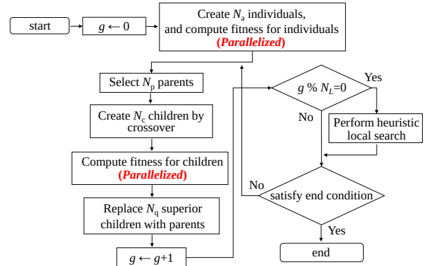
Fig. 3. Flow of parallelized NGnet-MTO.
