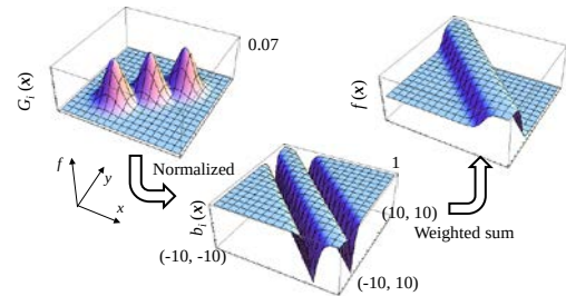
Fig. 1. Output of NGnet in case of 2D input. region, and all the Gaussian have the same isotropic deviations.
