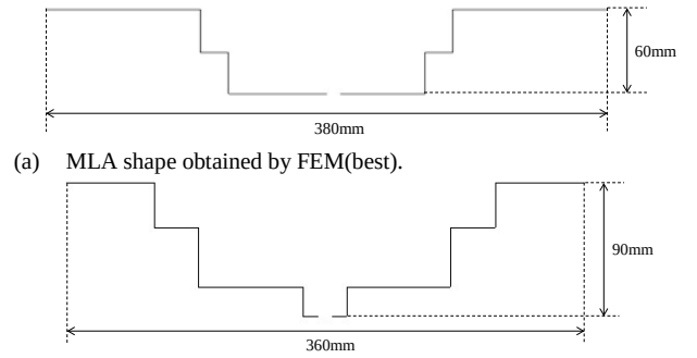
(a) MLA shape obtained by FEM(best). (b) MLA shape obtained by FEM-MOR(best). Fig. 2 MLA shapes obtained by optimization.
