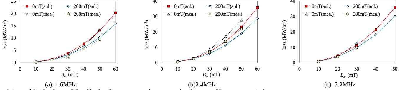
Fig. 6 Loss of SMC, where solid and broken lines represent the computed and measured losses, respectively.
