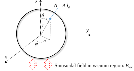
Fig. 2 Eddy current in a sphere immersed in uniform field.
