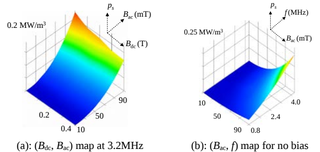
Fig. 7. Loss surface constructed by Akima method.
