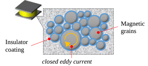
Fig. 1. Structure of soft magnetic composite.
