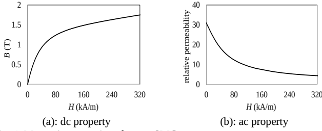
Fig. 4 Magnetic properties of target SMC.
