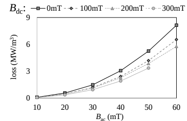
Fig. 3 Measured losses of SMC at 800kHz.
