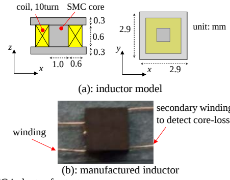
Fig. 8. SMC inductor for test.
