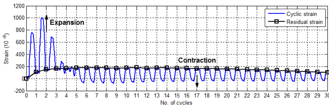
Fig. 2 Strain behavior during 30 cycles (water saturated, sealed and without thermal strain) (Sicat et al. , 2013).
