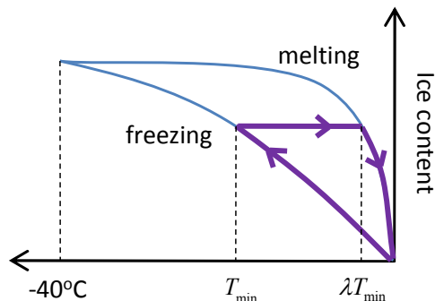
Fig. 5 Freezing and melting curve used in the analysis.
