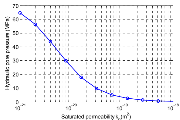
Fig. 16 Hydraulic pore pressure reduction as permeability increases (cooling rate= 15^\circ\text{C/h} , S_r=95.8\% ).
