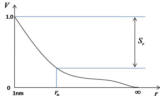
Fig. 3 Typical cumulated pore size distribution.
