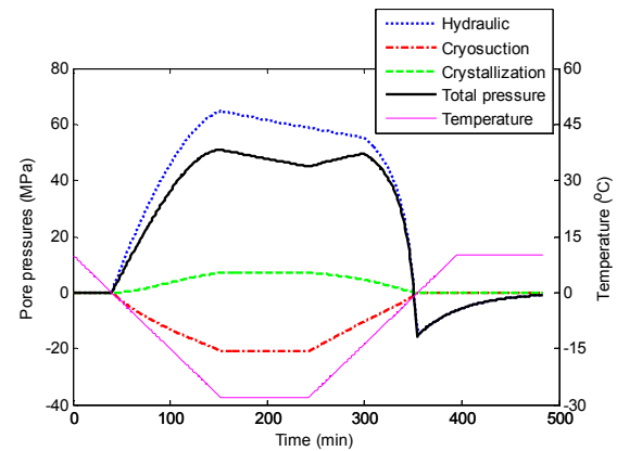
Fig. 10 Simulated hydraulic, crystallization and cryosuction pressures.
