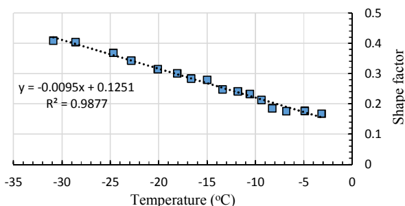
Fig. 8 Pore shape factor as a function of freezing point, based on Sun (2010a).
