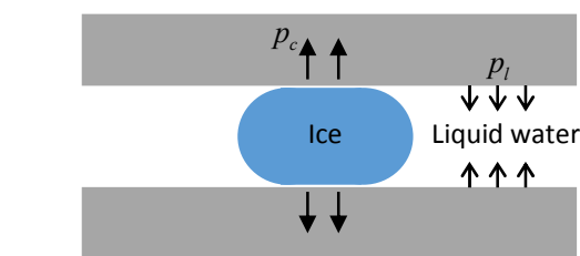
Fig. 7 Crystallization pressure and cryosuction pressure in a cylindrical pore.
