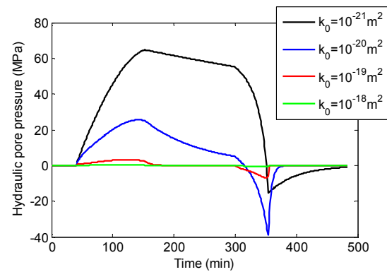
Fig. 12 Calculated hydraulic pore pressure with different permeability.
