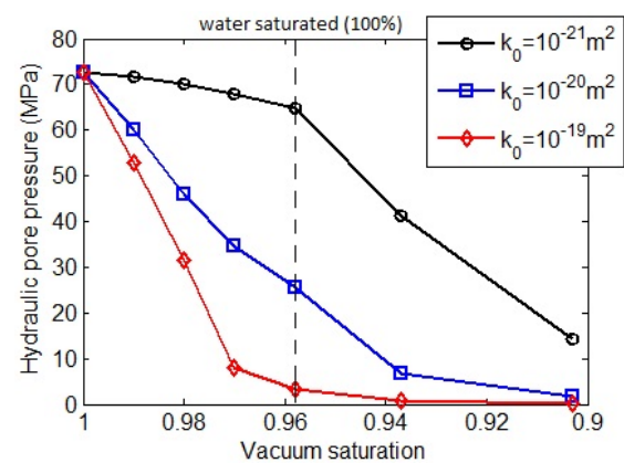
Fig. 14 Hydraulic pore pressure (peak value) change with vacuum saturation degree (cooling rate= 15^\circ\text{C/h} ).
