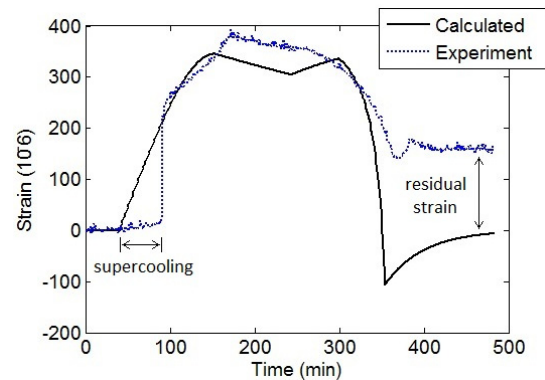
Fig. 11 Calculated strain and experimental test (first cycle, k_0 = 10^{-21} \text{ m}^2 ).
