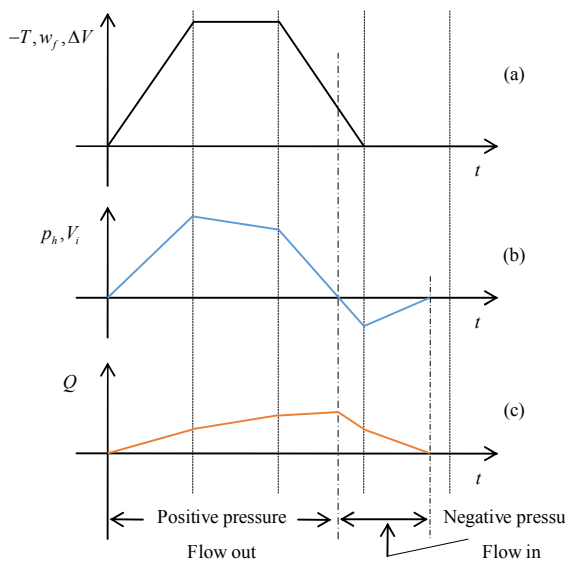
Fig. 4 Change of each parameters (a) temperature ( -T ), frozen water amount ( w_f ), total increased volume ( \Delta V ) (b) hydraulic pressure ( p_h ), volume balanced by deformation ( V_i = \Delta V - Q ) (c) the released flow ( Q ).
