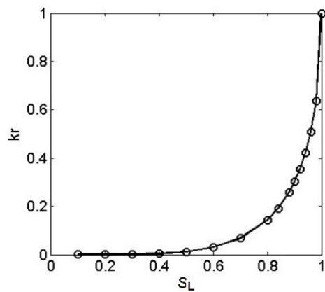
Fig. 6 Relative permeability to liquid saturation degree.
