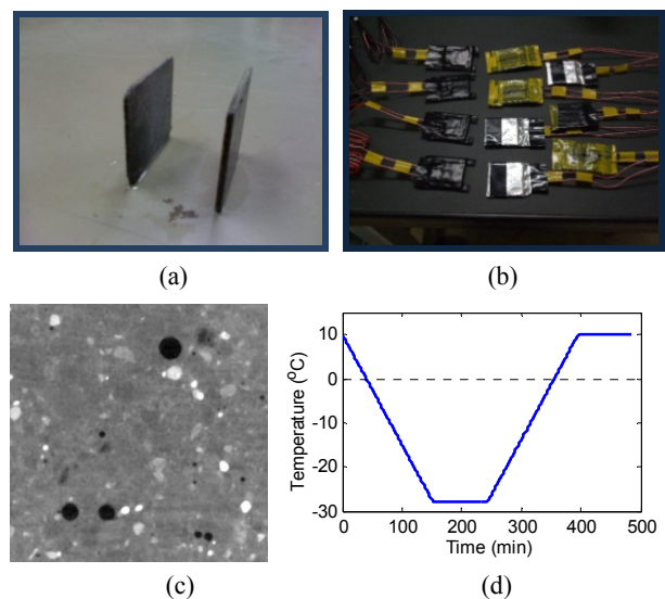
Fig. 9 Outline of the experiment (a) 40 \times 40 \times 2\text{mm} cut specimens; (b) sealed specimens; (c) X-ray CT scanning ( 6.2 \times 6.2\text{mm} ).
