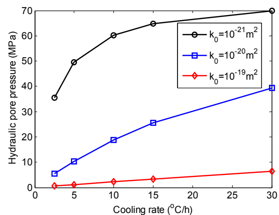
Fig. 15 Hydraulic pore pressure change with cooling rate ( S_r=95.8\% ).
