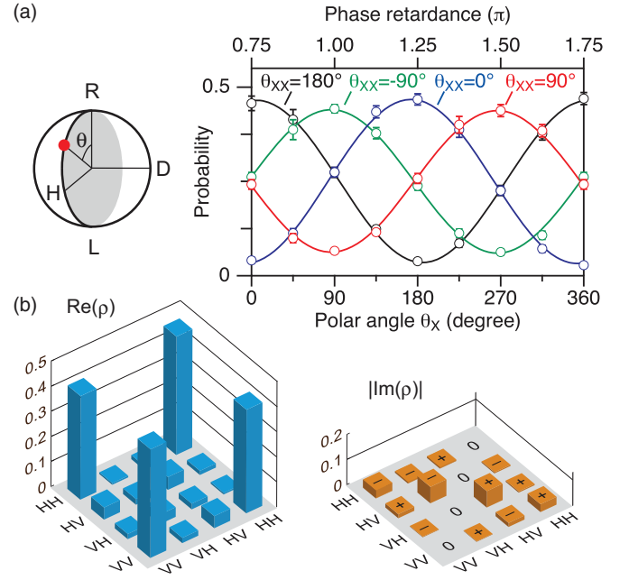
FIG. 3. (Color online) (a) Normalized coincidence counts as a function of the X polarization angle ( \theta_X ) for four different values of the XX polarization ( \theta_{XX} ). The error bars include only Poissonian noise. The sinusoidal fits are also shown by lines. (b) Tomographic representation of the measured two-photon state. The density matrix is reconstructed using coincidence counts for 36 projection bases. The absolute values are plotted for the imaginary part of the matrix, and their signs are shown in the top of each element.
