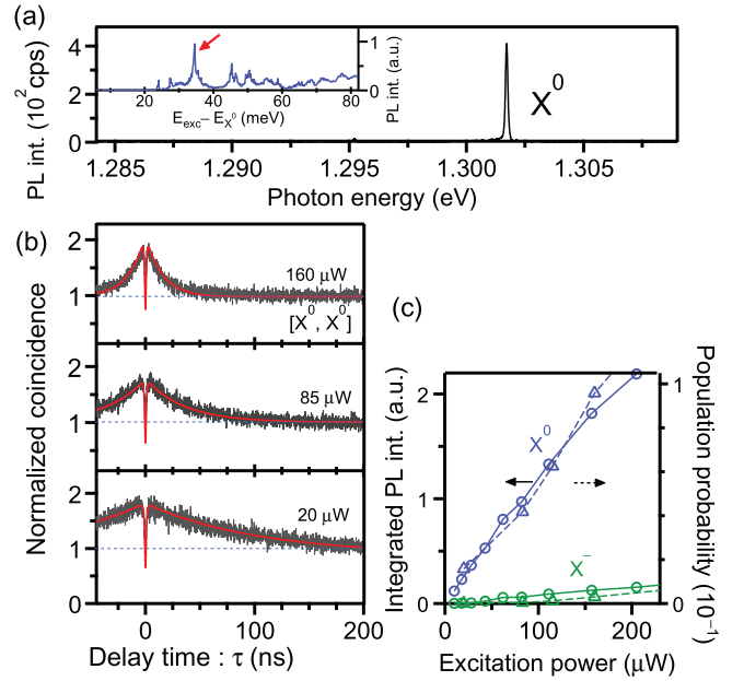
FIG. 5. (Color online) (a) \mu\text{-PL} spectrum under quasiresonant excitation with the same QD at 20 \mu\text{W} excitation. X^0 is exclusively populated. \mu\text{-PLE} spectrum with X^0 emission is shown in the inset. (b) Autocorrelation functions for X^0 under quasiresonant excitation. Slower decay of the bunching peaks is distinct in comparison to nonresonant excitation. (c) Steady-state solutions (triangles) compared with measured PL intensities for X^0 and X^- emissions (circles). In contrast to Fig. 4(b), the |X^0\rangle state is predominantly populated.
