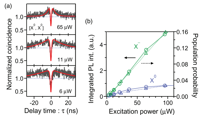
FIG. 4. (Color online) (a) Autocorrelation functions for the X^0 at three excitation powers. Decay of the bunching peak at \tau \sim 0 becomes slower as the excitation power decreases. (b) Steady-state solutions of the rate equations (triangles) compared with measured PL intensities for X^0 and X^- emissions (circles). Circles (triangles) indicate the integrated PL intensities (calculation). Right axis is obtained after appropriate scaling to the PL intensity.
