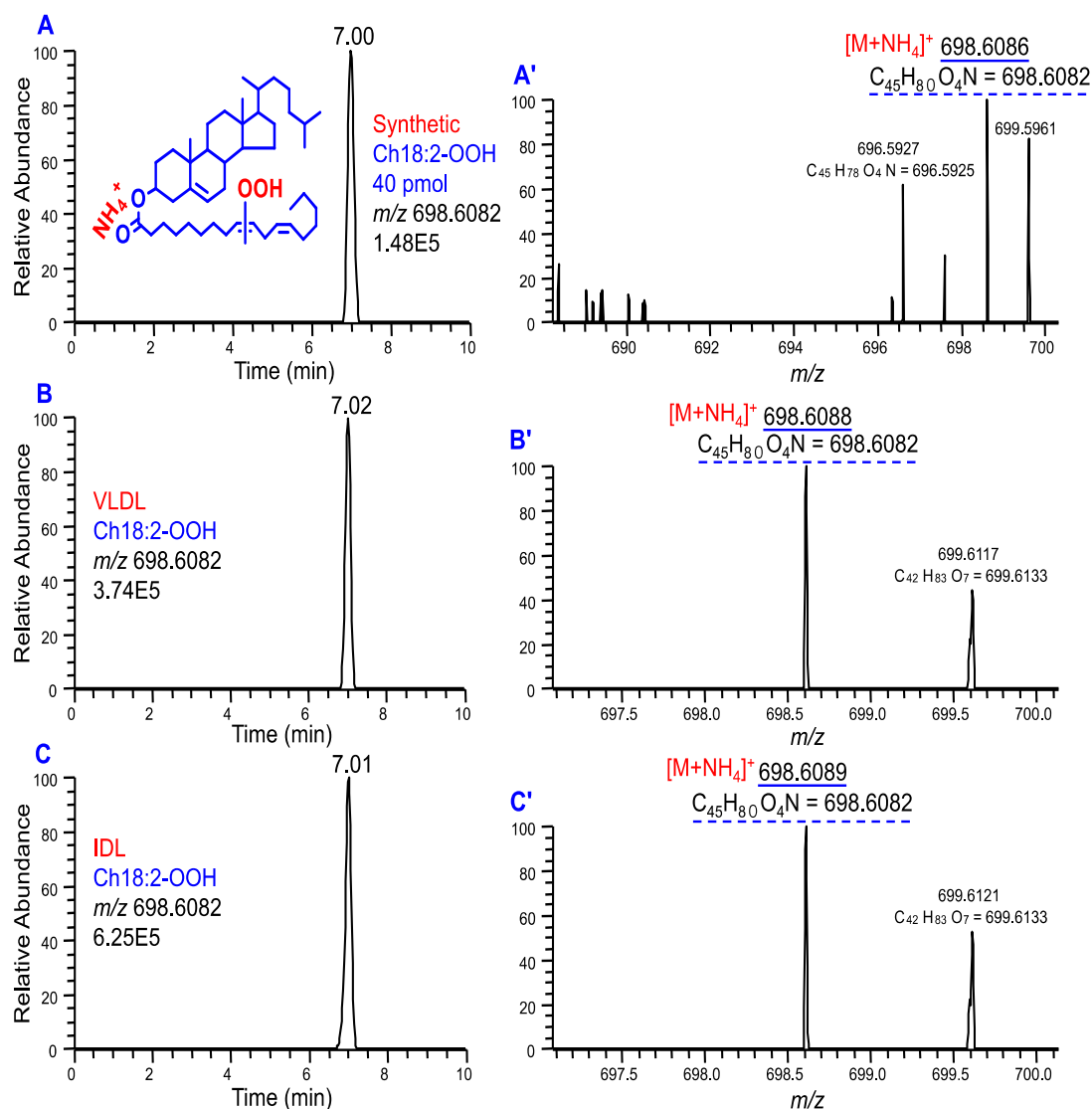
Figure 2.2 LC/LTQ Orbitrap profiles of cholesteryl linoleate monohydroperoxide (Ch18:2-OOH) in positive-ion mode. (A) extracted ion ( m/z 698.6082) chromatogram of synthetic Ch18:2-OOH; (A') mass spectrum of peak associated with retention time at 7.00 min in (A); (B) extracted ion ( m/z 698.6082) chromatogram of VLDL; (B') mass spectrum of peak associated with retention time at 7.02 min in (B)= Ch18:2-OOH; (C) extracted ion ( m/z 698.6082) chromatogram of IDL; (C') mass spectrum of peak associated with retention time at 7.01 min in (C)= Ch18:2-OOH
