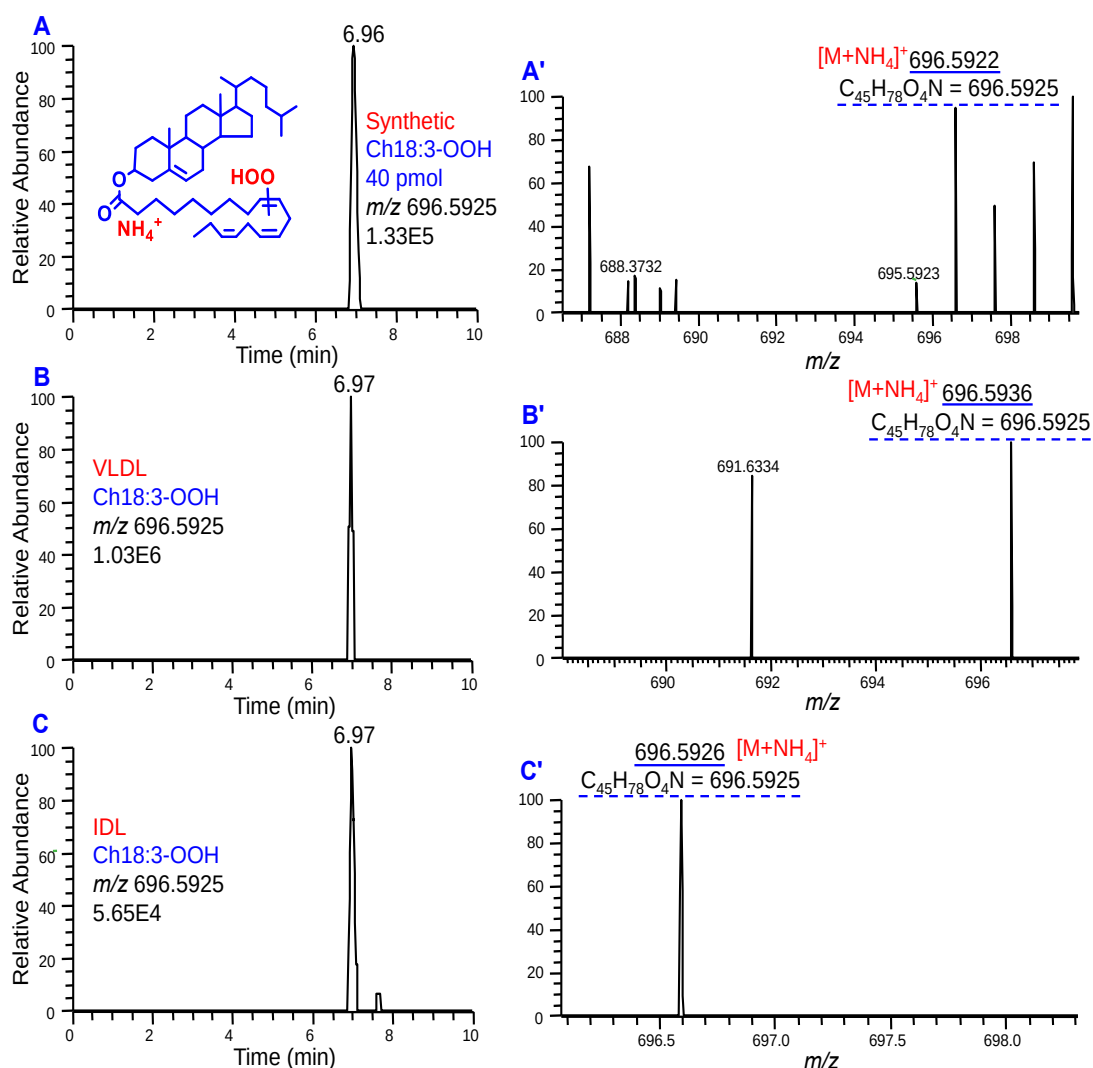
Figure 2.3 LC/LTQ Orbitrap profiles of cholesteryl linolenate monohydroperoxide (Ch18:3-OOH) in positive-ion mode. (A) extracted ion ( m/z 696.5925) mass chromatogram of synthetic Ch18:3-OOH; (A') mass spectrum of peak associated with retention time at 6.96 min in (A); (B) extracted ion ( m/z 696.5925) mass chromatogram of VLDL; (B') mass spectrum of peak associated with retention time at 6.97 min in (B)= Ch18:3-OOH; (C) extracted ion ( m/z 696.5925) mass chromatogram of IDL; (C') mass spectrum of peak associated with retention time at 6.97 min in (C)= Ch18:3-OOH
