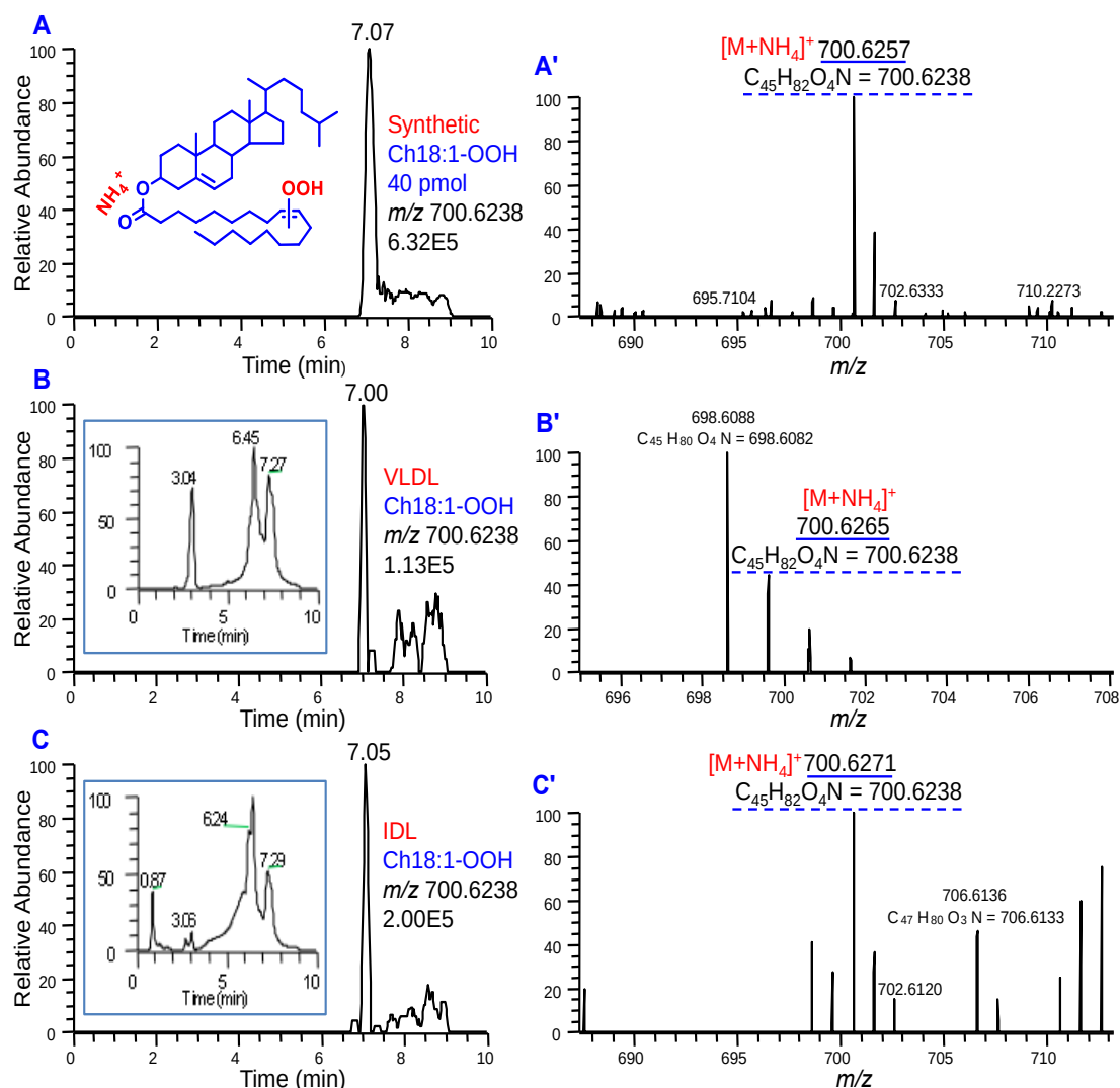
Figure 2.1 LC/LTQ Orbitrap profiles of cholesteryl oleate monohydroperoxide (Ch18:1-OOH) in positive-ion mode. (A) extracted ion ( m/z 700.6238) chromatogram of synthetic Ch18:1-OOH; (A') mass spectrum of peak associated with retention time at 7.07 min in (A); (B) total ion chromatogram (inside square) and extracted ion ( m/z 700.6238) chromatogram of VLDL; (B') mass spectrum of peak associated with retention time at 7.00 min in (B)= Ch18:1-OOH; (C) total ion chromatogram (inside square) and extracted ion ( m/z 700.6238) chromatogram of IDL; (C') mass spectrum of peak associated with retention time at 7.05 min in (C)= Ch18:1-OOH
