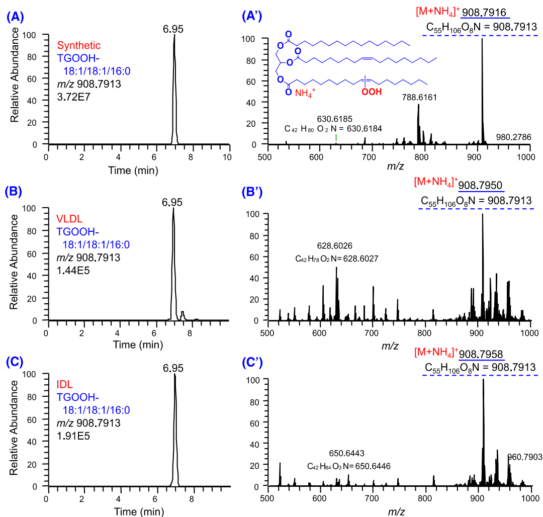
Figure 3.4 LC/LTQ Orbitrap profiles of TGOOH-18:1/18:1/16:0 in positive-ion mode: (A) extracted ion ( m/z 908.7913) chromatogram of synthetic TGOOH-18:1/18:1/16:0 (40 pmol); (A') mass spectrum of peak associated with retention time of 6.95 min in (A); (B) extracted ion ( m/z 908.7913) chromatogram of VLDL; (B') mass spectrum of peak associated with retention time at 6.95 min in (B) = TGOOH-18:1/18:1/16:0; (C) extracted ion ( m/z 908.7913) chromatogram of IDL; (C') mass spectrum of peak associated with retention time at 6.95 min in (C) = TGOOH-18:1/18:1/16:0.
