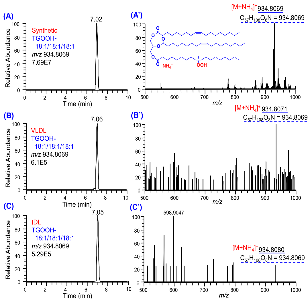
Figure 3.5 LC/LTQ Orbitrap profiles of triolein monohydroperoxide (TGOOH-18:1/18:1/18:1) in positive-ion mode: (A) extracted ion ( m/z 934.8069) chromatogram of synthetic TGOOH-18:1/18:1/18:1 (40 pmol); (A') mass spectrum of peak associated with retention time of 7.02 min in (A); (B) extracted ion ( m/z 934.8069) chromatogram of VLDL; (B') mass spectrum of peak associated with retention time at 7.06 min in (B) = TGOOH-18:1/18:1/18:1; (C) extracted ion ( m/z 934.8069) chromatogram of IDL; (C') mass spectrum of peak associated with retention time at 7.05 min in (C) = TGOOH-18:1/18:1/18:1.
