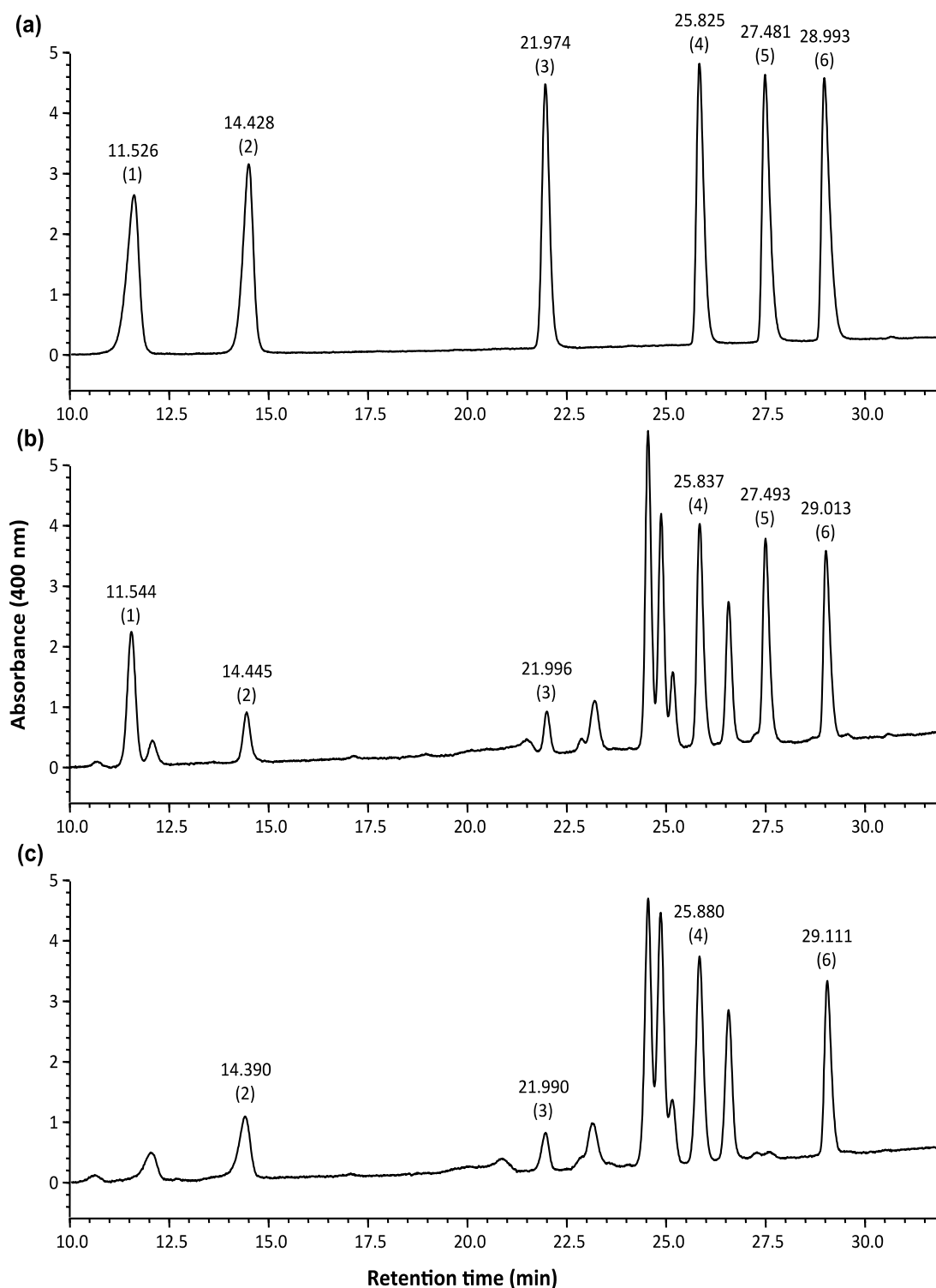
Figure 4.2. HPLC chromatogram of the 2-nitrophenylhydrazine derivatives of (a) mixture of standard fatty acids, (b) fatty acid from a human plasma spiked with FA10:0 (200 \mu\text{mol/L} ) and (c) fatty acids from a fasting human plasma. Peaks: 1, capric (FA10:0); 2, undecanoic (FA11:0); 3, myristic (FA14:0); 4, palmitic (FA16:0); 5, heptadecanoic (FA17:0); and 6, stearic acid (FA18:0).
