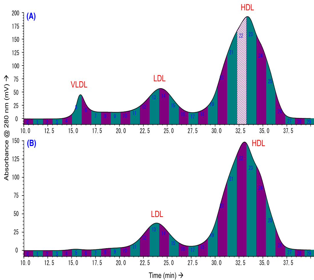
Figure 3.6 Size-exclusion HPLC chromatograms of lipoproteins from (A) total lipoprotein fraction ( d < 1.225 ), (B) lipoprotein fraction of d = 1.019-1.225 isolated by ultracentrifugation.
