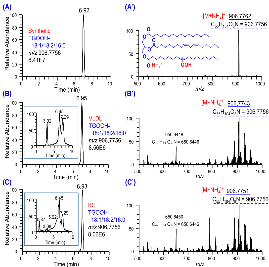
Figure 3.3 LC/LTQ Orbitrap profiles of TGOOH-18:1/18:2/16:0 in positive-ion mode: (A) extracted ion ( m/z 906.7756) chromatogram of synthetic TGOOH-18:1/18:2/16:0 (40 pmol); (A') mass spectrum of peak associated with retention time of 6.92 min in (A); (B) total ion chromatogram (inside square) and extracted ion ( m/z 906.7756) chromatogram of VLDL; (B') mass spectrum of peak associated with retention time at 6.95 min in (B) = TGOOH-18:1/18:2/16:0; (C) total ion chromatogram (inside square) and extracted ion ( m/z 906.7756) chromatogram of IDL; (C') mass spectrum of peak associated with retention time at 6.93 min in (C) = TGOOH-18:1/18:2/16:0.
