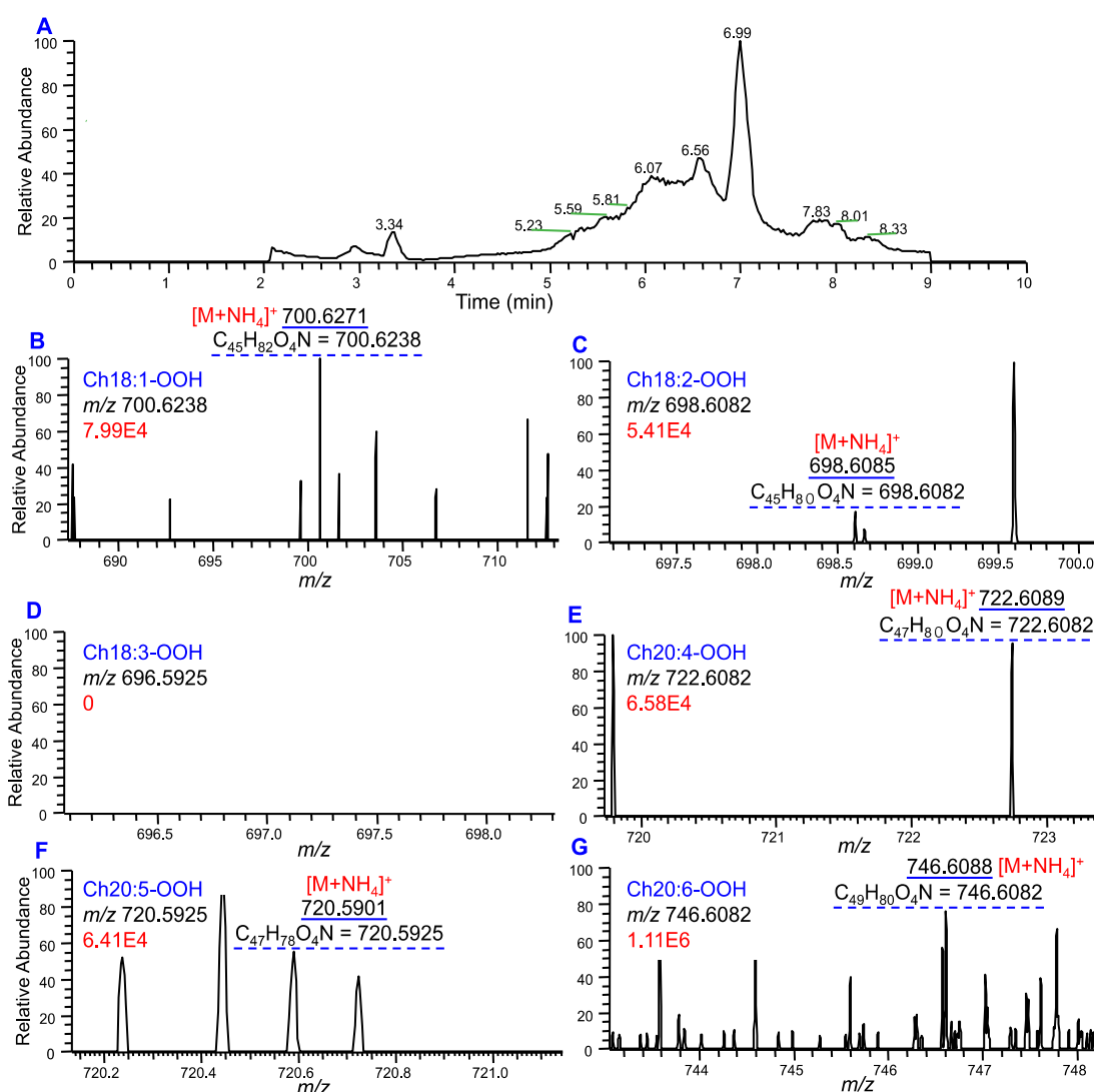
Figure 2.4 LC/LTQ Orbitrap profiles of cholesteryl ester hydroperoxides present in a plasma sample in positive-ion mode. (A) total ion chromatogram of plasma extract; (B) mass spectrum showing m/z 700.6271 = Ch18:1-OOH; (C) mass spectrum showing m/z 698.6085 = Ch18:2-OOH; (D) Ch18:3-OOH ( m/z 696.5925) is absent in plasma; (E) mass spectrum showing m/z 722.6089 = Ch20:4-OOH; (F) mass spectrum showing m/z 720.5901 = Ch20:5-OOH; (G) mass spectrum showing m/z 746.6088 = Ch20:6-OOH
