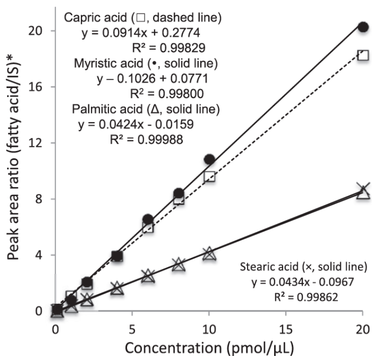
Figure 4.3 Calibration curves for 2-nitrophenylhydrazine derivatives of capric (FA10:0), myristic (FA14:0), palmitic (FA16:0) and stearic acid (FA18:0).
