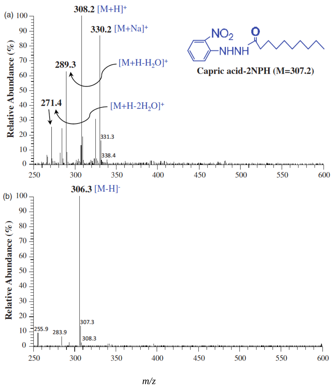
Figure 4.1 Electrospray ionization mass spectra of NPH-derivative of capric acid in (a) positive- and (b) negative-ion mode. Key diagnostic ion peaks are annotated in bold type with their m/z value.
