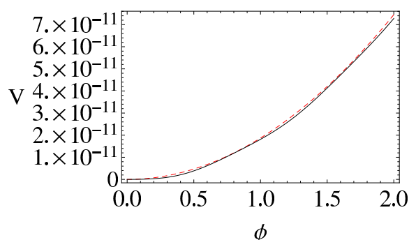
Figure 3. The scalar potential V versus the inflaton value \phi . Along with figure 2, the black-solid curve corresponds to the scalar potential (3.34) with modulations for the parameter b/L = 1/5 and \langle \text{Re } U^2 \rangle = 1.2 . On the other hand, the red-dotted curve corresponds to the leading scalar potential (3.24) without modulations for the same parameters.
