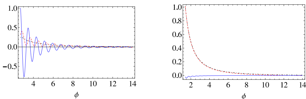
Figure 2. The behavior of the slow-roll parameters, \epsilon , \eta and \xi^2 , which correspond to black-dotdashed, red-dashed and blue-solid curves, respectively. In the left (right) panel, we set b/L = 1/5 ( 1/10 ) and \langle \text{Re } U^2 \rangle = 1.2 ( 2.4 ).
