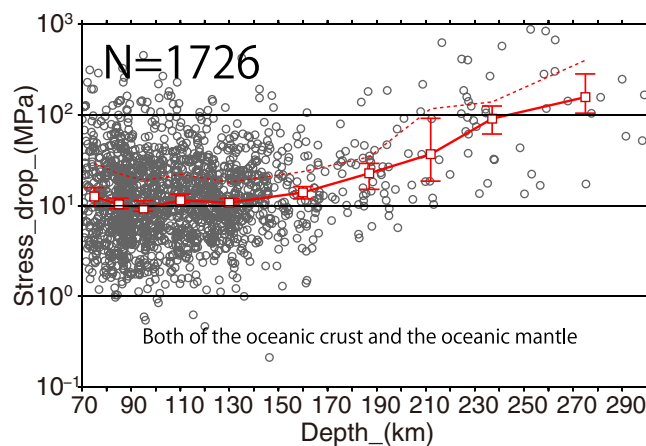
Figure 3. Estimated stress drops for all intraslab earthquakes plotted against depth. Gray dots show individual stress drops for events. Red open squares and red error bars, respectively, denote the median stress drops and the 95% confidence level for the median stress drop at depths of 70–80 km, 80–90 km, 90–100 km, 100–120 km, 120–140 km, 140–175 km, 175–200 km, 200–225 km, 225–250 km, and 250–330 km. The 95% confidence levels for the median stress drops are based on the results of 2000 times bootstrap resampling. The red line and colored dashed line, respectively, connect the median stress drop points and the average stress drop points.
