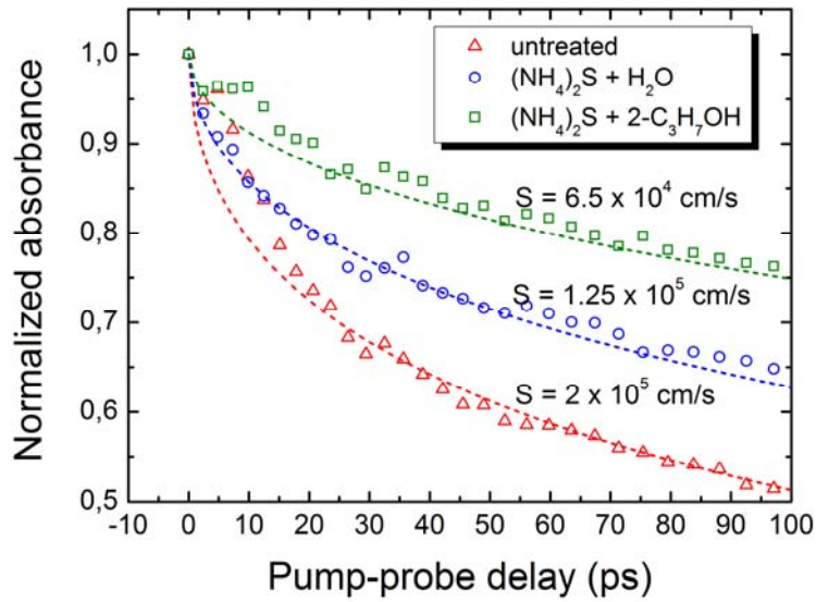
Fig. 2. Fitting of the initial absorbance decay for untreated n-GaAs(100) sample, as well as for samples passivated with aqueous and alcoholic sulfide solutions. Dots represent experimental data and dashed lines indicate fitting results obtained using a solution of the one-dimensional diffusion equation from Ref. [22].
