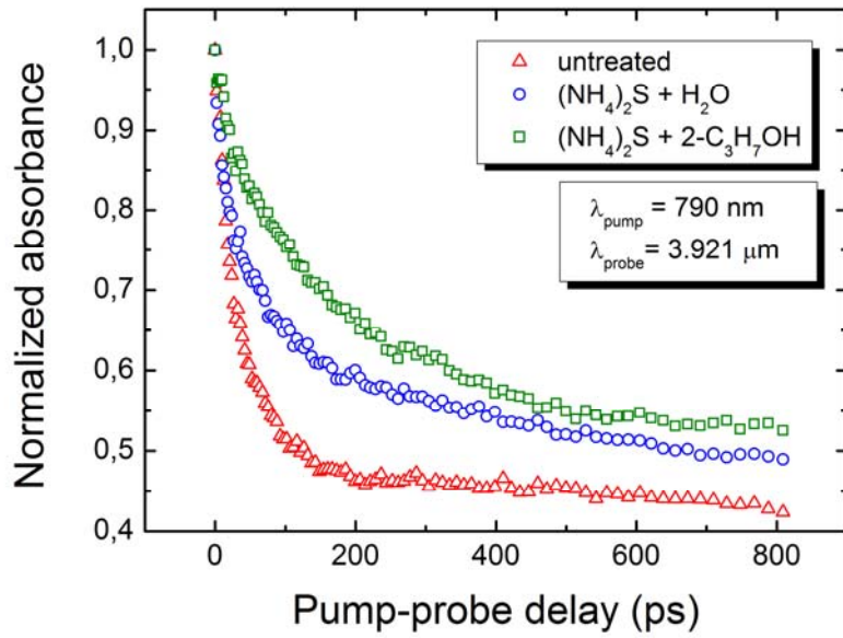
Fig. 1. Normalized time-resolved absorbance decay for untreated n-GaAs(100) sample, as well as for samples passivated with aqueous and alcoholic sulfide solutions as measured with femtosecond visible pump infrared probe technique.
