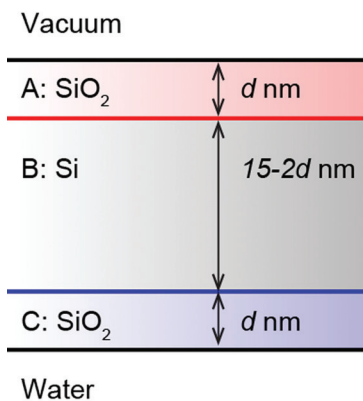
(A) Before Oxidation
