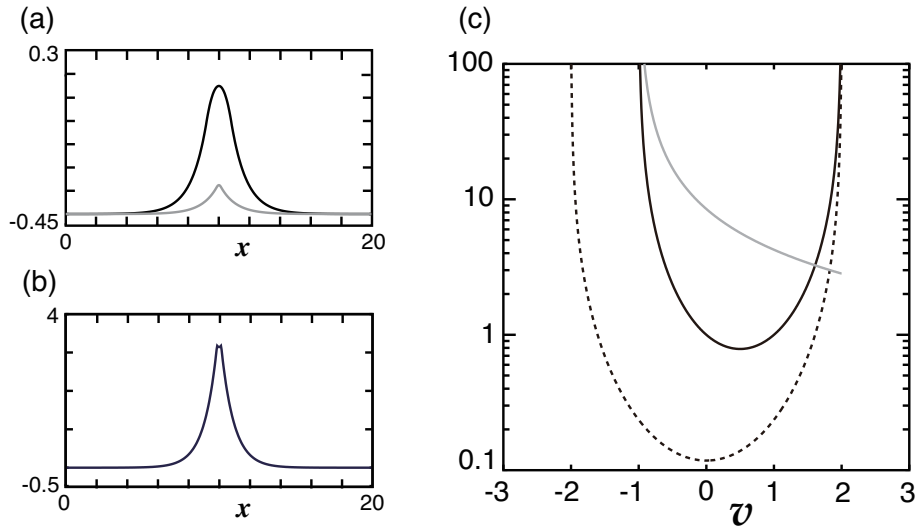
FIGURE 4. (a) The profiles of large (black) and small (gray) stationary pulse solutions obtained from Eqs. (24) for \vartheta = 0.1 . The other parameters are the same as in Fig. 3. For the u -component, the profiles of these pulse solutions are both given by the rectangular function u(x; \phi_2^{(0)}, \phi_1^{(0)}) in Eq. (3). From the bifurcation curve in Fig. 3(b), we see that the large pulse is stable, while the small one is unstable. (b) The profile of eigenfunction associated with the unstable real eigenvalue of the small pulse solution. (c) The graphs of M_0(v) (broken curve), M_1(v) (gray solid curve) and M(v) (black solid curve) in Eq. (22).
