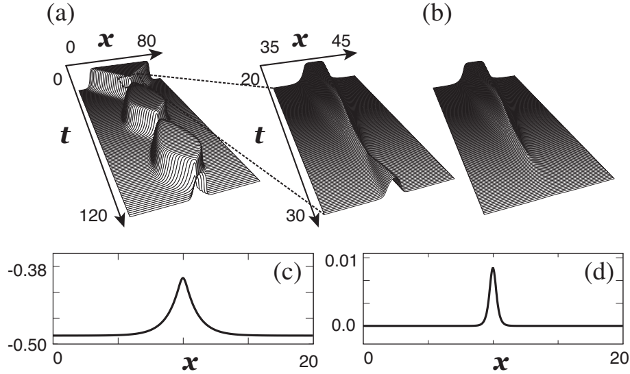
FIGURE 1. (a), (b): Bird-view plot for the colliding interfaces of a front-back pulse system observed numerically in the original RD system (1) with \vartheta(x) = \varsigma . The horizontal and vertical axes represent the space and the time, respectively and only v(x, t) is shown. Transition from standing breather to annihilation occurs when \varsigma = \varsigma_s \approx 0.0137267 . The other parameters are set to (\epsilon, D, \tau) = (0.05, 1.0, 0.160) . (a) The interfaces collide and the pulse eventually settles down to a standing breather. When \varsigma is slightly larger than \varsigma_s , it settles down to the background constant solution as shown in (b). Just after the collision between the two interfaces, the pulse remains as a small stationary pulse for a certain time. (c) Profile of a codimension one stationary pulse solution and (d) profile of its associated eigenfunction whose unstable eigenvalue is 22.72. In (c) and (d), the profiles of the v component are depicted.
