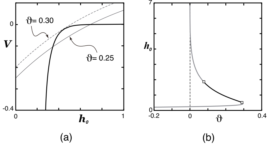
FIGURE 3. (a) The two graphs of h_0 = -\sqrt{2}\epsilon \log(-V/\sqrt{2}M(V)) (solid black) and V = \vartheta - e^{-h_0/\sqrt{D}}/2 (solid or broken gray). The vertical axis is the value of v^{(0)} at the interface V and the horizontal axis is the pulse width h_0 . Each intersection corresponds to a stationary pulse solution. For \vartheta \approx 0.3 , the graphs are tangent (broken gray curve) and they have two intersections for \vartheta < 0.3 (solid gray curve). (b) By changing \vartheta and plotting h_0 of the intersections of the two graphs in (a), we obtain a bifurcation curve for the stationary pulse solution for mHS (23). A pair of pulse solutions are created via a saddle-node bifurcation around \vartheta = 0.3 , the larger of which diverges in width at \vartheta = 0 . On the other hand, the smaller one continues to exist for \vartheta < 0 . Furthermore, the spectrum obtained from Eqs. (25) for linear stability reveals that, as \vartheta is varied, the larger pulse undergoes Hopf bifurcations twice (indicated by the open squares) and that the smaller one is always unstable with one positive real eigenvalue. The black and gray curves indicate stable and unstable solutions, respectively. The other parameters are fixed as \tau = 0.160 , D = 1.0 , \epsilon = 0.05 .
