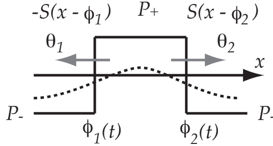
FIGURE 2. Schematic figure for a pulse constructed by two front solutions. We set \phi_1(t) = -\theta_1 t + l_1(t) and \phi_2(t) = \theta_2 t + l_2(t) where \theta_1 := \theta(v_1) and \theta_2 := \theta(v_2) are treated as constant, which vary with time when the scalar equation (4) is coupled with the v -field (indicated by the dotted line).
