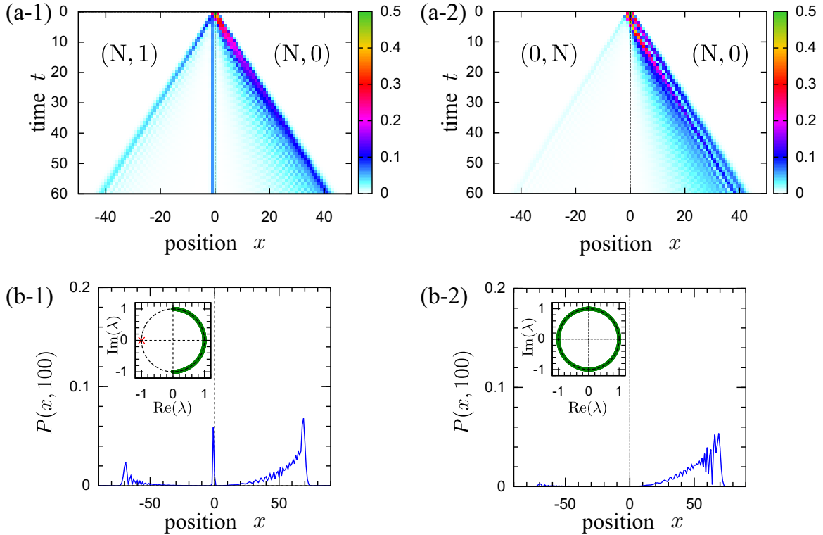
FIG. 3. (Color online) Examples of bound states as signatures of a topological phase transition in split-step Hadamard walks. Top: Contour maps of the probability distribution P(x,t) in the x - t plane for the quantum walk (a-1) U_B(\theta_\gamma) , Eq. (38), and (a-2) U_B(\theta_\delta) , Eq. (39). The topological numbers (\nu_0, \nu_\pi) for the negative and positive x regions are shown in the figures. A letter “N” means that the topological number for the corresponding quasienergy cannot be defined because of the gap closing. (b) The position dependence of the probability distribution P(x,t) at t = 100 . The eigenvalues of the time-step operators are shown in the insets as in Figs. 1(b-1) and 1(b-2).
