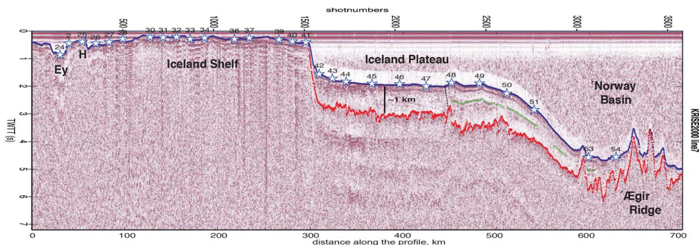
Figure 2. KRIS7 reflection section, bandpass filtered 20–40 Hz with a 48 dB/oct drop-off and plotted with an AGC window of 1 s. Seafloor picks are blue and basement picks red. OBS stations with data, white stars. Green picks mark reflector R2, dashed line is an unconformity. Within the TFZ, the Eyjafjardaráll basin (Ey) marks the southern continuation of the Kolbeinsey Ridge, and the Híllinn (H) volcanic system the northward continuation of the NVZ. The Iceland Shelf has thin sediment cover whereas sediment thickness of 1–1.5 km (1–1.5 s) characterizes the Iceland Plateau.
