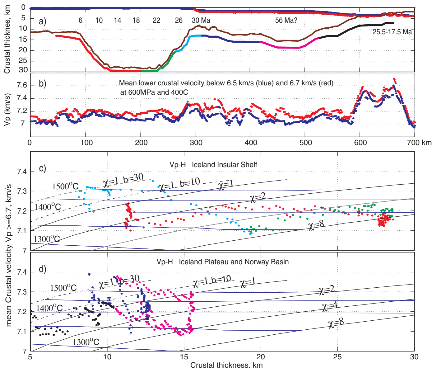
Figure 7. Average lower crustal velocity (Vp) and crustal thickness (H) along KR1SE7. (a) Plot of seafloor topography (blue), basement (red), and Moho with colors indicating different regions discussed in text. Brown line shows total crustal thickness (from basement to Moho). Crustal age is based on the NUVEL-1A spreading model [DeMets et al. , 1994] with a half-spreading rate of 0.9 cm/yr at 105°, and distance from magnetic anomaly 5 (10 Ma), at 125 km. (b) Average lower crustal velocity along the KR1SE7 line, below the 6.5 (blue), and the 6.7 (red) km/s isovelocity contours. Higher-velocity anomalies are associated with narrow (~30 km) lower crustal high-velocity domes. Similar domes characterize both active and extinct central volcanoes of Iceland. (c) and (d) Vp-H across the Iceland Shelf and the Iceland Plateau to the Aegir Ridge, respectively. A 100°C decrease in mantle temperatures is inferred across the Iceland shelf and from the eastern margin of the Iceland Plateau towards the Aegir Ridge. Cessation of spreading at the Aegir Ridge was associated with a marked decrease in inferred mantle temperatures, in line with decreasing supply of partial melt.
