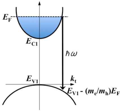
FIG. 7. (Color online) Schematic band diagram of a doped QW. E_{C1} and E_{V1} are the lowest subband energies in the conduction and valence band, respectively. k_t is the wave vector in the QW plane. The arrow in the downward direction indicates the photon emission with the photon energy of \hbar\omega from the Fermi level to the valence band QW state.
