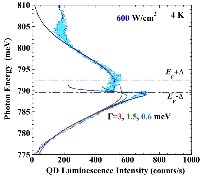
FIG. 8. (Color online) Lifetime-broadening dependence of the fitted luminescence spectra for the one observed with the excitation power of 600 W/cm 2 .
