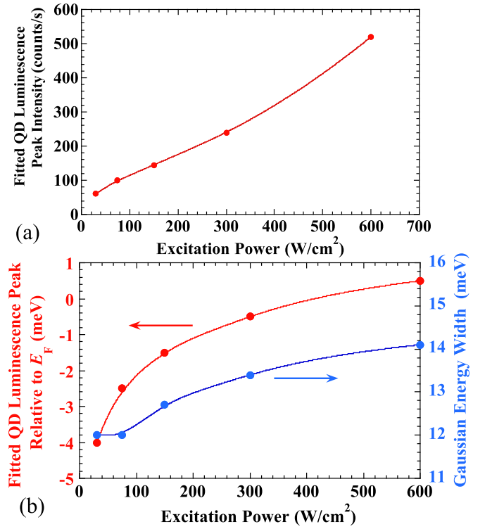
FIG. 6. (Color online) Excitation power dependence of the Gaussian-function parameters used for fitting the spectra, shown in Fig. 4. (a) The QD PL peak intensity. (b) The QD PL peak energy relative to the electron Fermi energy (given by the energy separation \delta ) and Gaussian half energy width.
