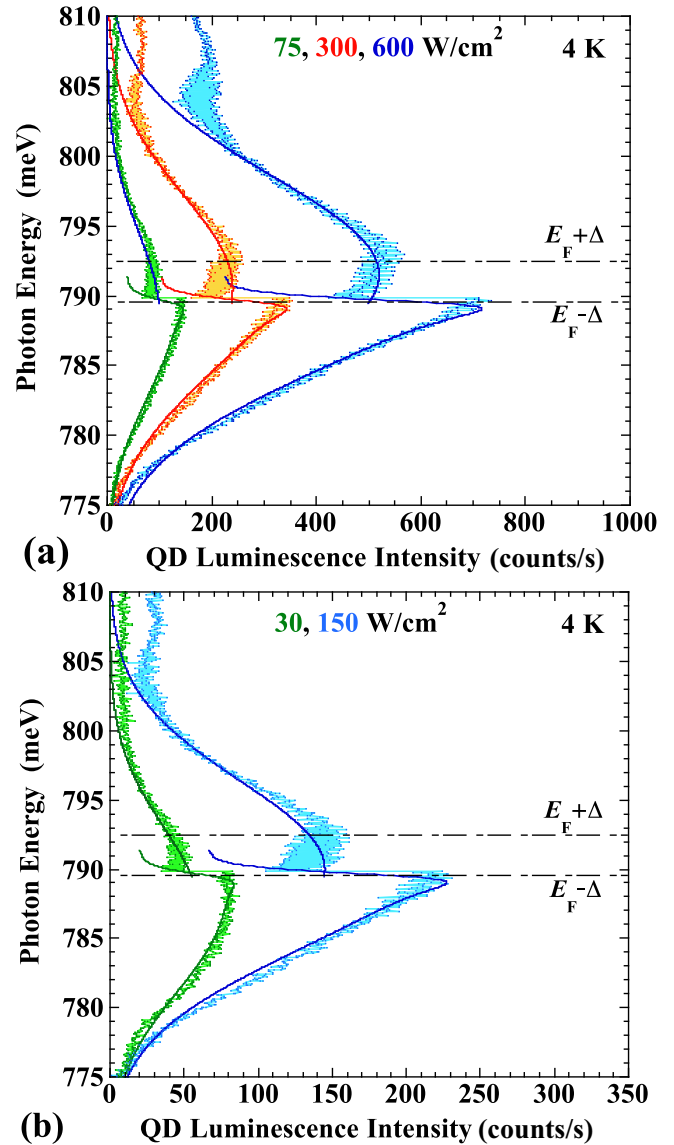
FIG. 4. (Color online) Measured excitation power dependence of QD luminescence spectra. The measured photon counts are connected with neighboring counts with thin lines: (a) 75, 300, and 600 W/cm 2 ; (b) 30 and 150 W/cm 2 . The solid lines are fitting with the parameters of E_F = 791.0 meV and \Delta = 1.42 meV.
