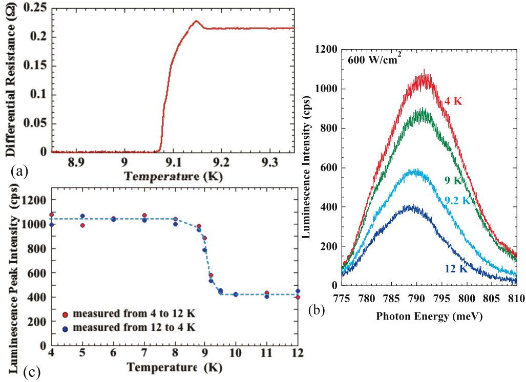
FIG. 2. (Color online) (a) Temperature dependence of differential resistance measured on the deposited Nb layer. (b) Temperature dependence of InAs-QD luminescence spectra. (c) Temperature dependence of QD luminescence peak intensity. To confirm the relation to T_C = 9.07 K of Nb, measured data for the temperature rising and falling sequences are shown.
