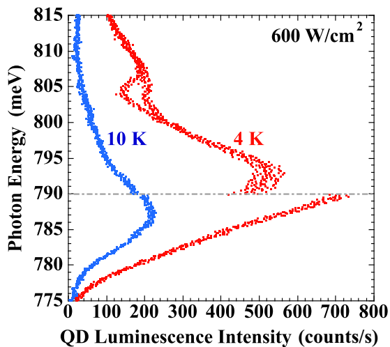
FIG. 3. (Color online) Luminescence spectra observed at 4 and 10 K with 600 \text{ W/cm}^2 excitation power from another pillar with the diameter of 1.5 \mu\text{m} . Only the measured photon counts are plotted without connecting lines. The alternate long and short dashed line is the guide to the eye, indicating the luminescence intensity sharp edge.
