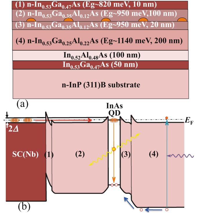
FIG. 1. (Color online) (a) Schematic of InAs QD-based heterostructure sample. (b) Schematic band structure after the Nb deposition on the sample surface. The layers (1)–(4) correspond to those shown in (a). Below T_C , the SC gap 2\Delta opens in the Nb superconductor, and Cooper pairs penetrate into InAs QDs through the semiconductor heterostructure with the proximity effect. Minority holes are generated with the external He-Ne laser irradiation and transported to InAs QDs. A Cooper pair recombines with a pair of holes and generates a pair of photons.
