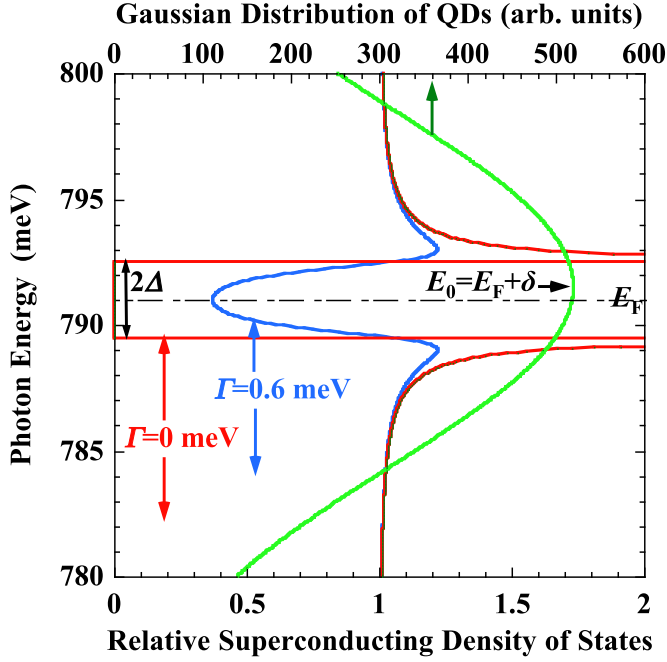
FIG. 5. (Color online) Broadened SC DOS with \Gamma = 0.6 meV and Gaussian distribution of QD energy states employed for the fitting in Fig. 4 are shown. The Gaussian peak is given by E_0 = E_F + \delta , where E_F is the Fermi energy and the energy separation \delta from E_F is given as 0.5 meV for the case of 600 \text{ W/cm}^2 photoexcitation. SC DOS without broadening ( \Gamma = 0 meV) is also shown. 2\Delta is the SC gap.
