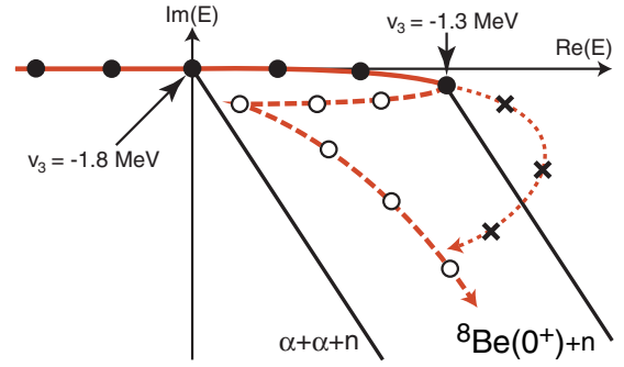
FIG. 4. (Color online) Pole trajectory of the {}^9\text{Be } 1/2^+ state in a complex energy plane by changing the three-body potential. The closed circles represent the poles obtained as isolated three-body resonances in CSM. The open circles and crosses are speculated pole positions for the virtual states and broad resonances, respectively.
