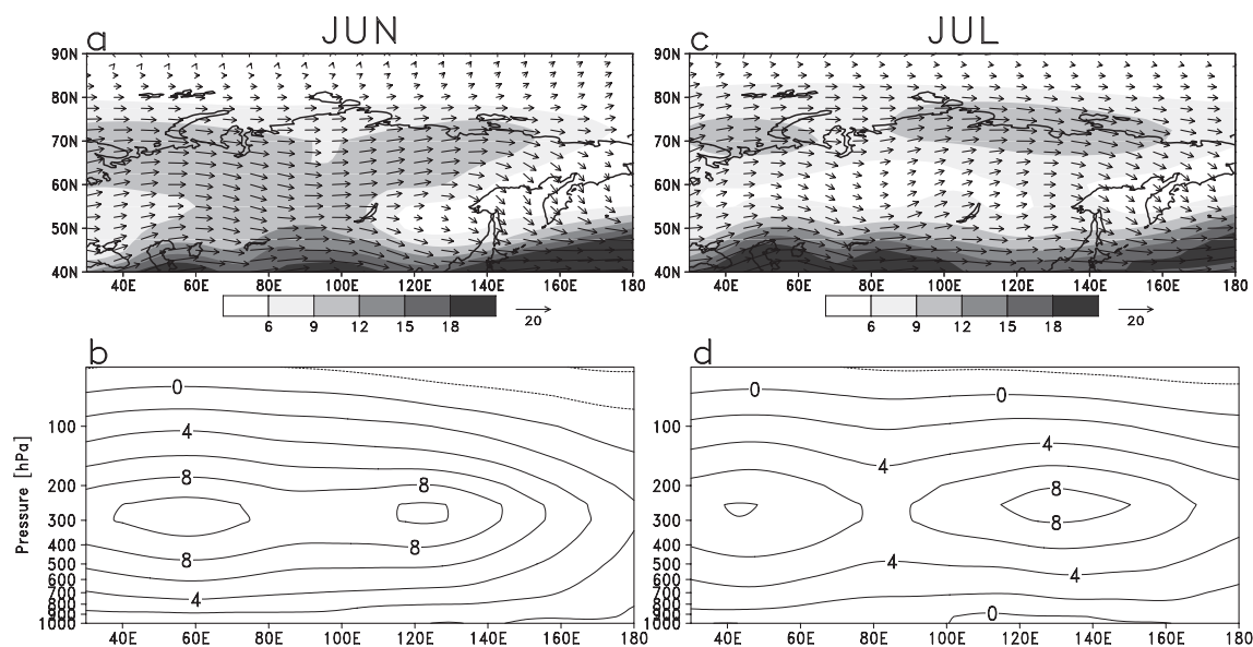
Fig. 5. As in Fig. 3, but for June and July.
