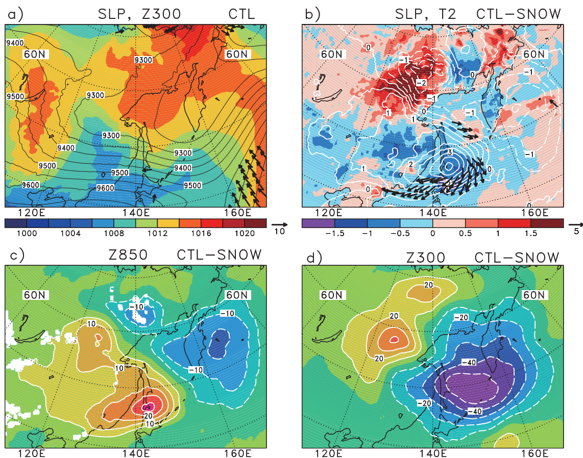
Fig. 9. (a) Distribution of sea-level pressure (shadings; hPa), 10-m wind (arrows; \text{m s}^{-1} ) and 300-hPa geopotential height (50 m contour interval) for the period 9–15 August 2008 in the CTL run. (b) Differences in 2-m air temperature (shadings; ^{\circ}\text{C} ), SLP (0.5 hPa contour interval), 10-m wind (arrows; \text{m s}^{-1} ), (c) 850-hPa and (d) 300-hPa geopotential height between the CTL and SNOW runs.
