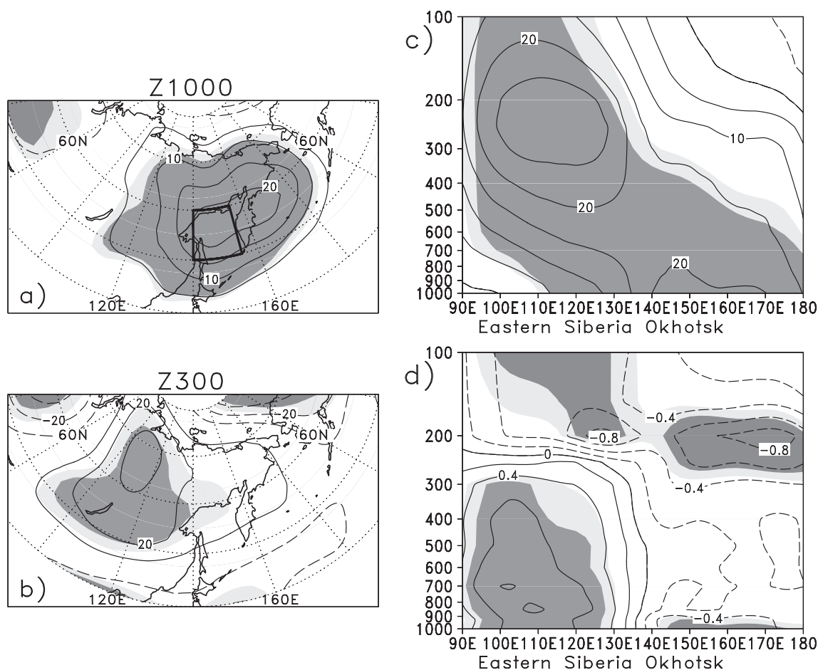
Fig. 2. Monthly atmospheric patterns linearly regressed onto the Okhotsk high index (regions surrounded by thick solid lines: 50–60°N, 140–155°E) in (a) 1000-hPa geopotential height (5 m contour interval) and (b) 300-hPa height (10 m contour interval) based on the NCEP2 reanalysis in August during 1979–2012. (c) Longitude–pressure sections of height (5 m contour interval) and (d) air temperature (0.2 K contour interval) along 55°N. Light and heavy shadings indicate statistical significance at the 95 % and 99 % levels, respectively.
