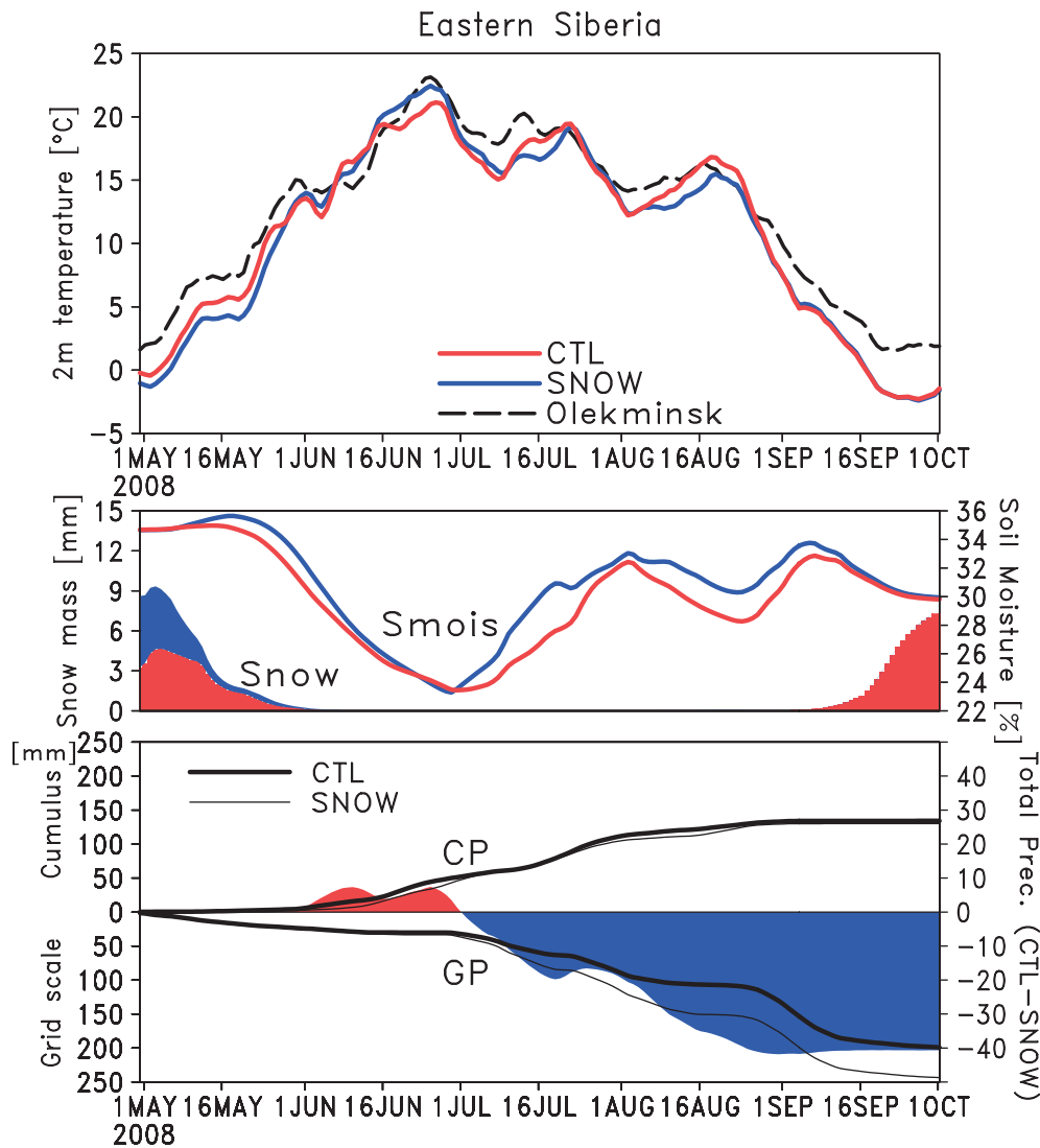
Fig. 7. Time series of 11-day low-pass-filtered surface parameters averaged over eastern Siberia ( 60^{\circ}\text{N} , 120\text{--}130^{\circ}\text{E} ) in the CTL (red shadings and lines) and SNOW (blue shadings and lines) runs from May through September in 2008. Top panel: 2-m air temperature ( ^{\circ}\text{C} ) and observed surface air temperature (dashed line) at Olekminsk ( 60^{\circ}\text{N} , 120^{\circ}\text{E} ) based on station data. Middle panel: snow mass (shadings; mm) and 10–40 cm soil moisture (%). Lower panel: accumulated cumulus precipitation (CP), sub-grid scale precipitation (GP), and total precipitation differences (shadings) between the CTL and SNOW runs.
