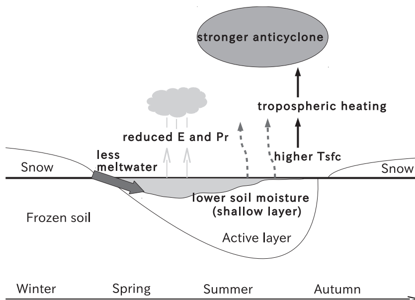
Fig. 1. Schematic diagram of seasonal changes in early-snowmelt years from winter to autumn in eastern Siberia. E : evaporation, Pr : precipitation, and T_{sfc} : surface air temperature (Matsumura and Yamazaki 2012).
