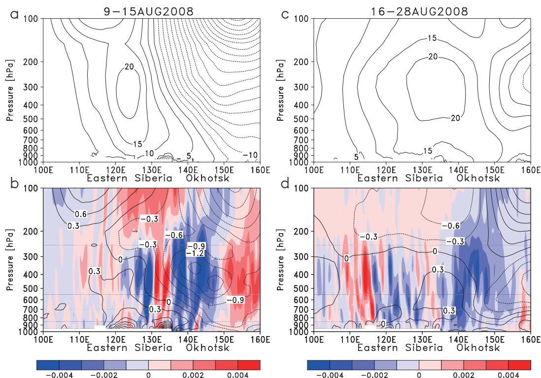
Fig. 11. Longitude-pressure sections of differences in (a) geopotential height (5 m contour interval), (b) air temperature (0.3 K contour interval) and vertical velocity (shadings; \text{m s}^{-1} ) (positive values indicate upward) between the CTL and SNOW runs during 9–15 August 2008 averaged the areas of 50–60°N. (c) and (d): As for (a) and (b), but for during 16–28 August 2008.
