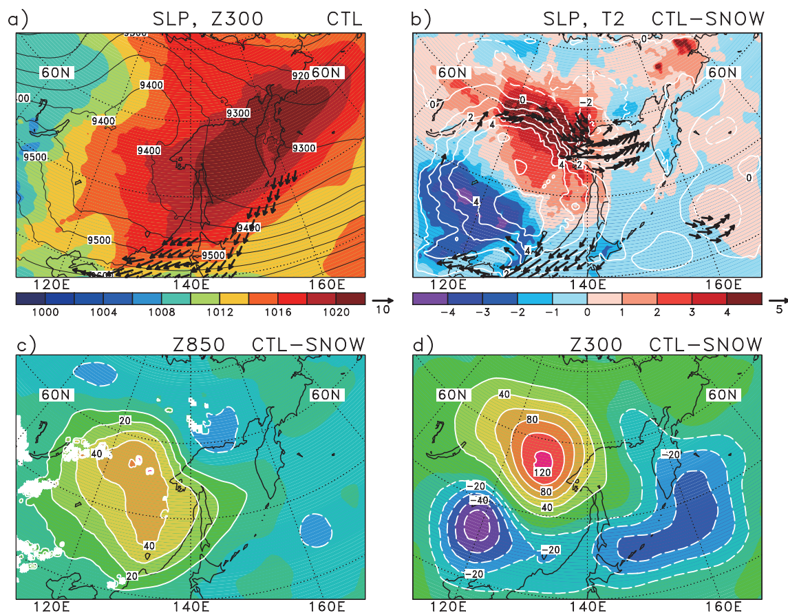
Fig. 12. As in Fig. 9, but for the period 13–27 August 2002.
