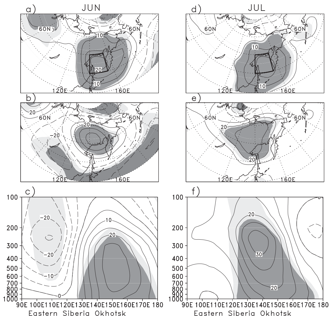
Fig. 4. As in Figs. 2a, 2b, and 2c, but for June and July.
