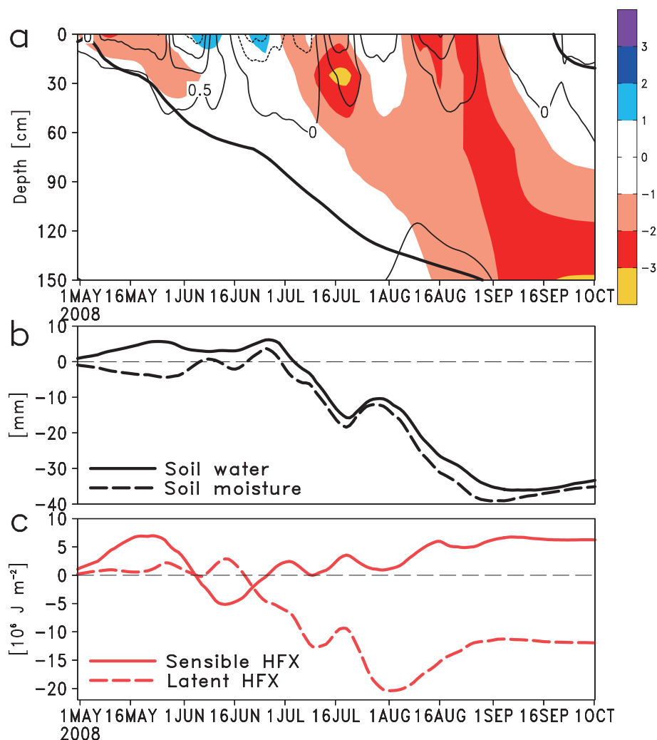
Fig. 8. As in Fig. 7, but for (a) time-depth sections of the CTL – SNOW differences in soil temperature (0.5°C contour interval) and moisture (shadings; %), and (b) time series of the CTL – SNOW differences in vertically accumulated soil moisture (dashed line) and liquid water (solid line) and (c) accumulated upward surface sensible (solid line) and latent (dashed line) heat fluxes. The bold solid contours in (a) indicate 0°C in the CTL run.
