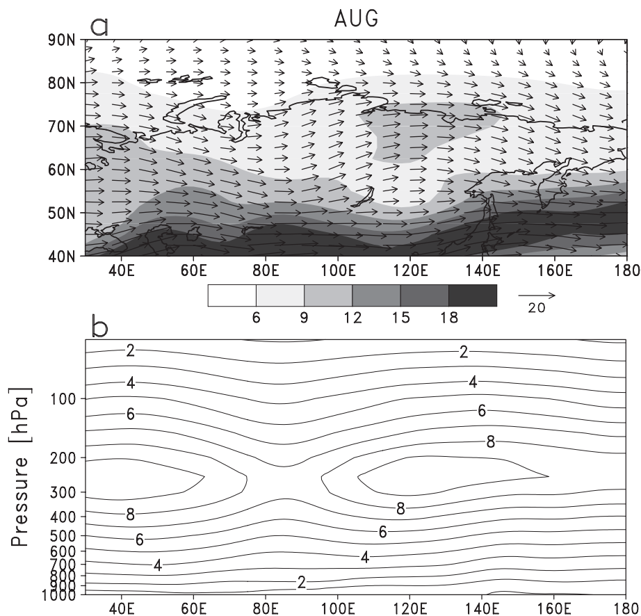
Fig. 3. (a) Climatological 300-hPa zonal wind (shaded; \text{m s}^{-1} ) and vector (arrows; \text{m s}^{-1} ), and (b) longitude-pressure sections of zonal wind ( 1 \text{ m s}^{-1} contour interval) averaged the areas of 60\text{--}70^\circ\text{N} in August for the period 1979–2012.
