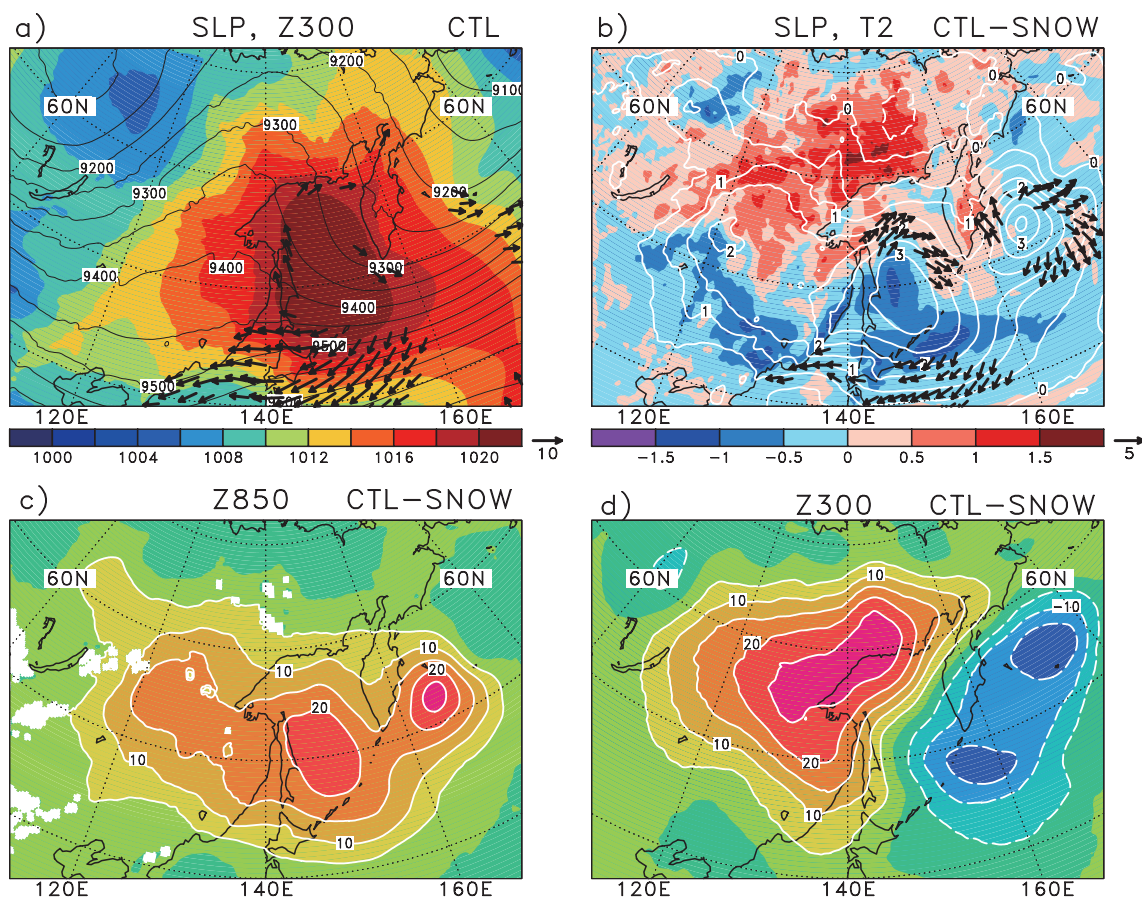
Fig. 10. As in Fig. 9, but for the period 16–28 August 2008.
