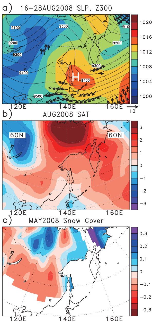
Fig. 6. (a) Typical weather pattern developed in August OH for the period 16–28 August 2008 based on the NCEP2 reanalysis, showing mean sea-level pressure (shadings; hPa), 10-m wind (arrows; \text{m s}^{-1} ), and 300-hPa geopotential height (50 m contour interval). (b) Surface air temperature anomalies ( ^{\circ}\text{C} ) in August 2008 based on the NCEP2 reanalysis. (c) Observed snow cover ratio anomalies in May 2008 based on station data (Yabuki et al. 2011).
