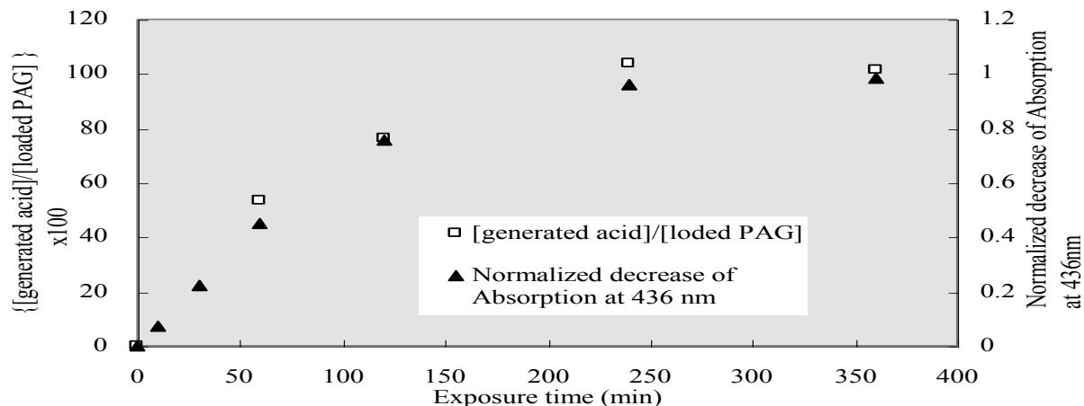
Fig. 5. The ratio of the generated acid concentration against the loaded PAG concentration and normalized decrease of absorption at g-line vs. exposure time plot.
