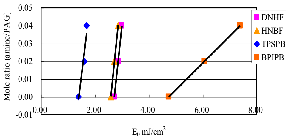
Fig. 3. Relation between amine/PAG ratio and sensitivity
