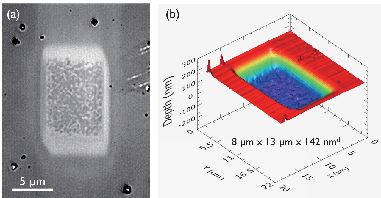
Fig. 1. Sputter crater on Genesis DOS sample. (a) Laser scanning confocal microscope image. (b) 3-D image obtained by atomic force microscope.
