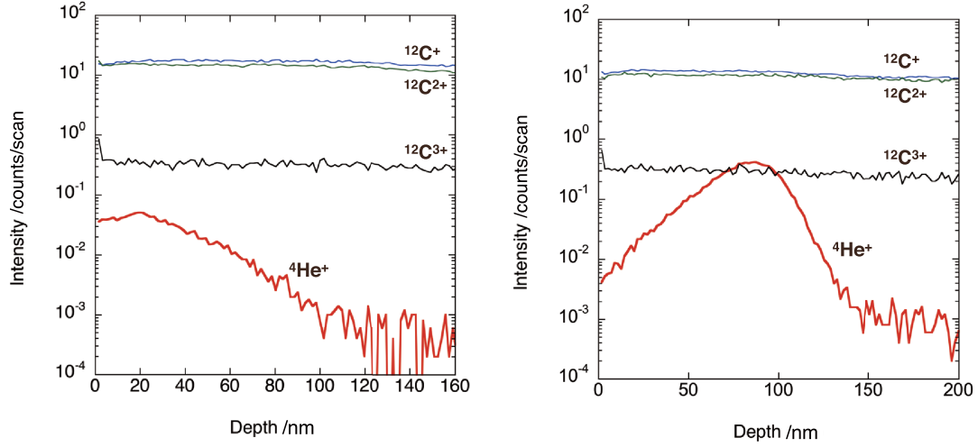
Fig. 3. Depth profile of ion intensity on 2014/3/11. (a) Genesis DOS sample. (b) Ion-implanted DOS sample.
