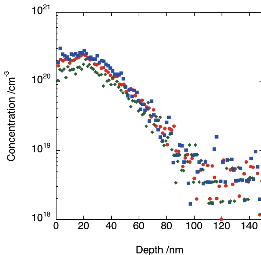
Fig. 5. Depth profile of solar wind ^4\text{He} concentration from Genesis DOS sample. Three independent measurements plotted as circles (2014/3/11), squares (2014/3/12), and diamonds (2014/3/14) are shown.
