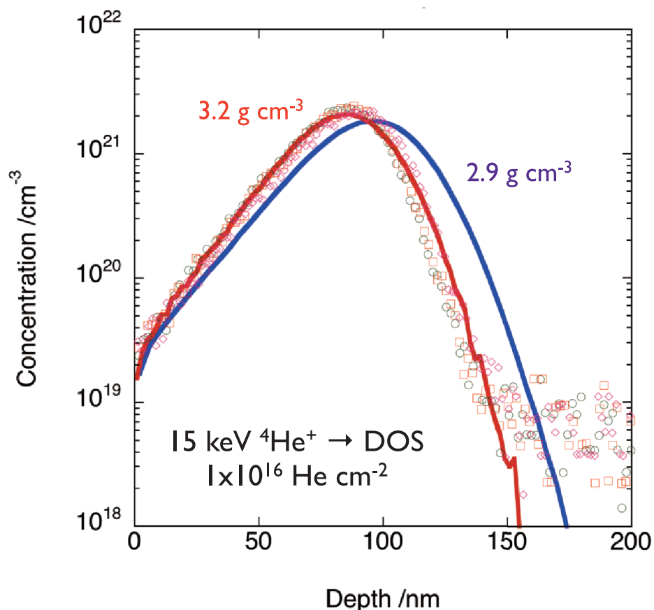
Fig. 4. Depth profile of ^4\text{He} concentration implanted in DOS. Three independent measurements plotted as circles (2014/3/11), squares (2014/3/12), and diamonds (2014/3/14) are shown. Distributions calculated by TRIM simulation are shown by lines. Data are shown in Table S1.
