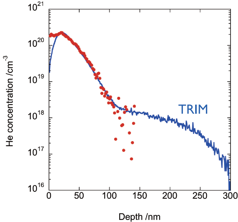
Fig. 6. Average depth profile of solar wind ^4\text{He} into Genesis DOS sample. Circles are from observation with background correction. Line is calculated by TRIM simulation assuming density of 3.2 \text{ g cm}^{-3} using energy distributions of solar wind ^4\text{He} observed by ACE/SWICS (Reisenfeld et al. , 2013).
