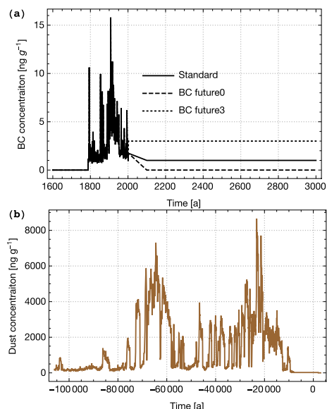
Figure 3. Aerosol time series of (a) black carbon (BC) and (b) dust. (a) The standard BC time series consists of ice core data by McConnell et al. (2007) and projections based on Bauer et al. (2013) with two additional trajectories of the future. In the period before data are available the BC concentration is set to 0. (b) The dust concentration from NGRIP (Ruth, 2007), where the missing Holocene period (after -8 ka) is assigned a constant value of 20 \text{ ng g}^{-1} , and a value of 0 is assumed after the year 2000.
