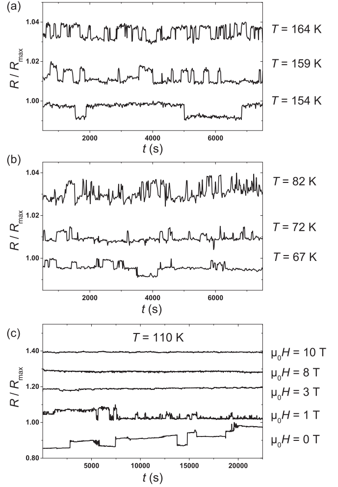
FIG. 2. (a) Random telegraph noise of the single MnAs nanowire and (b) of the bent nanocluster arrangement determined at different temperatures. (c) Suppression of the RTN of the bent nanocluster by an external magnetic field.
