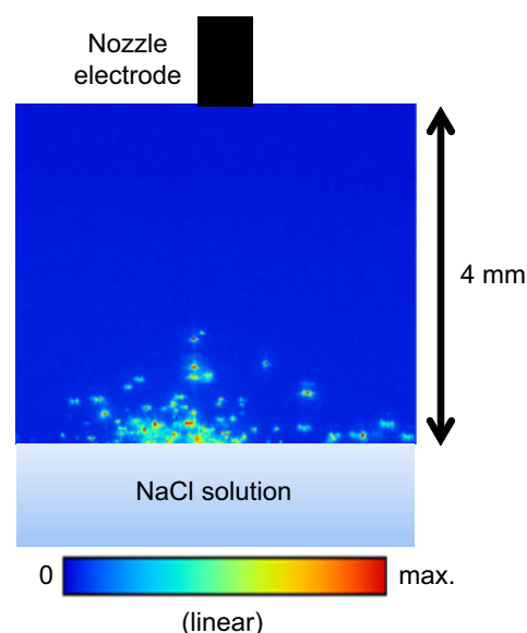
Fig. 5. Distribution of mist in the discharge space, which was examined by laser Mie scattering. The discharge parameters are the same as those in Figure 2.
