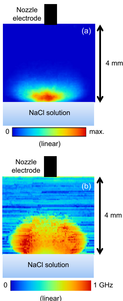
Fig. 4. LIF results for Na at the same discharge parameters as those in Figure 2. (a) Distribution of Na density and (b) distribution of quenching frequency of laser-produced \text{Na}(^2P^o) .
