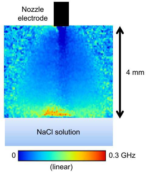
Fig. 3. Distribution of the frequency of collisional quenching for \text{OH}(A^2\Sigma^+) . The discharge parameters are the same as those in Figure 2. This figure roughly represents the distribution of the \text{H}_2\text{O} density.
