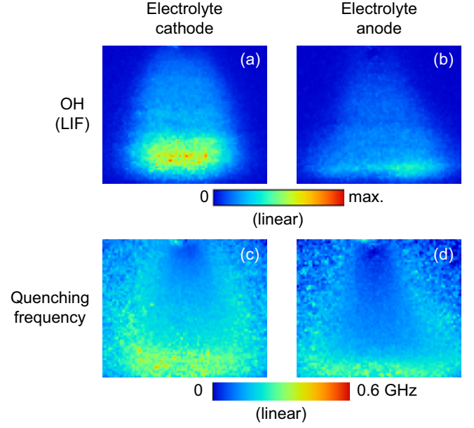
Fig. 7. Comparisons of the LIF images of OH ((a) and (b)) and the spatial distributions of the collisional quenching frequency of OH( A^2\Sigma^+ ) ((c) and (d)), observed when the electrolyte worked as the cathode and the anode.
