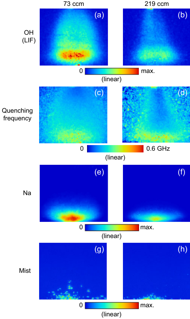
Fig. 6. Comparisons of the LIF images of OH ((a) and (b)), the spatial distributions of the collisional quenching frequency of OH( A^2\Sigma^+ ) ((c) and (d)), the Na densities ((e) and (f)), and the images of laser Mie scattering ((g) and (h)) observed at gas flow rates of 73 and 219 cm. The discharge current was fixed at 40 mA.
