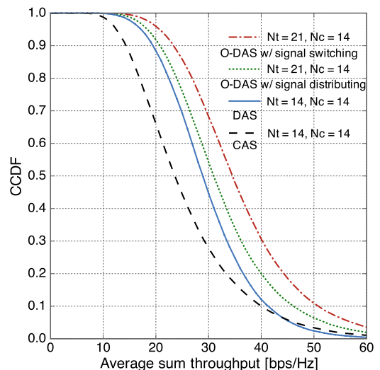
Fig. 9 CCDF of average sum throughput ( N_c=14 ).
