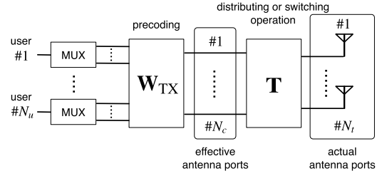
Fig. 7 Transmitter structure.
