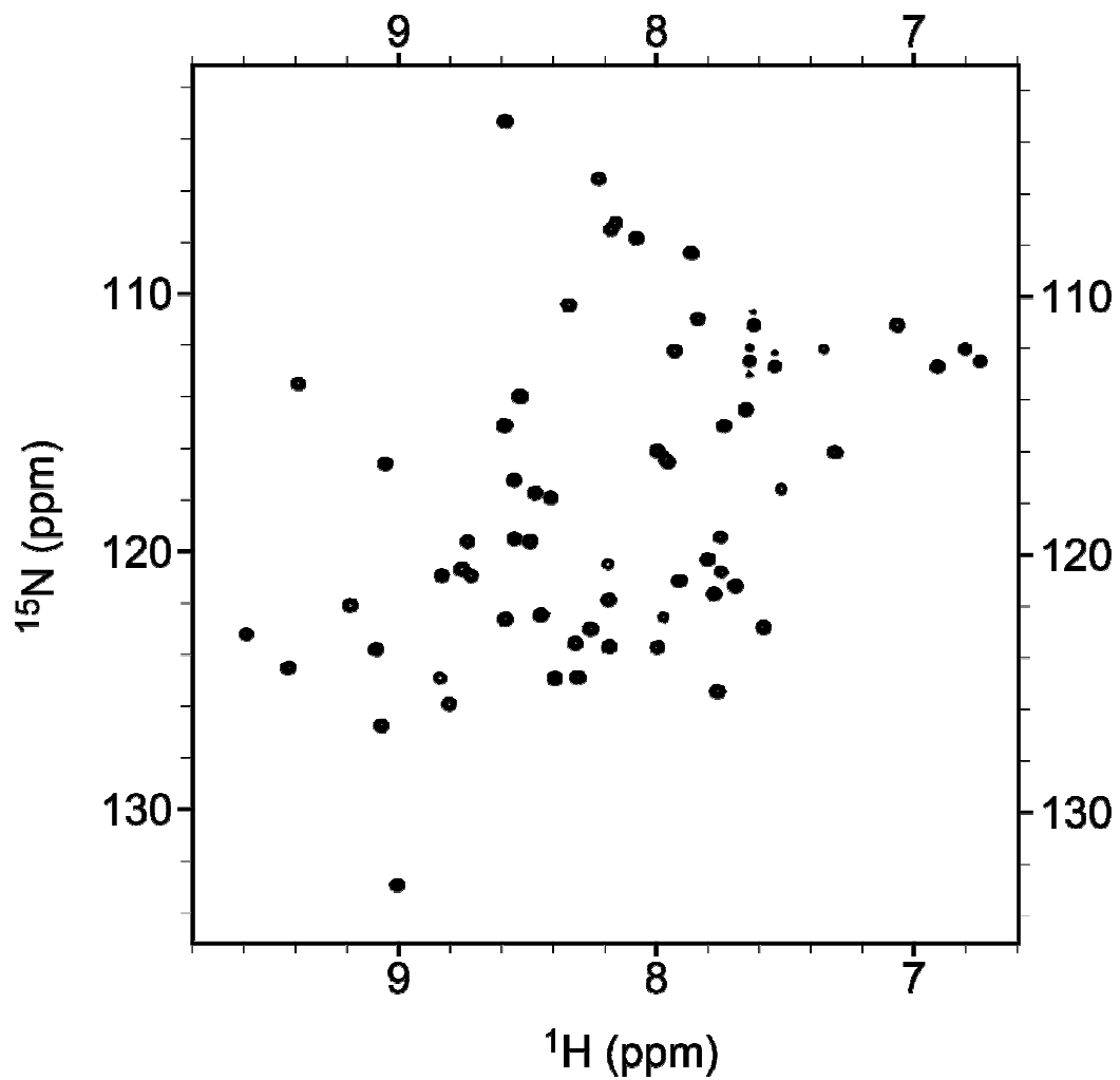
Figure 5. ^1\text{H} - ^{15}\text{N} HSQC spectrum of 0.7 mM ^{15}\text{N} -labeled ABF-2 in 20 mM phosphate buffer at pH 5.7 and 20 ^{\circ}\text{C} .
