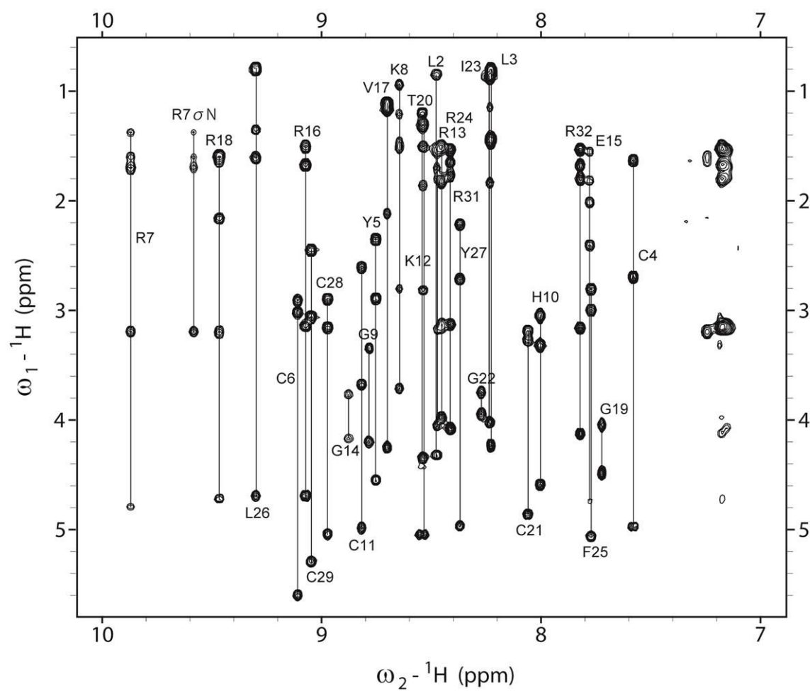
Figure 7. Fingerprint region of the 2D TOCSY spectrum of Crp4.
