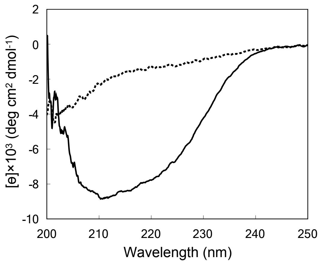
Figure 4. Circular dichroism spectra of correctly folded (solid line) and misfolded (dotted line) ABF-2.
