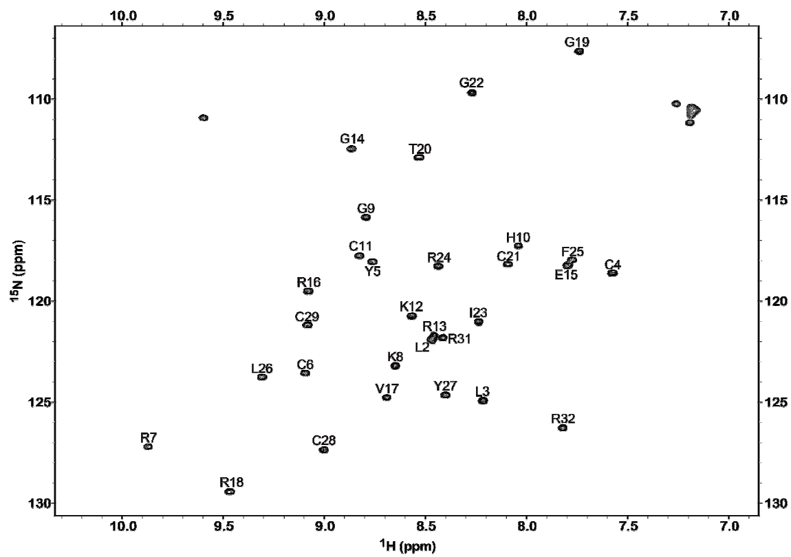
Figure 8. ^1\text{H} - ^{15}\text{N} HSQC spectrum of 0.5 mM ^{15}\text{N} -labeled Crp4.
