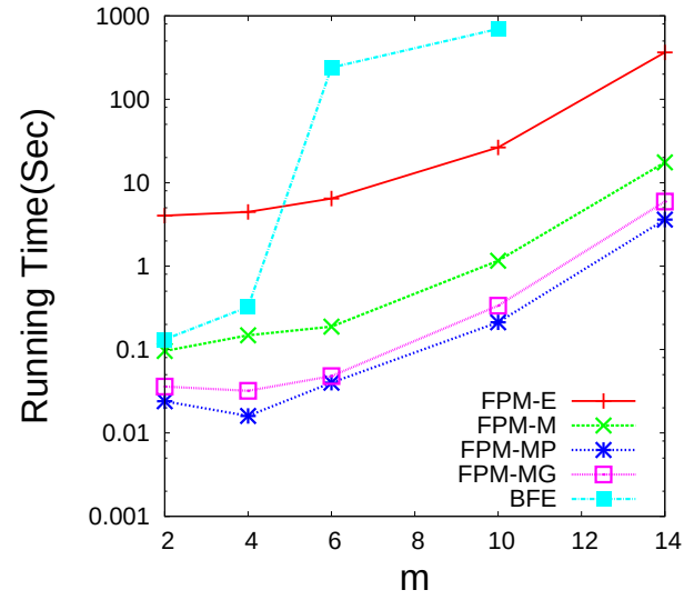
Figure 4.4: Exp 3: Running time varying the true and mining pattern widths r_* and r with r = r_* .
