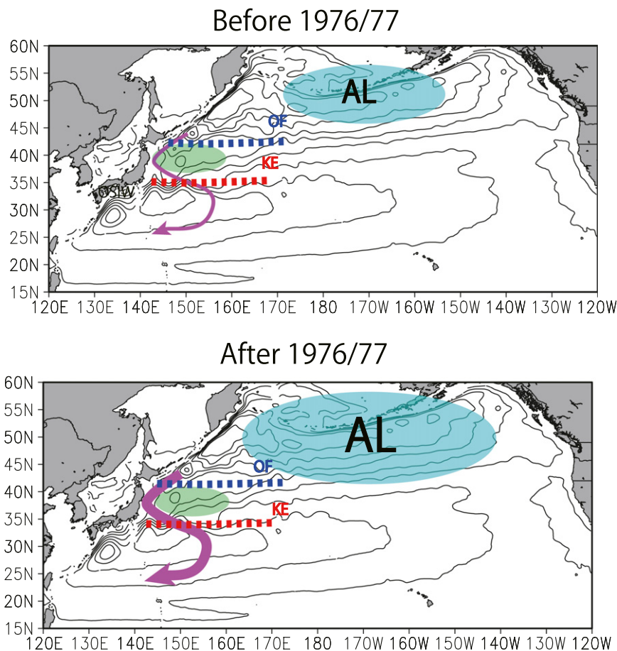
FIG. 15. Schematic of the freshening processes at the salinity minimum density of NPIW, driven by the 1976/77 regime shift in the wind stress.
