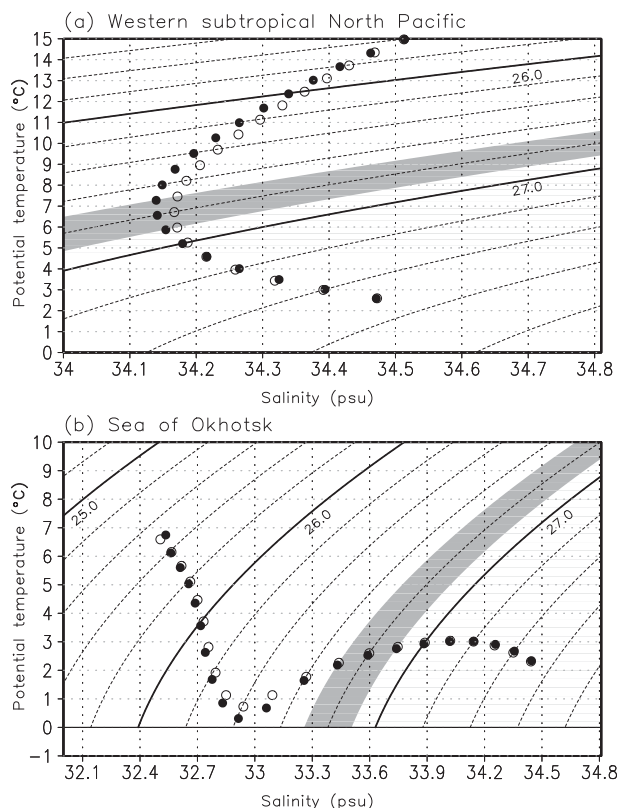
FIG. 5. As in Fig. 4, but for the simulated data.
