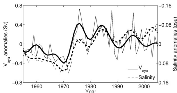
FIG. 9. Time series of annually averaged V_{\text{oya}} in the rectangular region shown in Fig. 8c (solid line) and salinity anomalies in the MWR ( 40^{\circ} – 44^{\circ} N, 145^{\circ} – 150^{\circ} E) at 26.8 \sigma_{\theta} (dashed line). The positive anomaly of V_{\text{oya}} means that the southward transport of the Oyashio is strengthened relative to the climatological value. The term V_{\text{oya}} at 26.8 \sigma_{\theta} is calculated from the meridional velocity and layer thickness defined as the distance between \pm 0.05 \sigma_{\theta} at the corresponding isopycnal surface, as defined by Eq. (1). Thick lines denote 7-yr low-pass filtered data. Note that salinity anomalies are shown on the axis of negative upward.
