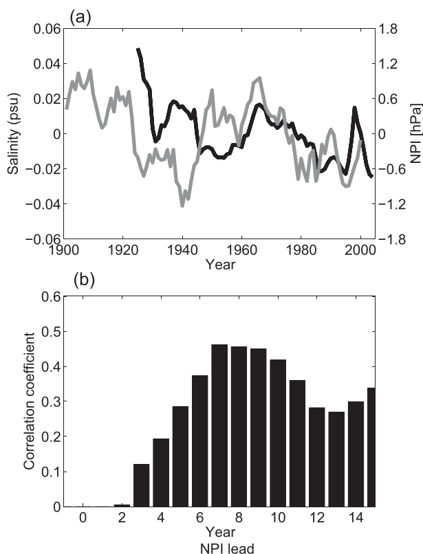
FIG. 14. (a) Time series of the 5-yr running mean of annual-mean salinity anomalies at 26.8 \sigma_\theta averaged over the western subtropical North Pacific (rectangular region denoted by purple lines in Fig. 2a) (black) and NPI anomalies (gray) from December to the following May. The scale of the NPI is indicated on the right axis. (b) Lead-lag correlations between the 5-yr running mean of salinity at 26.8 \sigma_\theta and the NPI from 1925 to 2004.
