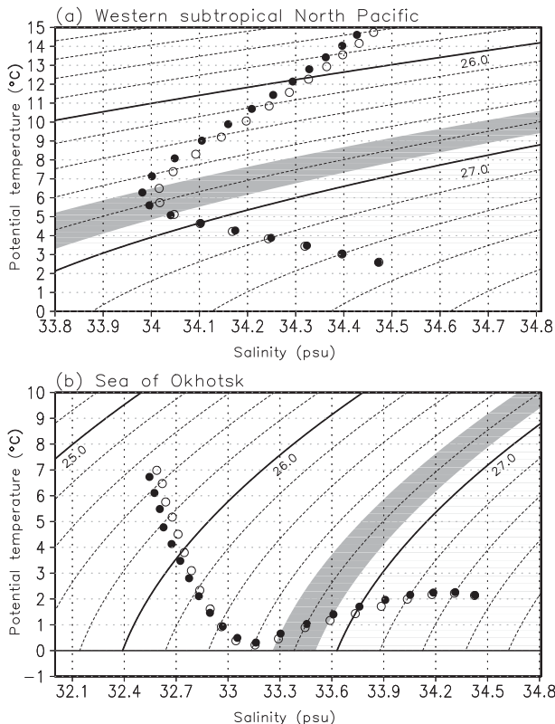
FIG. 4. Time variations of the observed T - S curve averaged over (a) the western subtropical North Pacific and (b) the Sea of Okhotsk (rectangular regions denoted by purple and green lines in Fig. 2a). Open (closed) circles denote the past (1955–76) and present (1977–2004) values on isopycnal surfaces. The shading indicates the density range of the salinity minimum core from 26.7 to 26.9 \sigma_\theta .
