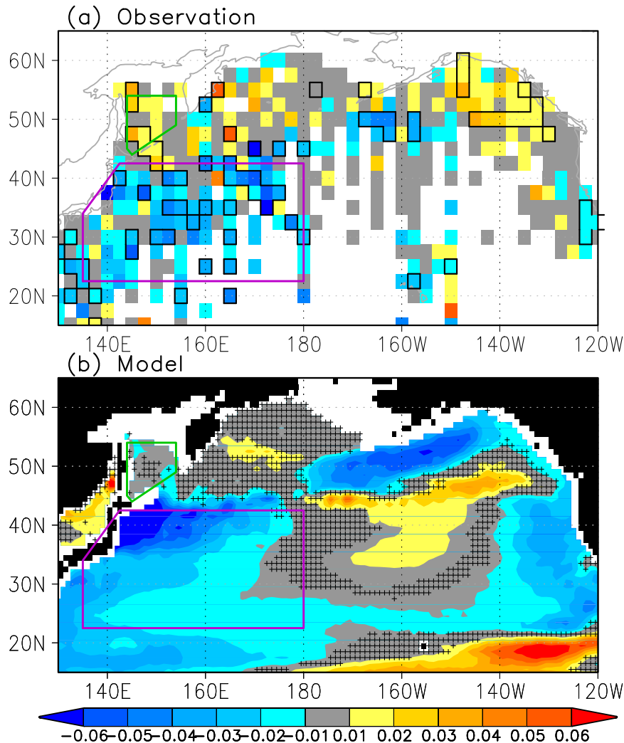
FIG. 2. Spatial pattern of change in the annually averaged salinity from 1955–76 to 1977–2004 at 26.8 \sigma_\theta for (top) the observations and (bottom) the model simulation. The colors indicate the amplitude of the difference. Negative values indicate that potential temperature decreased from 1955–76 to 1977–2004. (a) The black grid box boundary indicates a region where the difference is significant at the 95% confidence level. In (a), the grid boxes where yearly temperature anomalies are not available for more than 5 yr in each period are not used for the analysis. (b) The region for insignificant difference is marked by the cross hatching. The statistical significance of the difference is based on a Student's t test distribution with 1 degree of freedom \text{yr}^{-1} . The boundaries of the western subtropical region (purple) and the Sea of Okhotsk (green), for which area-averaged quantities are displayed in Fig. 3, are indicated.
