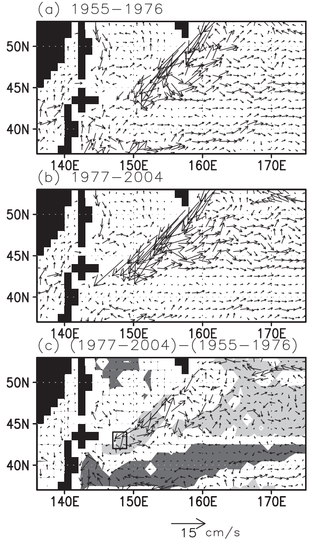
FIG. 8. The mean state of annually averaged current velocity ( \text{cm s}^{-1} ) at 26.8 \sigma_\theta from the model simulation: (a) 1955–76, (b) 1977–2004, and (c) the difference of the mean state between the latter (1977–2004) and former (1955–76) periods. In (c), the dense and light shades indicate regions where the negative and positive difference of the absolute current speed is significant at the 95% confidence level, respectively. For the calculation of the significance, we assume that each year is independent.
