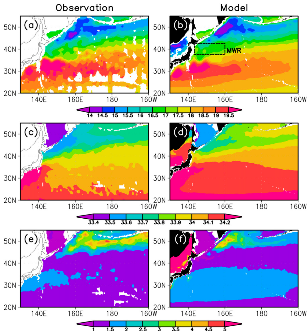
FIG. 1. Climatologies of (a),(b) acceleration potential, (c),(d) salinity, and (e),(f) PV at 26.8 \sigma_\theta for (left) the observations and (right) the model simulation. The contour interval is (top) 0.5 \text{ m}^2 \text{ s}^{-2} , (middle) 0.1 \text{ psu} , and (bottom) 0.5 \times 10^{-10} \text{ m}^{-1} \text{ s}^{-1} . The acceleration potential is calculated relative to 2000 dbar. In (b), the region for the MWR (broken line) is indicated.
