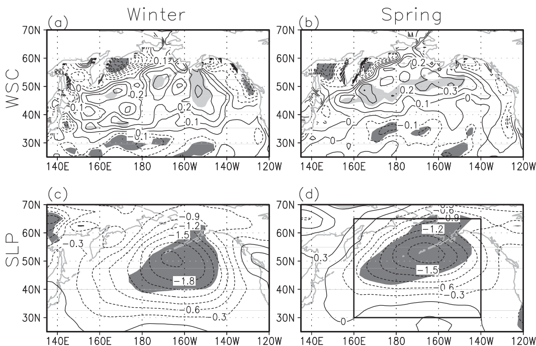
FIG. 13. Regression maps of annually averaged (a), (b) wind stress curl and (c), (d) sea level pressure in (left) winter and (right) spring onto the normalized time series of annually averaged V_{\text{oya}} at 26.8 \sigma_\theta with a 7-yr low-pass filter. In the left and right panels, V_{\text{oya}} leads the wind stress curl and sea level pressure fields by 0 and 3 yr. The contour interval is (top) 0.1 \times 10^{-7} \text{ N m}^{-3} and (bottom) 0.3 hPa. The light and heavy shades indicate regions where the positive and negative correlation is significant at the 90% confidence level, respectively. In (d), the boundary for the calculation of NPI is indicated.
