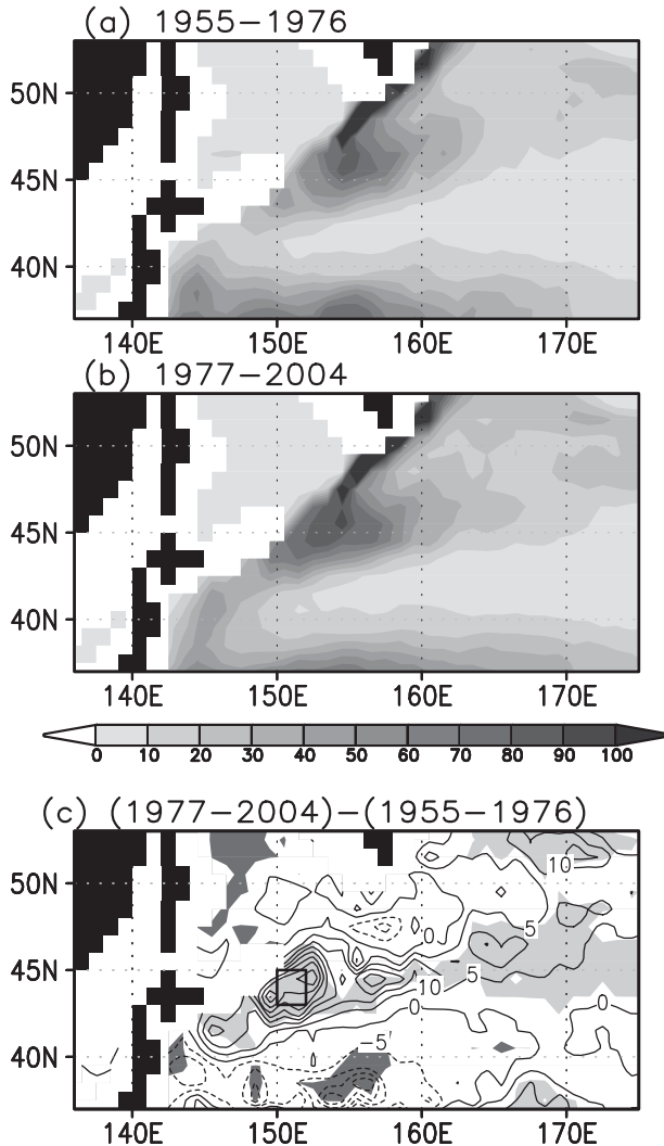
FIG. 10. The mean state of annually averaged EKE ( \text{cm}^2 \text{s}^{-2} ) at 26.8 \sigma_\theta from the model simulation: (a) 1955–76, (b) 1977–2004, and (c) the difference of the mean state between the latter (1977–2004) and former (1955–76) periods. In (c), the light and dense shades indicate regions where the positive and negative difference is significant at the 95% confidence level, respectively. For calculation of the significance, we assume each year is independent.
