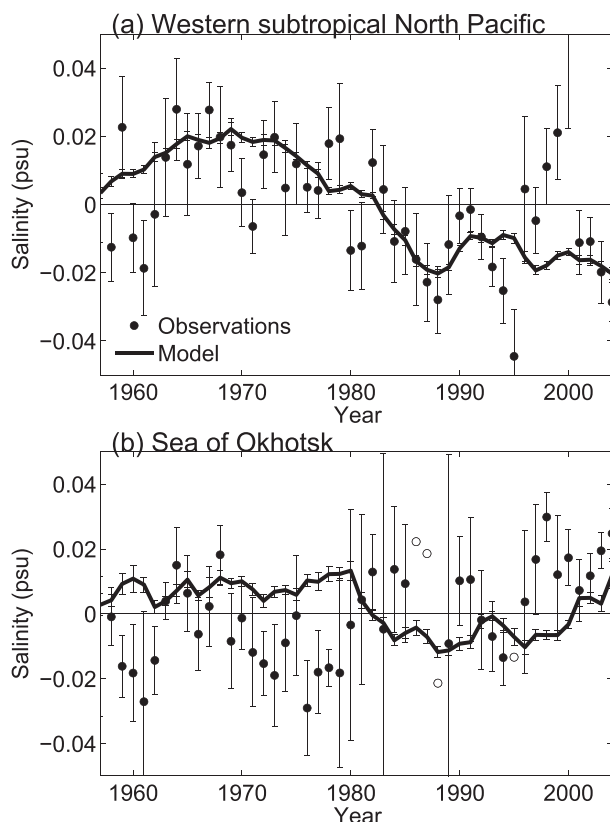
FIG. 3. Time series of annual-mean salinity anomalies at 26.8 \sigma_\theta averaged over (a) the western subtropical North Pacific and (b) the Sea of Okhotsk (rectangular regions denoted by purple and green lines in Fig. 2a) for observations (circles) and model (solid line). A vertical line represents a \pm 1 standard error of the annual mean of the observation. In (b), open circles indicate the anomalies for the area, in which the number of the data is very small.
