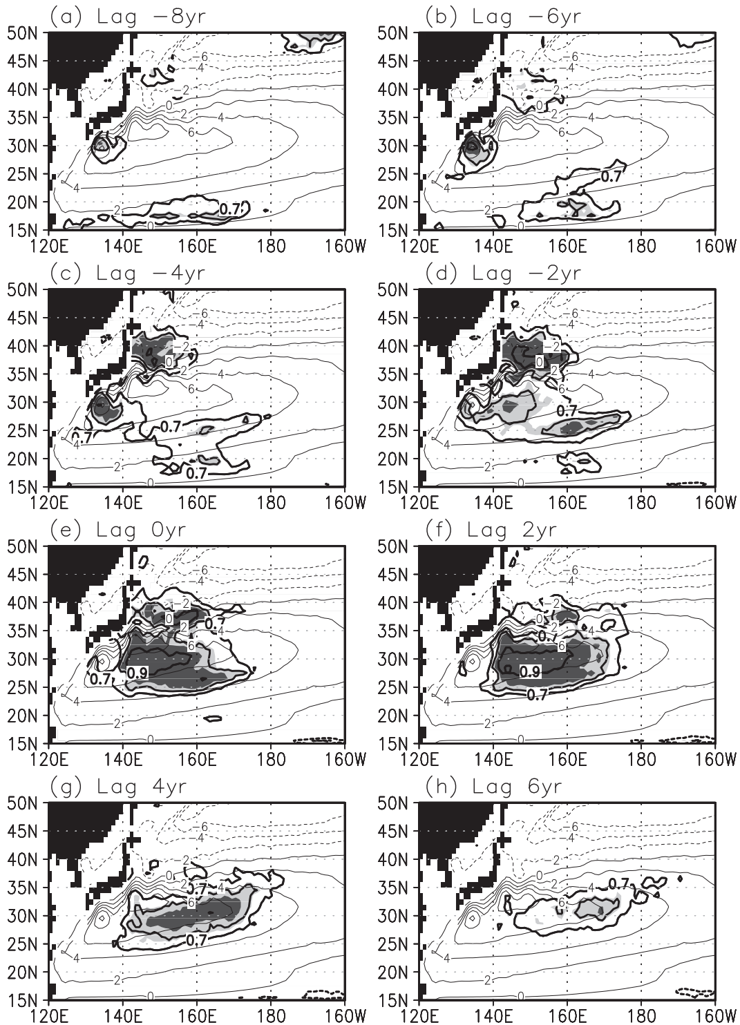
FIG. 6. Lead-lag correlation maps (thick contours) of 7-yr low-pass filtered annually averaged salinity at 26.8 \sigma_\theta , with the time series averaged over the subtropical recirculation gyre ( 22.5^\circ\text{--}37.5^\circ\text{N} , 135^\circ\text{--}170^\circ\text{E} ) at lags (a) -8 , (b) -6 , (c) -4 , (d) -2 , (e) 0 , (f) +2 , (g) +4 , and (h) +6 yr. The contour interval is 0.1 , and values less than 0.7 are omitted. The light and heavy shadings indicate the regions where the absolute value of the correlation is significant at the 90\% and 95\% confidence level, respectively. The climatology of annual-mean pressure (kPa) at 26.8 \sigma_\theta (thin contours) is superimposed on each panel.
