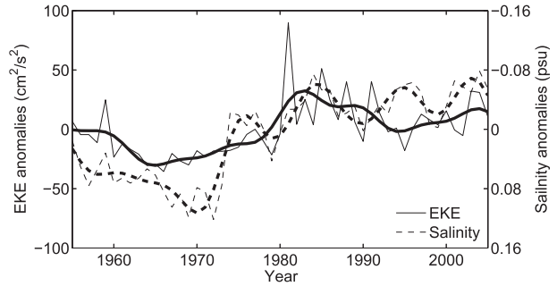
FIG. 11. The time series of annually averaged EKE anomalies in the rectangular region near the subarctic front shown in Fig. 10c (solid line) and salinity anomalies in the MWR ( 40^\circ\text{--}44^\circ\text{N} , 145^\circ\text{--}150^\circ\text{E} ) at 26.8 \sigma_\theta , as in Fig. 9. Thick lines denote 7-yr low-pass filtered data.
