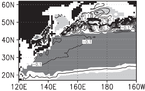
FIG. 7. Change in the annually averaged PV at 26.8 \sigma_\theta from 1955–76 to 1977–2004 for the model simulation. The contour interval is 0.05 \times 10^{-10} \text{ m}^{-1} \text{ s}^{-1} . Negative values indicate that PV decreased from 1955–76 to 1977–2004. The light (heavy) shading indicates the region where the positive (negative) difference is significant at the 95% confidence level.
