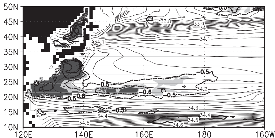
FIG. 12. Correlation maps (thick contours) of 7-yr low-pass filtered annually averaged salinity at 26.8 \sigma_\theta , with the recirculation gyre index. The contour interval is 0.1 and values less than 0.5 are omitted. The light and heavy shades indicate regions where the absolute value of the correlation is significant at the 90% and 95% confidence level, respectively. The annual climatology of salinity (thin contours) at 26.8 \sigma_\theta is superimposed.
