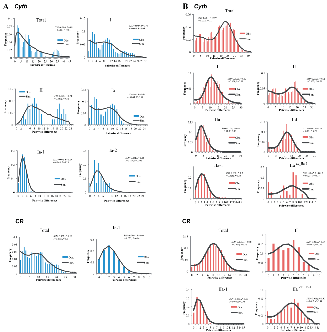
Fig. 5 Mismatch distribution of the mitochondrial cytochrome b ( Cytb ) and control region (CR) sequences for A. argenteus (a) and A. speciosus (b). Bars indicate observed frequency, and a line denotes the expected frequency under the sudden expansion model. SSD, sum of squared deviations; r , Harpending's raggedness index
