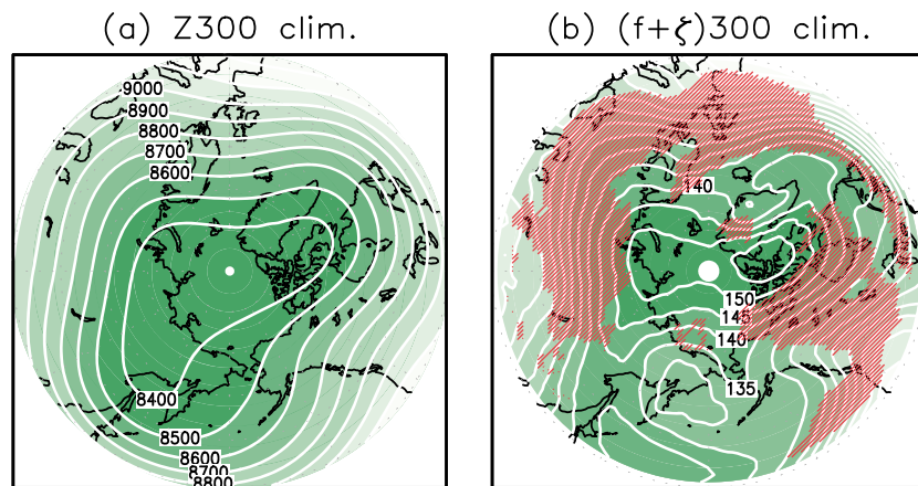
Figure 9. DJF-averaged climatologies of (a) geopotential height (m) and (b) absolute vorticity ( 10^6 \text{ s}^{-1} ) at 300 hPa. The climatology is defined as the 120-year average of the CNTL and N.ICE runs. Meridional gradients of the absolute vorticity exceeding 10^{-8} \text{ s}^{-1} \text{ km}^{-1} are hatched in red in Figure 9b.
