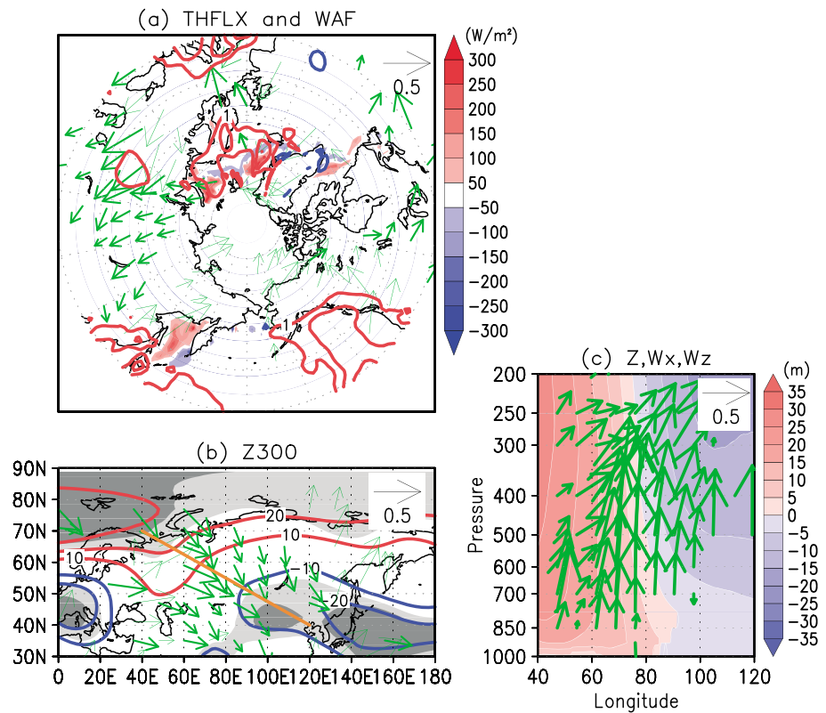
Figure 8. DJF-averaged anomalies of N.ICE with respect to the CNTL run. (a) Shading, contours, and arrows indicate turbulent heat flux ( \text{W m}^{-2} ; i.e., sensible plus latent heat, upward positive), the vertical component of wave activity flux ( 10^{-2} \text{ m}^2 \text{ s}^{-2} ) at 700 hPa, and the horizontal wave activity flux vector ( \text{m}^2 \text{ s}^{-2} ) at 300 hPa, respectively. The arrow length corresponding to 0.5 \text{ m}^2 \text{ s}^{-2} is indicated in the top-right corner of each panel. Note that the horizontal wave activity fluxes in the southward (northward) direction are drawn as thick (thin) arrows. (b) Geopotential height anomalies at 300 hPa. Contours and shading are the same as in Figure 5a. Associated wave activity fluxes are shown by green arrows. (c) Vertical cross-sections of geopotential height anomalies and the zonal and vertical components of wave activity flux along the brown line in (b). The vertical component of the vectors is multiplied by a factor of 600.
