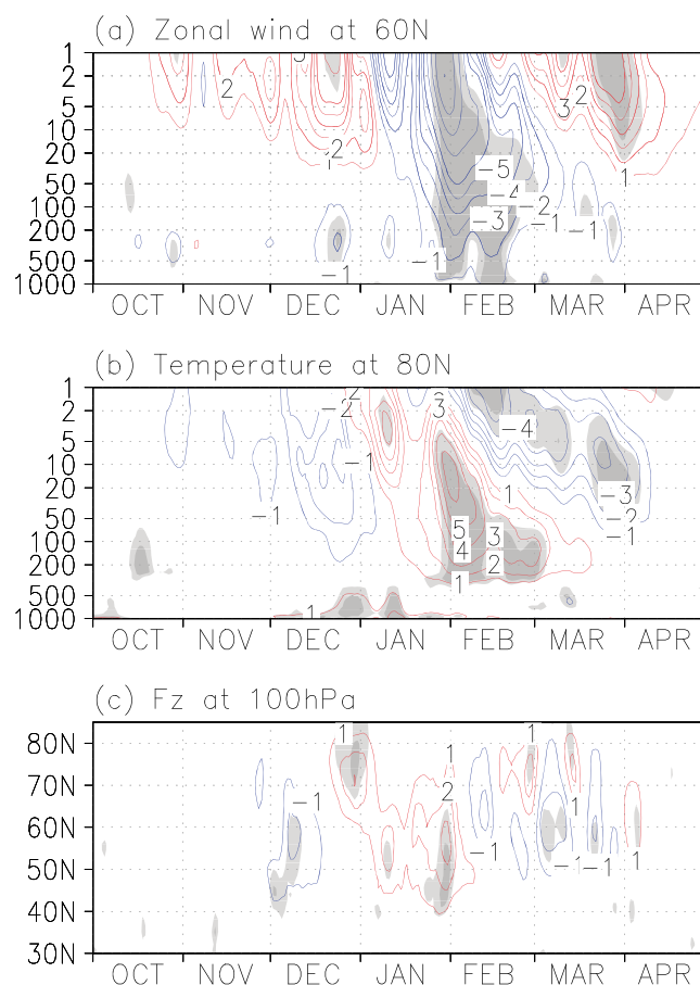
Figure 15. Winter seasonal evolution of anomalies of N_{ICE} with respect to CNTL for (a) zonal mean zonal wind at 60°N ( m s^{-1} ), (b) zonal mean temperature at 80°N (K), and (c) vertical component of EP flux ( 10^4 m^2 s^{-2} ) at 100 hPa. Contour and shading intervals are as in Figure 5a.
