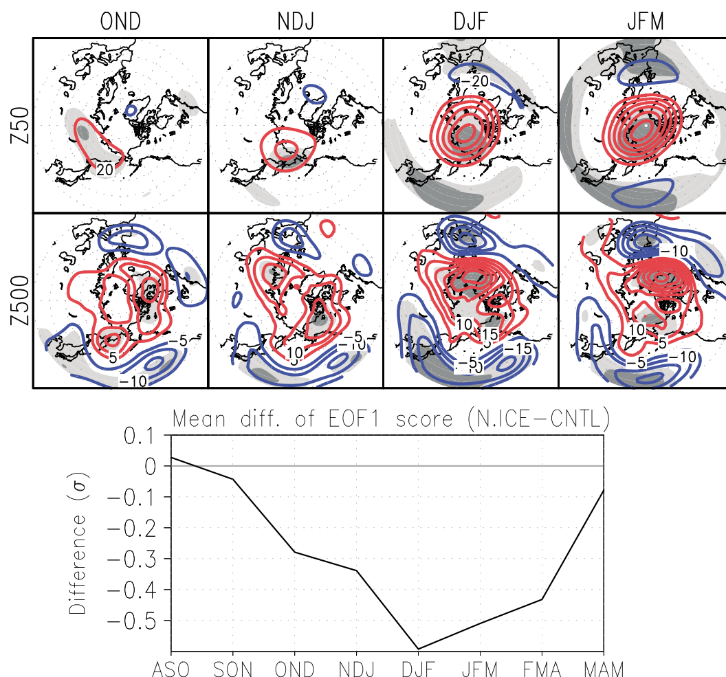
Figure 14. (Top) Geopotential height anomalies of N.ICE with respect to CNTL in OND, NDJ, DJF, and JFM at 50 hPa (upper row) and 500 hPa (lower row). Contours and shading intervals are as in Figure 5a. (Bottom) Time series of the mean difference of the EOF1 scores (i.e., N.ICE minus CNTL ).
