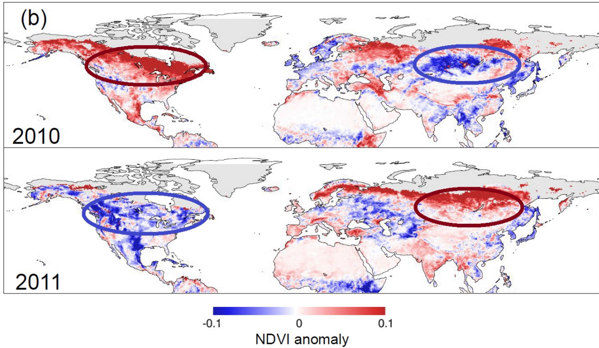
Figure 4.6. Distributions of spring (an average of April–May) (a) air temperature (NCEP/NCAR reanalysis data (Kalnay et al., 1996)) and (b) MODIS NDVI anomalies in the Northern Hemisphere for base period of 2009–2011. For NDVI anomaly, pixels corresponding to LST values of <0^{\circ}\text{C} were disregarded (gray shading) in order to eliminate unrealistically high NDVI values due to snow cover.
