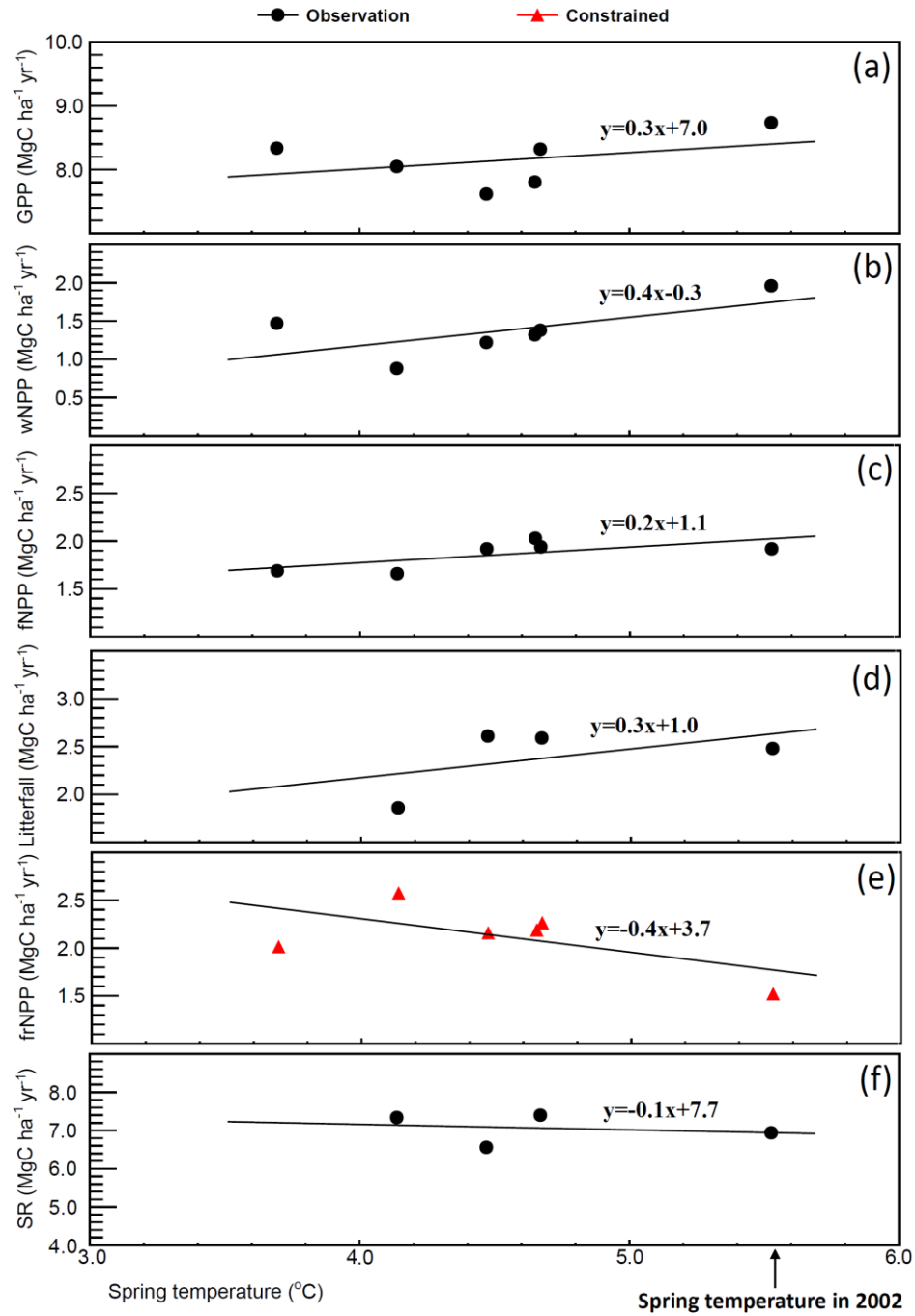
Figure 3.6. Relationships between the spring temperatures (March–May) and annual carbon fluxes: (a) GPP, (b) wNPP, (c) fNPP, (d) litterfall, (e) frNPP (constrained simulation), and (f) SR.
