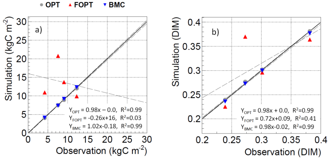
Figure 2.3. Scatter plots of (a) the modeled and observed total biomasses and (b) below- to above-ground biomass ratio. For each site, the inventory data were compared with the model outputs. For simplicity, it was assumed that the ecosystem in each study site possessed the observed biomasses in the first year of flux observation (2001 for TMK, TKY, and FJY and 2004 for LSH). The model results are shown for three different optimization schemes, OPT, FOPT, and BMC.
