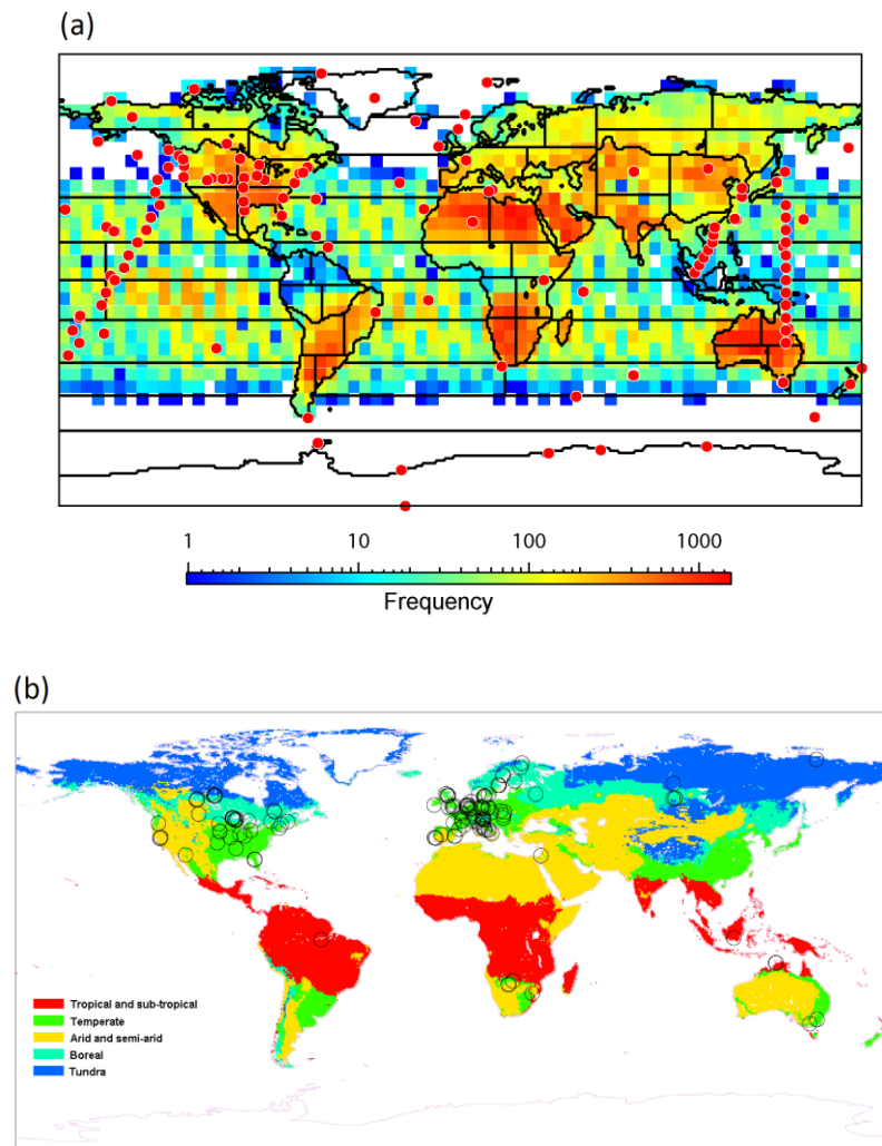
Figure 4.11. (a) Number of GOSAT Level 2 XCO 2 data per each 5^\circ \times 5^\circ grid cell over the analyzed period (29 months from Jun 2009–Oct 2011). The overlaid red circles indicate the locations of GV sites chosen for this study (212 sites). Solid line indicates boundaries of the 64 source regions. (b) Global site distribution of FLUXNET data (144 sites) used for the construction of the SVR models. Site
