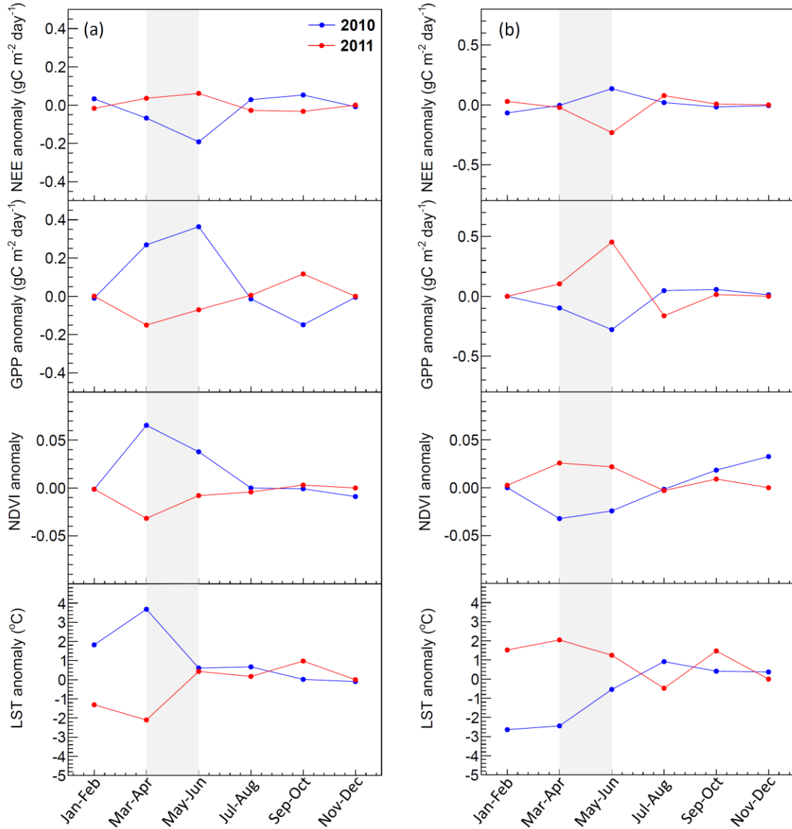
Figure 4.8. Two-monthly average seasonal variations of the SVR biosphere flux, SVR-based GPP, MODIS NDVI, and daytime LST in (a) North America (region IDs: 1, 2, and 8) and (b) boreal Eurasia (region ID 25). Anomalies refer to base period of 2010–2011.
