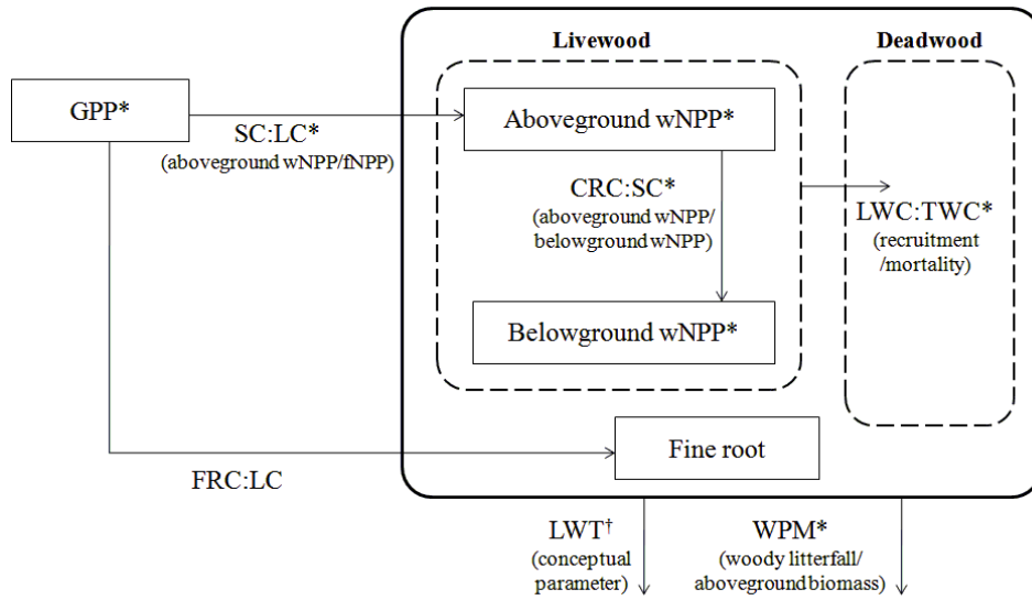
Figure 3.2. A simple schematic of carbon flow in the Biome-BGC model, illustrating carbon fluxes and parameters constrained in the present study. Abbreviations of model parameters: StemC:LeafC (SC:LC), FrootC:LeafC (FRC:LC), CrootC:StemC (CRC:SC), LivewoodC:TotalwoodC (LWC:TWC), live-wood turnover rate (LWT), and whole-plant mortality (WPM). *Observed values are available to constrain components. †Values for components can be conceptually fixed.
