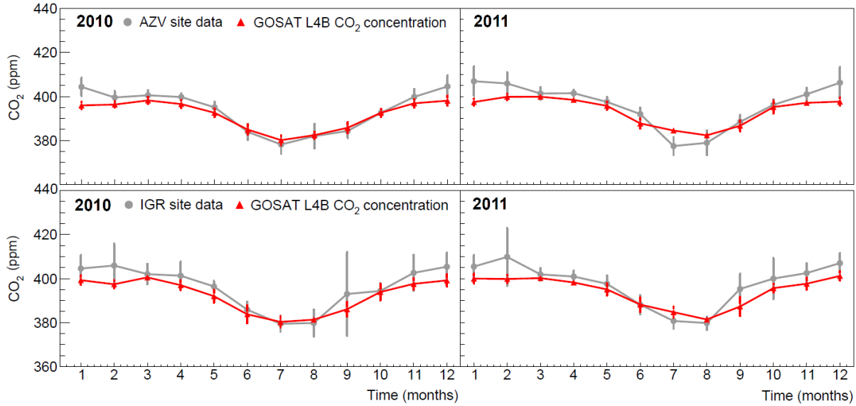
Figure 4.10. Temporal variations of monthly mean of daytime CO 2 concentrations (13:00-17:00 LST) from two Siberian tower observations (AZV and IGR sites) and GOSAT L4B in 2010 and 2011.
