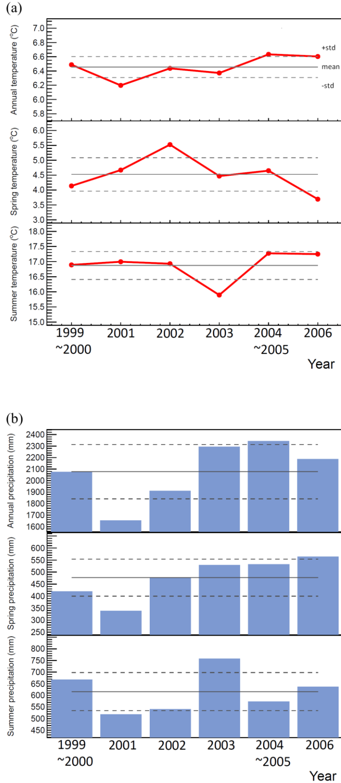
Figure 3.1. Interannual variations in the annual, spring (March–May), and summer (June–August) (a) temperature (°C), (b) precipitation amount (mm), and (c) PPFD ( \text{W m}^{-2} ) observed from 1999 to 2006 at the Takayama site. Temporal coverage was set to the same as that of inventory measurements from Ohtsuka et al., (2009).
