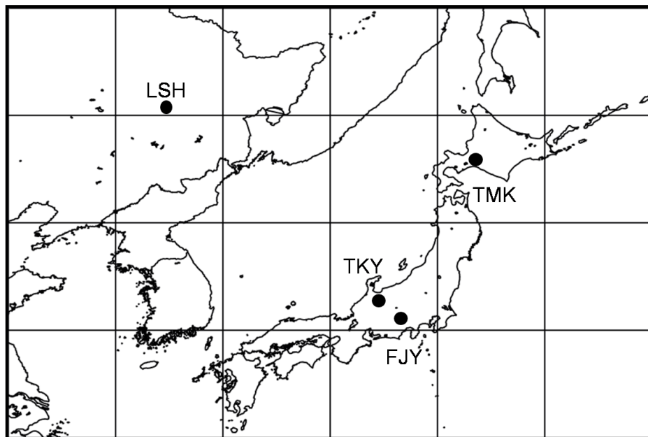
Figure 2.1. Locations of the four eddy flux observation sites used in this study.
