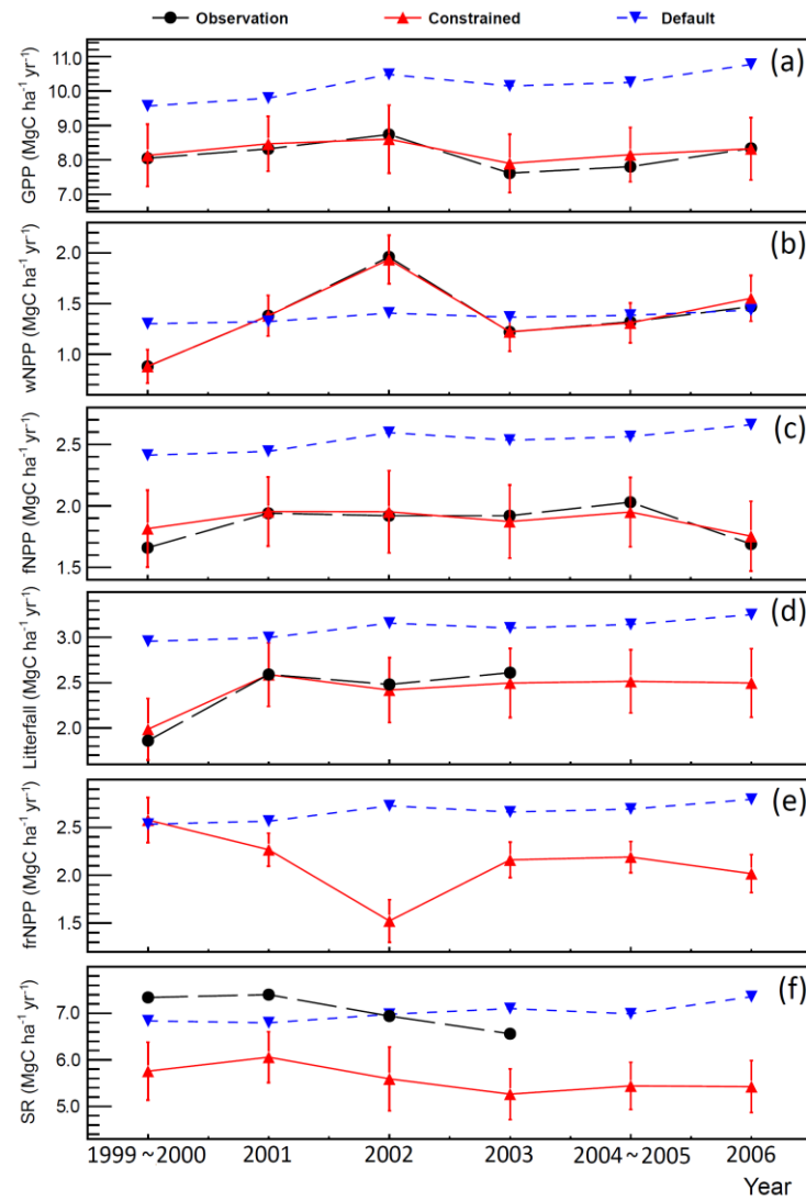
Figure 3.3. Interannual variations in observed and modeled (the constrained and default simulations) carbon fluxes ( \text{MgC ha}^{-1} \text{ yr}^{-1} ). (a) GPP (80% of the actual value), (b) wNPP, (c) fNPP, (d) litterfall (sum
