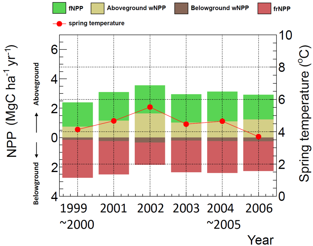
Figure 3.7. Interannual variations in the aboveground NPP (fNPP and aboveground wNPP), belowground NPP (belowground wNPP and frNPP), and spring temperatures (March–May).
