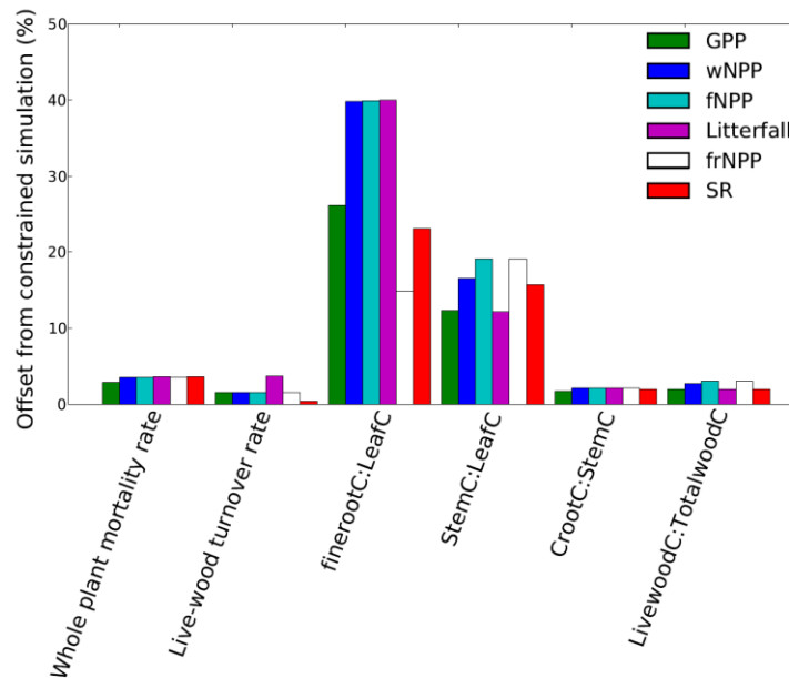
Figure 3.4. Model parameter sensitivity to annual GPP, wNPP, fNPP, litterfall, frNPP, and SR. For \pm 30\% range from the constrained parameter value, deviations from the constrained simulation (deviation (%) = |(\text{constrained flux} - x) / \text{constrained flux}| , for x being simulation with varied parameter values) were calculated for each parameter. The averages of the maximum deviation from 1999 to 2006 are shown here.
