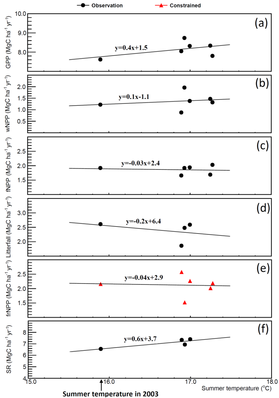
Figure 3.5. Relationships between the summer temperatures (June–August) and annual carbon fluxes: (a) GPP, (b) wNPP, (c) fNPP, (d) litterfall, (e) frNPP (constrained simulation), and (f) SR.
