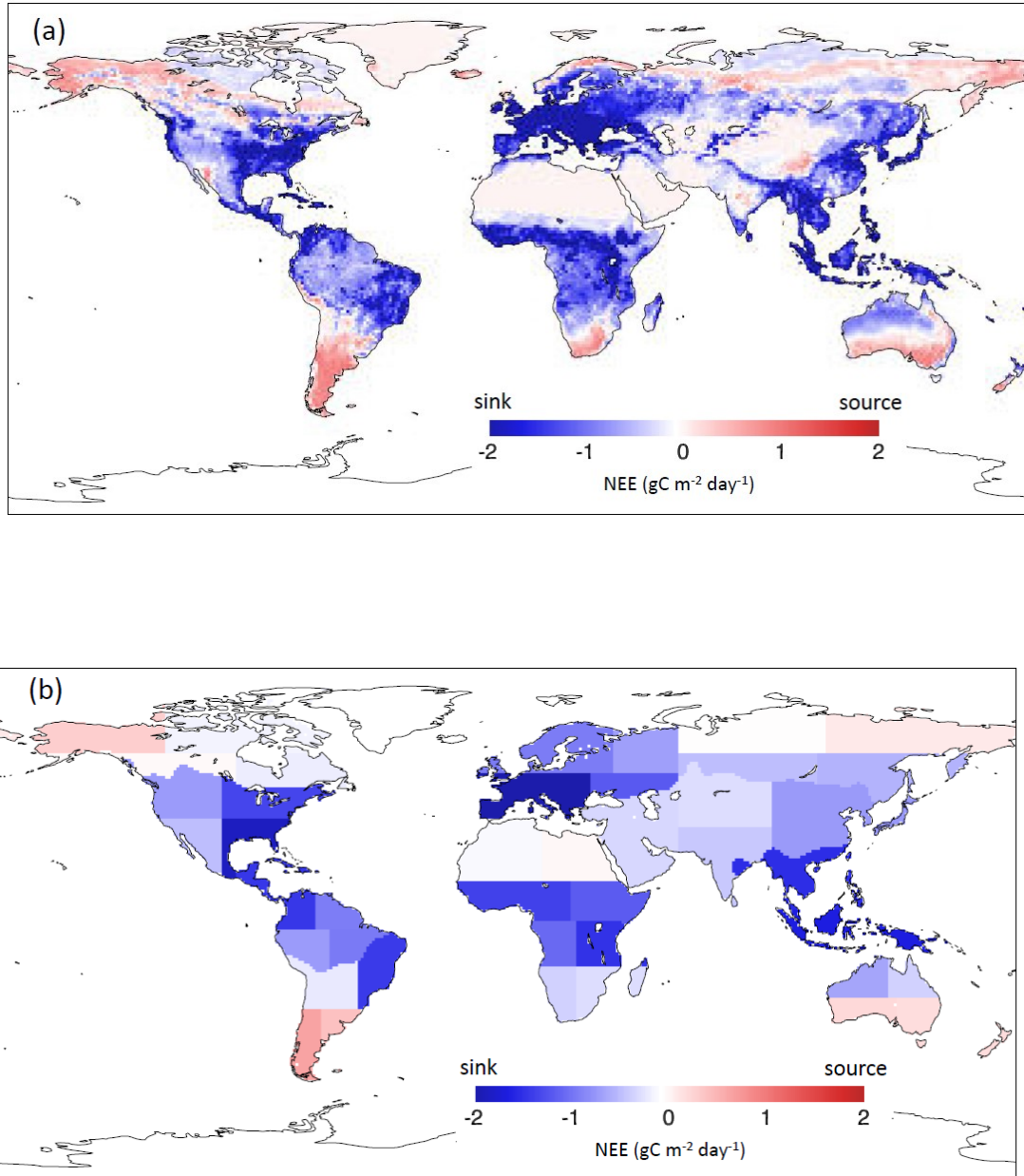
Figure 4.3. SVR-based global NEE on June 2009 with (a) the original 0.25^\circ \times 0.25^\circ resolution and (b) tile average configuration.
