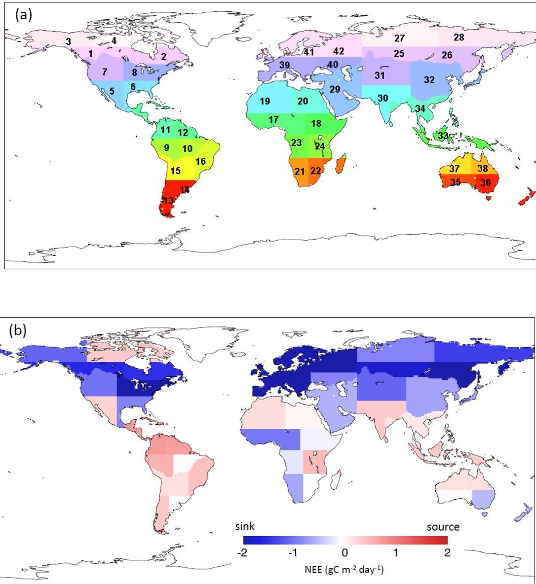
Figure 4.1. (a) Terrestrial region ID of GOSAT L4A and (b) global GOSAT biosphere flux on June 2009.
