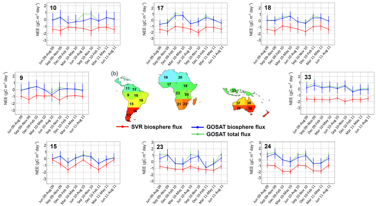
Figure 4.4. Three-monthly average seasonal variations of regional NEEs from the bottom-up (SVR) and top-down (GOSAT biosphere flux) approaches. The eight regional NEEs were each selected from (a) boreal and temperate regions (region IDs: 3, 7, 8, 25, 28, 32, 29, and 41) and (b) sub-tropical and tropical regions (region IDs: 9, 10, 15, 17, 18, 23, 24, and 33).
