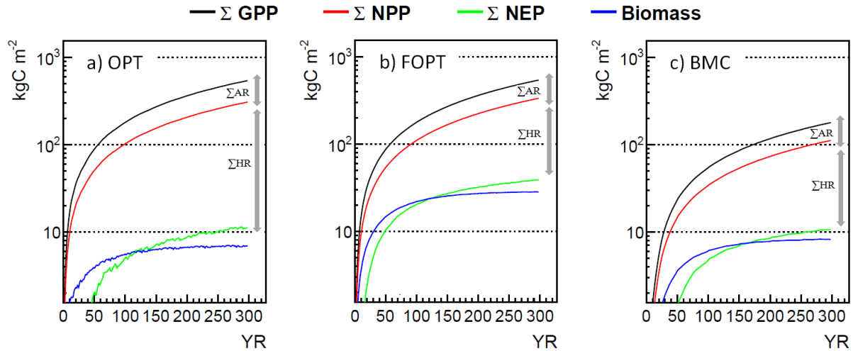
Figure 2.4 Carbon partition plots for simulation with three optimization schemes at the TMK site: (a) OPT, (b) FOPT, and (c) BMC. The cumulative GPP, NPP, NEP, and biomass are shown. The offsets between the cumulative GPP and NPP and cumulative NPP and NEP indicate the cumulative AR and HR, respectively. All the cumulative components were normalized such that the initial points start from zero; thus, the figures represent the carbon partitioning after the occurrence of disturbance events.
