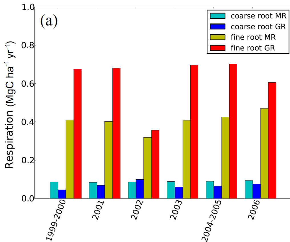
Figure 3.8. Constrained simulation results for (a) fine root and coarse root maintenance respiration (MR) and growth respiration (GR), and (b) fine root and coarse root autotrophic respiration (AR), heterotrophic respiration (HR), and SR.
