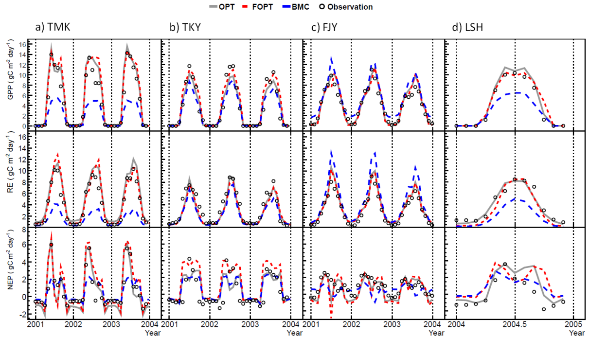
Figure 2.2. Seasonal variations of modeled and observed GPP, RE, and NEP at four eddy flux sites. The results of the three different optimization schemes are shown in different line colors: optimization to both carbon flux and biomass (OPT) (gray) and optimization only to carbon flux (FOPT) (red) and only to biomass (BMC) (blue). The observations are plotted with open circles.
