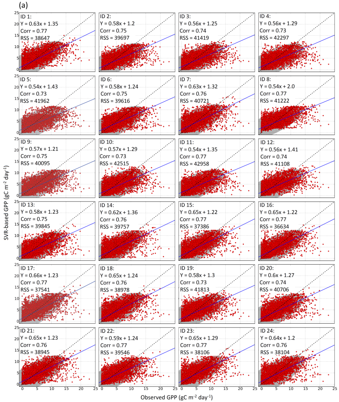
Figure 4.2. Validation of (a) GPP and (b) NEE estimated by the 24 SVR models at the FLUXNET sites. The results from the 24 models constructed from combinations of 10 inputs (SRAD, daytime LST, daily LST, EVI, NDVI, LAI, FPAR, GR43, NDVI43, and EVI43) are shown with regression, Pearson coefficient (Corr., p < 0.01 ), residual sum of squares (RSS), and 95% confidence ellipse.
