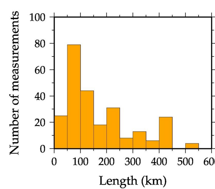
Fig.4 a. Rose diagram showing the number of azimuth alignment of frontal structures observed during 2010. In most cases structures prefer to elongate in the east-west (E-W) direction. Not a single case is observed which has a perfect north-south alignment. b. Histogram showing the number of length observed during 2010. The median length is approximately 100 km.
