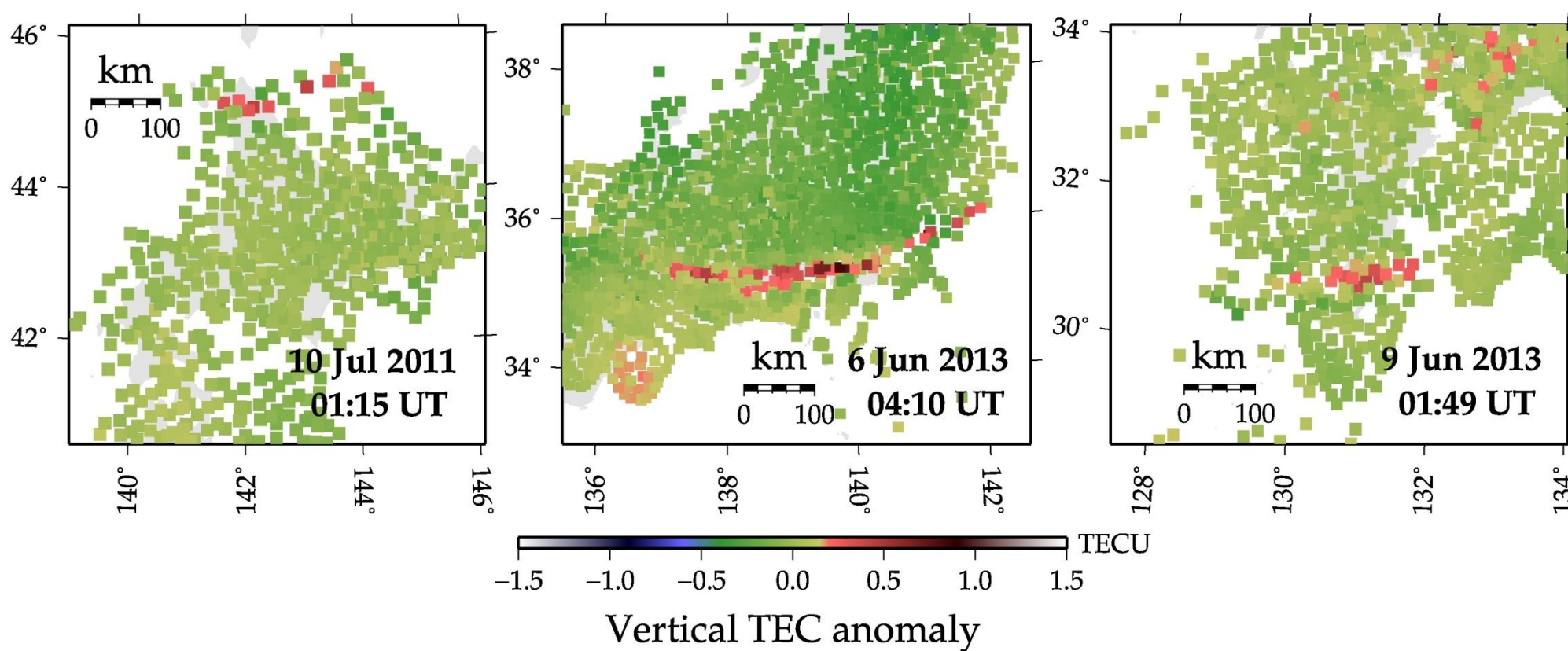
Fig.3 Horizontal shapes of sporadic-E layers observed over a. Wakkanai (45N), b. Kokubunji (35N), and c. Yamagawa (30N). Frontal structures with typical elongation in the east-west (E-W) direction are evident regardless of occurrence latitude. Lengths are in the range of ~50-500 km with an average of ~160 km (Maeda and Heki, EPS , 2015).
