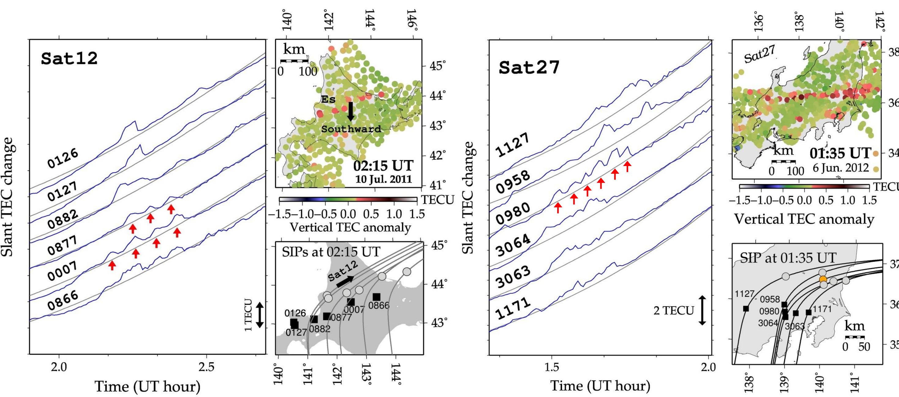
Fig.8 a. Another example of along-elongation QP structure observed over the central part of Japan. b. Vertical TEC anomaly map at 01:35 UT, showing an E-W frontal structure which was stationary during the observation. c. SIP positions with Satellite 27 and six GPS stations at 01:35 UT.
