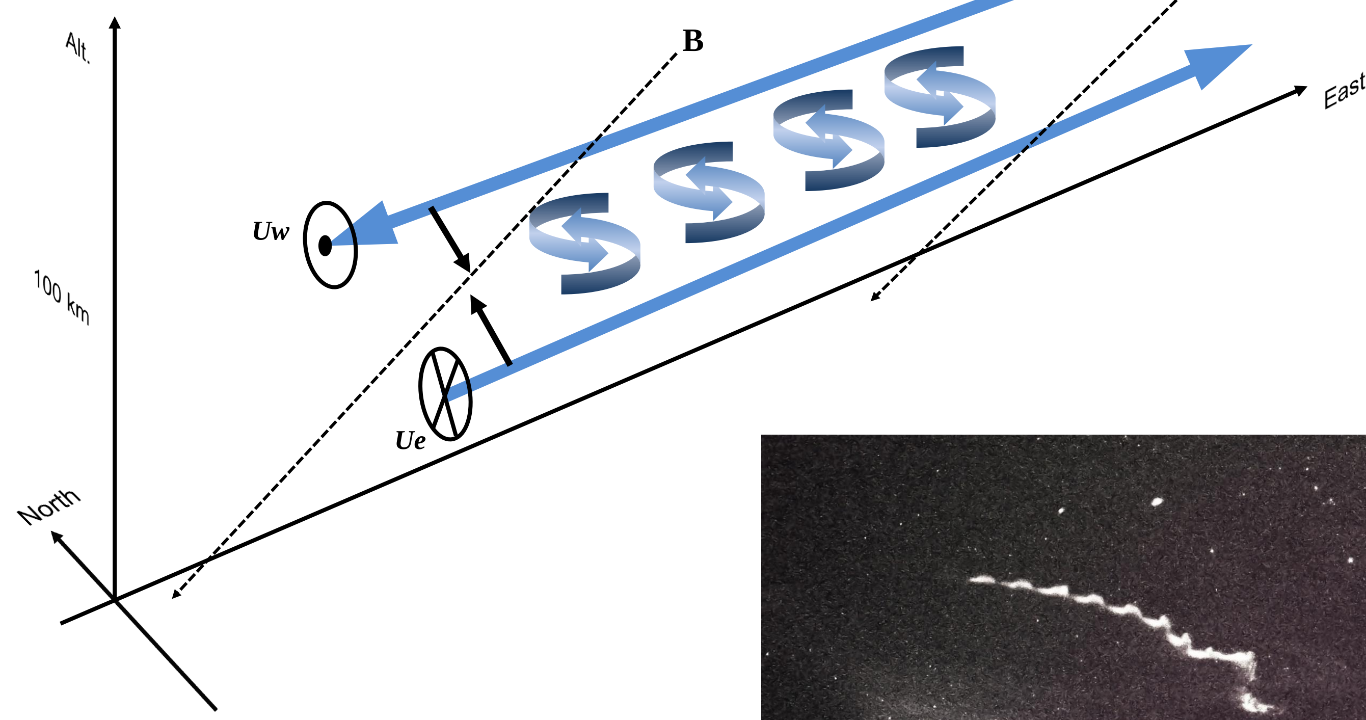
Pictorial image of a TMA trail in the E-region of the ionosphere observed during the SEEK-2 experiment conducted over southwestern Japan [Larsen et al., 2005]
