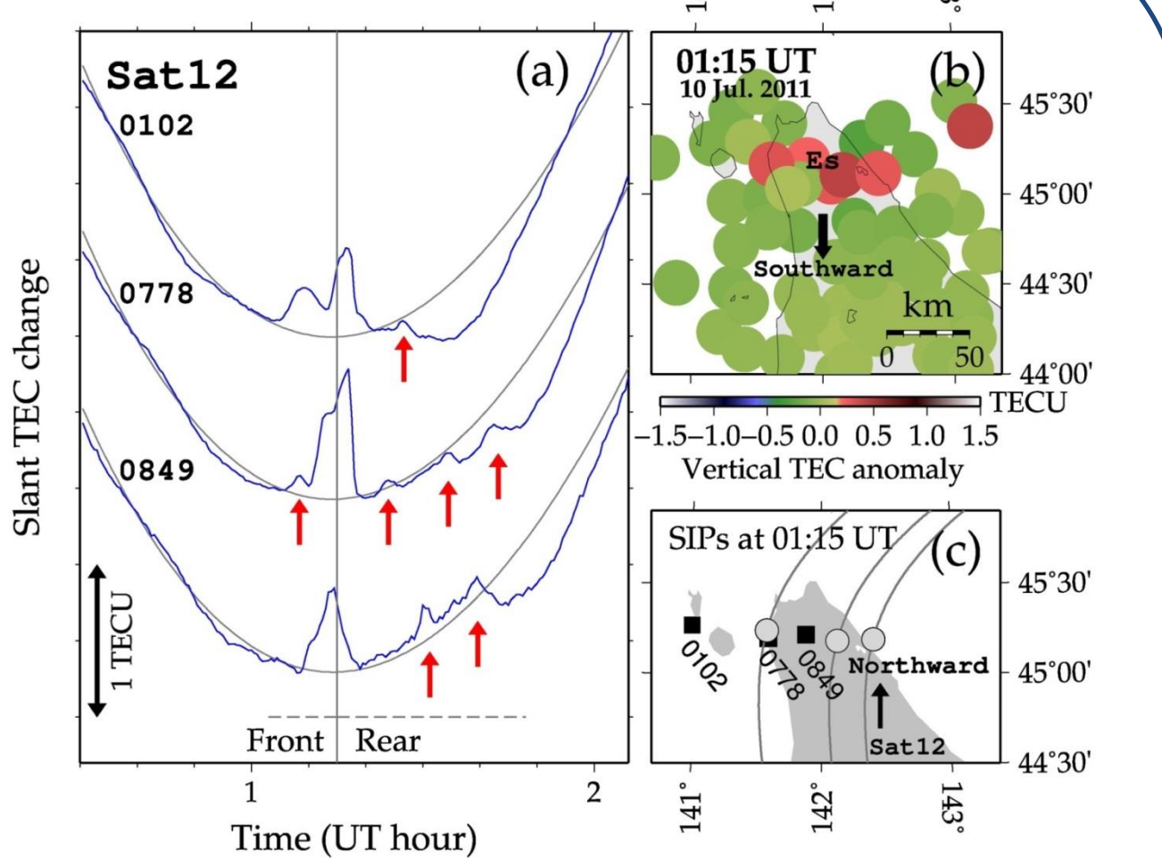
Fig.5 a. Slant TEC time series showing quasi-periodic TEC enhancement. Dominant peaks are accompanied by several small positive peaks. Since the frontal structure moved southward, the time period in the left/right of the vertical gray line at 01:15 UT represents the front/rear side of the structure (shown with horizontal dashed line). b. Vertical TEC anomaly map at 01:15 UT, showing a patchy frontal structure elongated in the E-W direction. c. SIPs of Satellite 12 and three GPS stations at 01:15 UT. Satellite 12 moved northward crossing the frontal structure during the time period shown in a.
