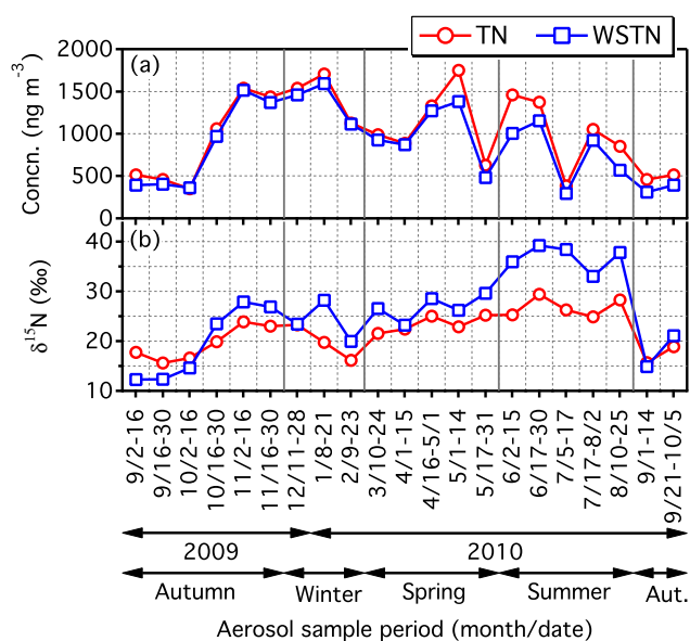
Figure 2. Seasonal variations in (a) concentrations of TN and WSTN and (b) N isotope ratios of TN ( \delta^{15}\text{N}_{\text{TN}} ) and WSTN ( \delta^{15}\text{N}_{\text{WSTN}} ).
