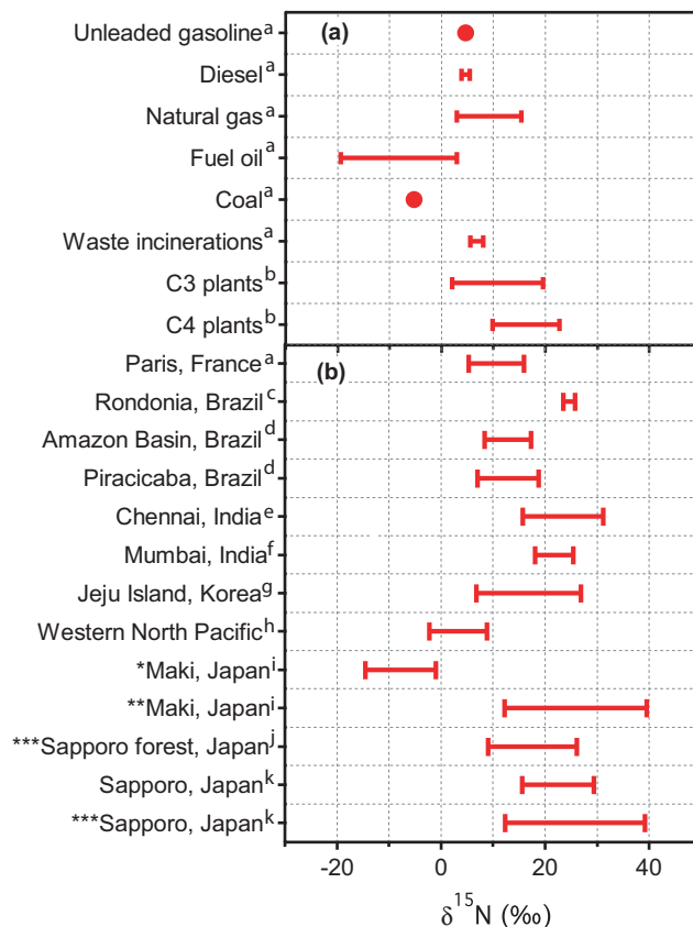
Figure 7. Range or mean N isotope ratios in the particles emitted from point sources, source substance, and atmospheric aerosols from different sites around the world. One, two and three asterisks show gaseous \text{NH}_3 , particulate \text{NH}_4^+ and WSTN, respectively. a Widory (2007); b Turekian et al. (1998); c–g Kundu et al. (2010a, b); d Martinelli et al. (2002); e Pavuluri et al. (2010); f Aggarwal et al. (2013); h,j Miyazaki et al. (2011, 2014); i Hayasaka et al. (2004); k This study.
