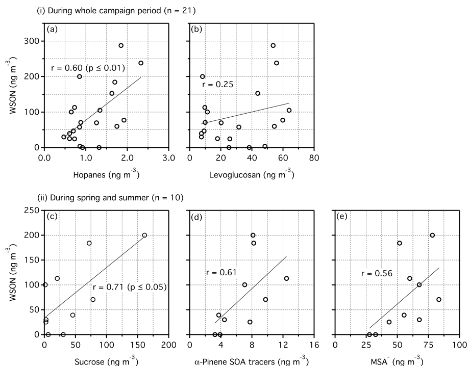
Figure 5. Linear relations of WSON with (a) hopanes (C 27 –C 32 hopanoid hydrocarbons) and (b) levoglucosan during the campaign period ( n = 21 ) and with (c) sucrose, (d) \alpha -pinene-SOA tracers (sum of 3-hydroxyglutaric, pinonic, pinic and 3-methyl-1,2,3-butanetricarboxylic acids), and (e) MSA - in spring and summer ( n = 10 ) in Sapporo aerosols.
