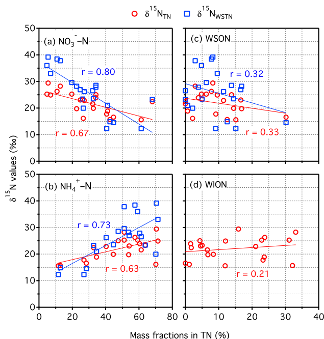
Figure 6. Scatterplots between \delta^{15}\text{N}_{\text{TN}} (and \delta^{15}\text{N}_{\text{WSTN}} ) and mass fractions of nitrogenous components ( \text{NO}_3^- -N, \text{NH}_4^+ -N, WSON and WION) in TN in Sapporo aerosols.
