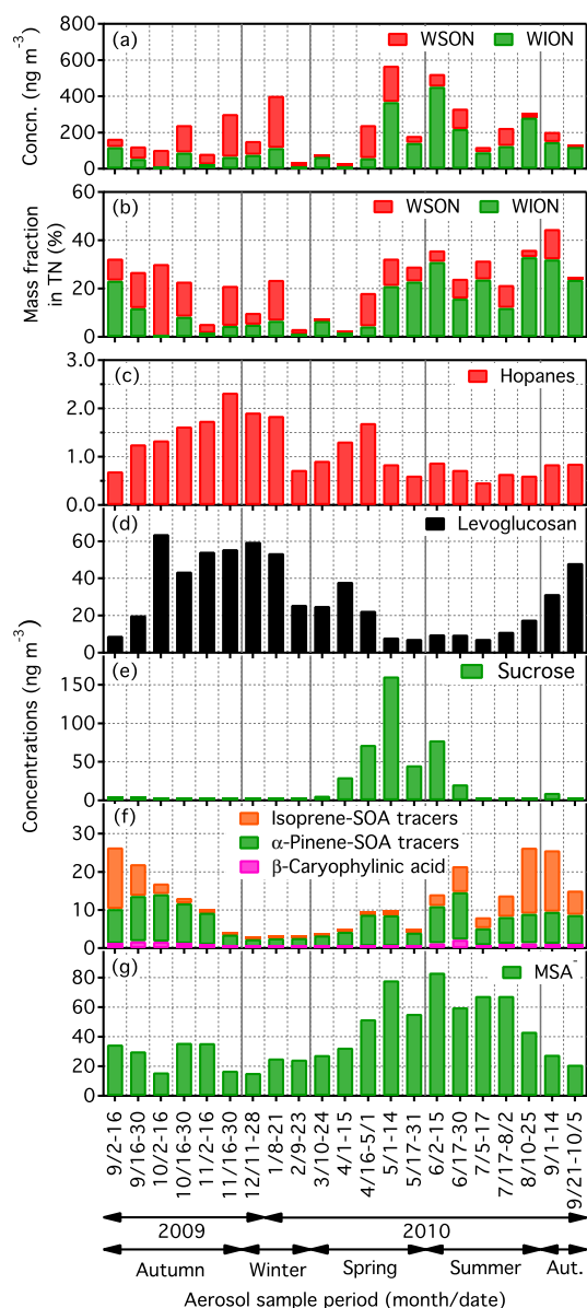
Figure 4. Seasonal variations in (a) concentrations of WSON and WION, (b) mass fractions of WSON and WION in TN, and (c)–(e) concentrations of organic molecular tracers and MSA − in Sapporo aerosols. Concentrations of hopanes are the sum of the concentrations of C 27 –C 32 hopanoid hydrocarbons. Concentrations of isoprene-SOA tracers are the sum of the concentrations of 2-methylglyceric acid, cis-2-methyl-1,3,4-trihydroxy-1-butene, 3-methyl-2,3,4-trihydroxy-1-butene, trans-2-methyl-1,3,4-trihydroxy-1-butene, 2-methylthreitol and 2-methylerythritol, whereas concentrations of \alpha -pinene-SOA tracers are the sum of the concentrations of 3-hydroxyglutaric, pinonic, pinic and 3-methyl-1,2,3-butanetricarboxylic acids. The data of organic molecular tracers are from Pavuluri et al. (2013) and MSA − is from Pavuluri et al. (2015).
