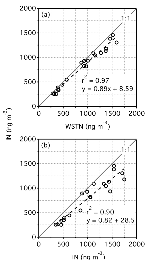
Figure 3. Linear relations of IN (sum of \text{NO}_3^- \text{-N} and \text{NH}_4^+ \text{-N} ) to (a) WSTN and (b) TN.
